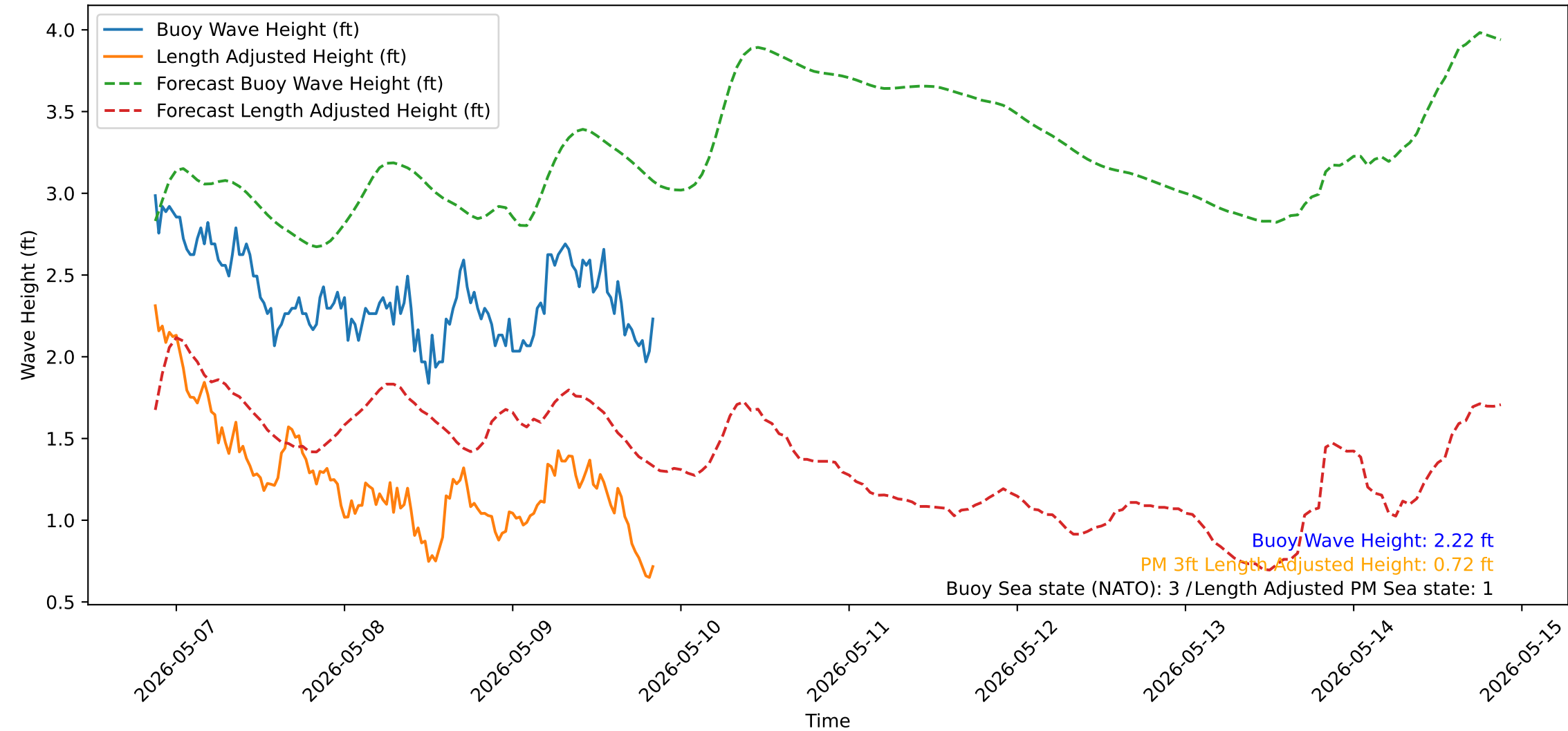
Wave Heights over Time for Green Beach at 2026-05-09 20:51:21
