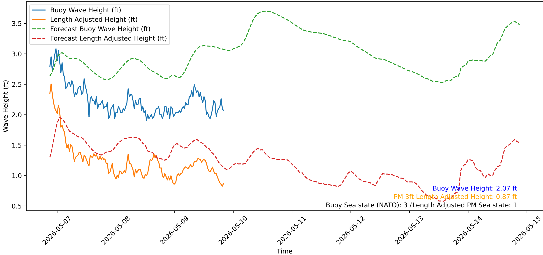
Wave Heights over Time for Red Beach at 2026-05-09 20:50:56
