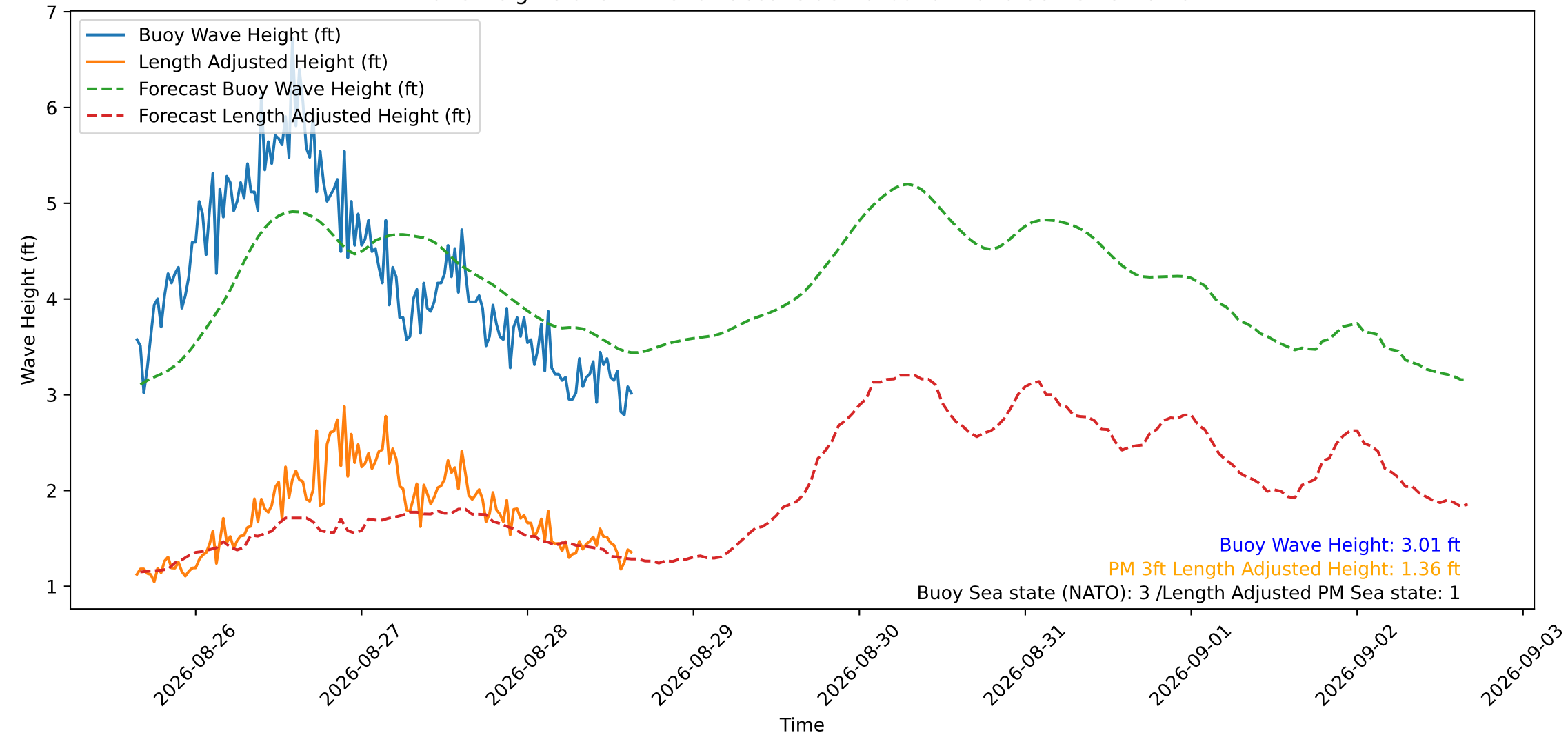
Wave Heights over Time for Oceanside Harbor at 2026-08-28 15:40:29
