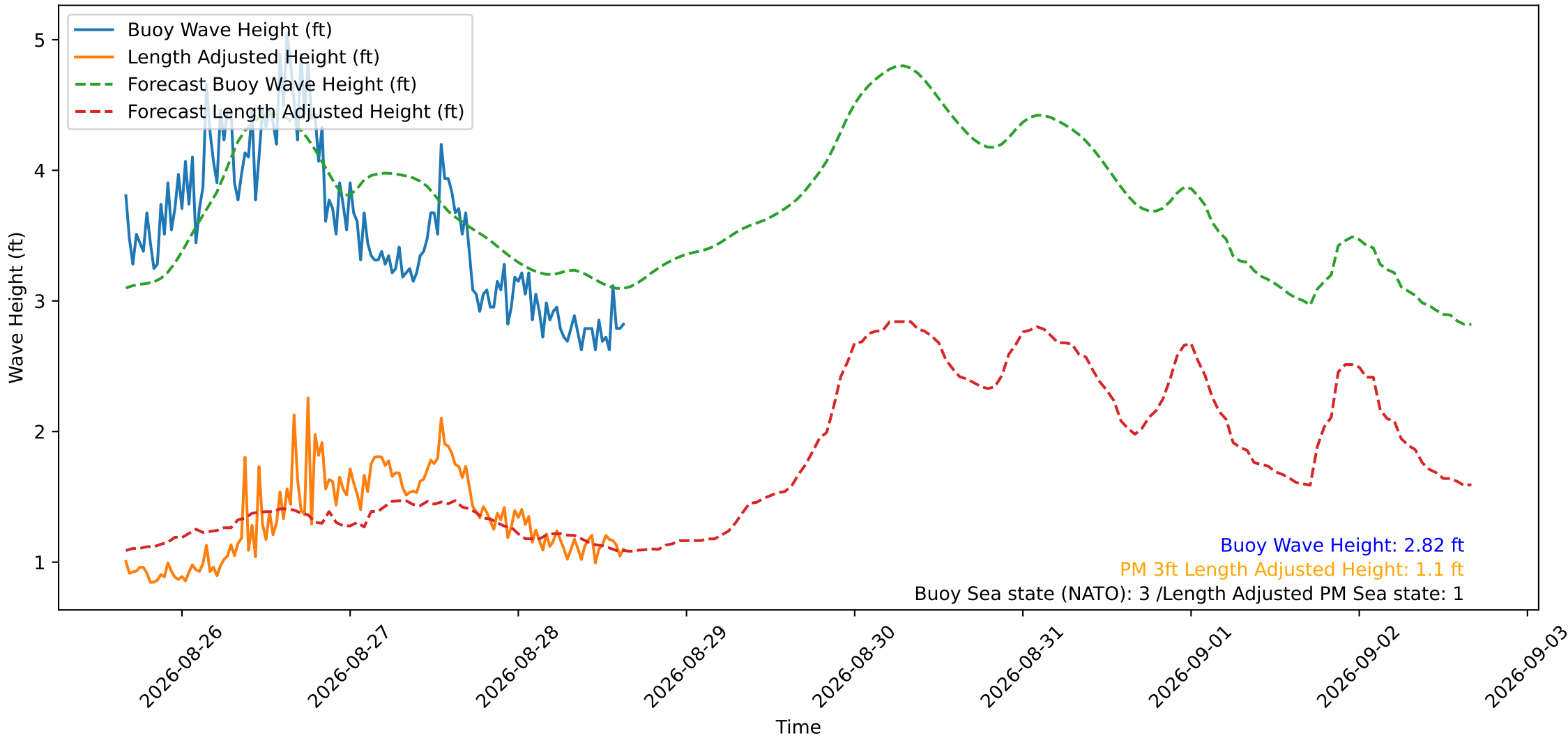
Wave Heights over Time for Red Beach at 2026-08-28 15:40:49
