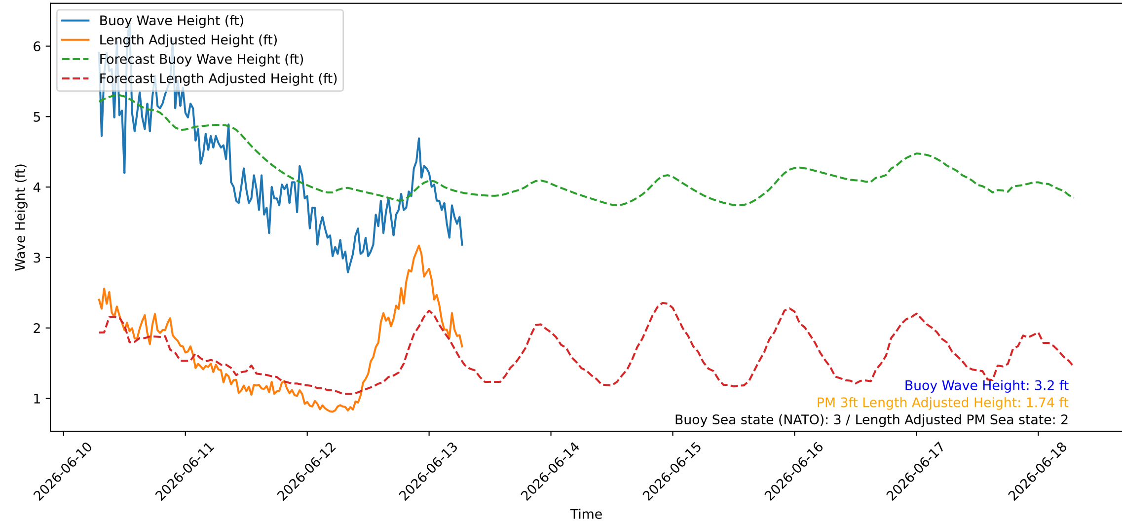
Wave Heights over Time for Oceanside Harbor at 2026-06-13 07:10:26
