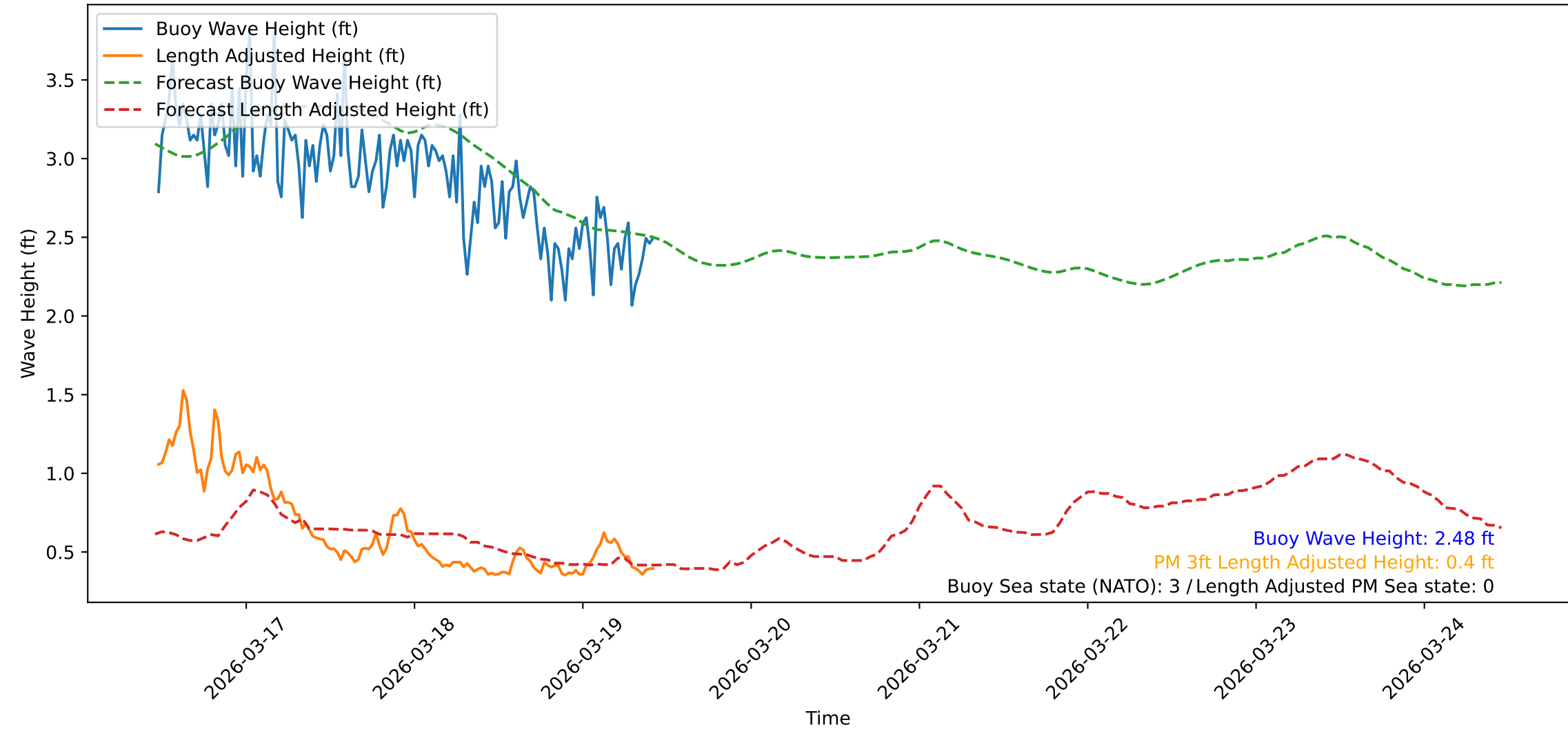
Wave Heights over Time for Red Beach at 2026-03-19 11:00:47
