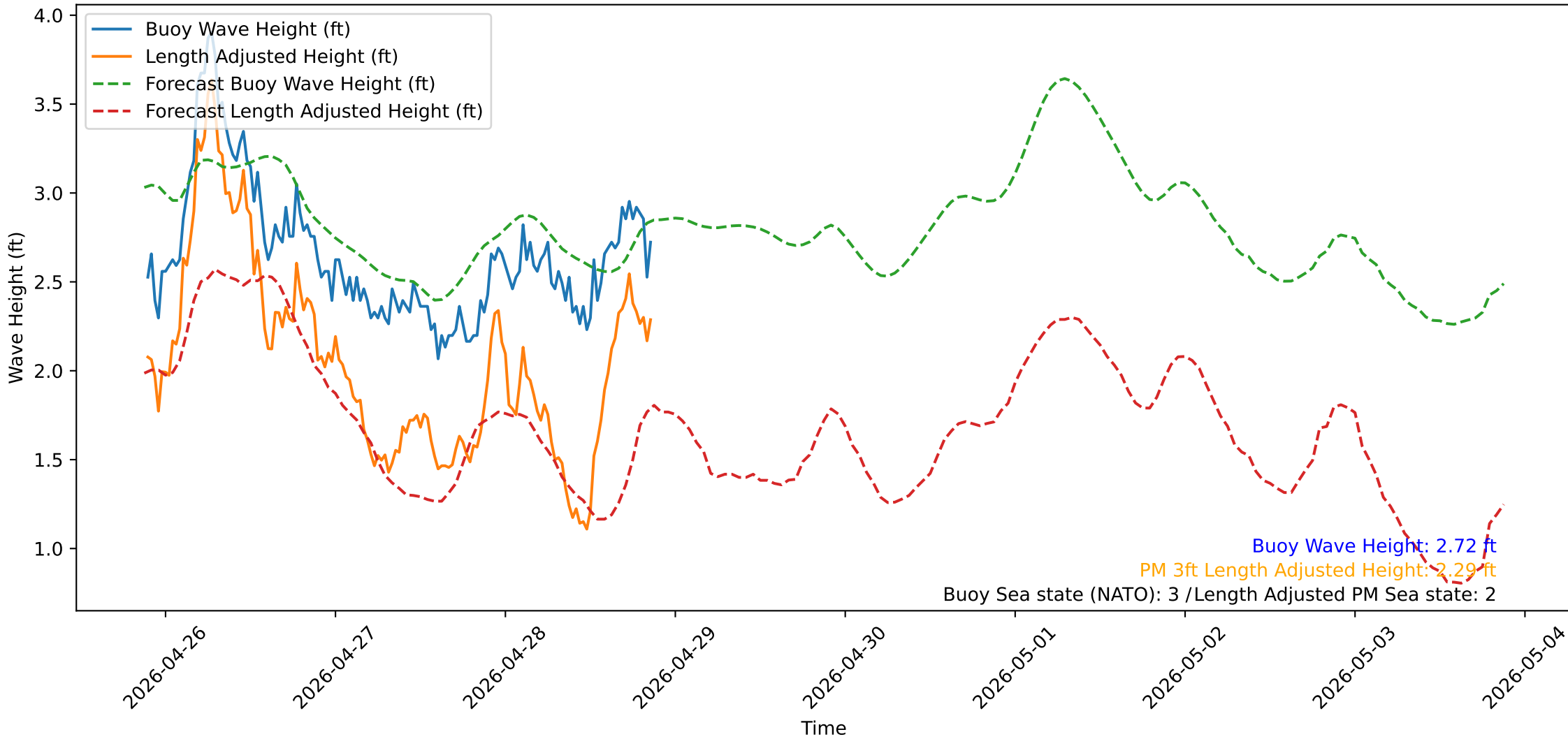
Wave Heights over Time for Oceanside Harbor at 2026-04-28 21:20:32
