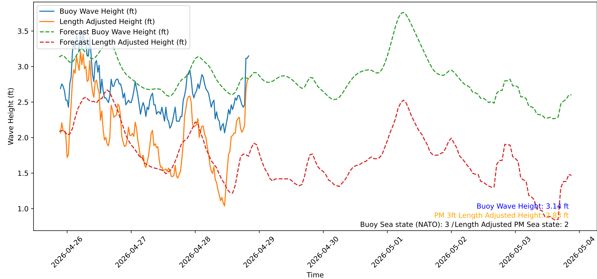
Wave Heights over Time for Green Beach at 2026-04-28 21:21:15
