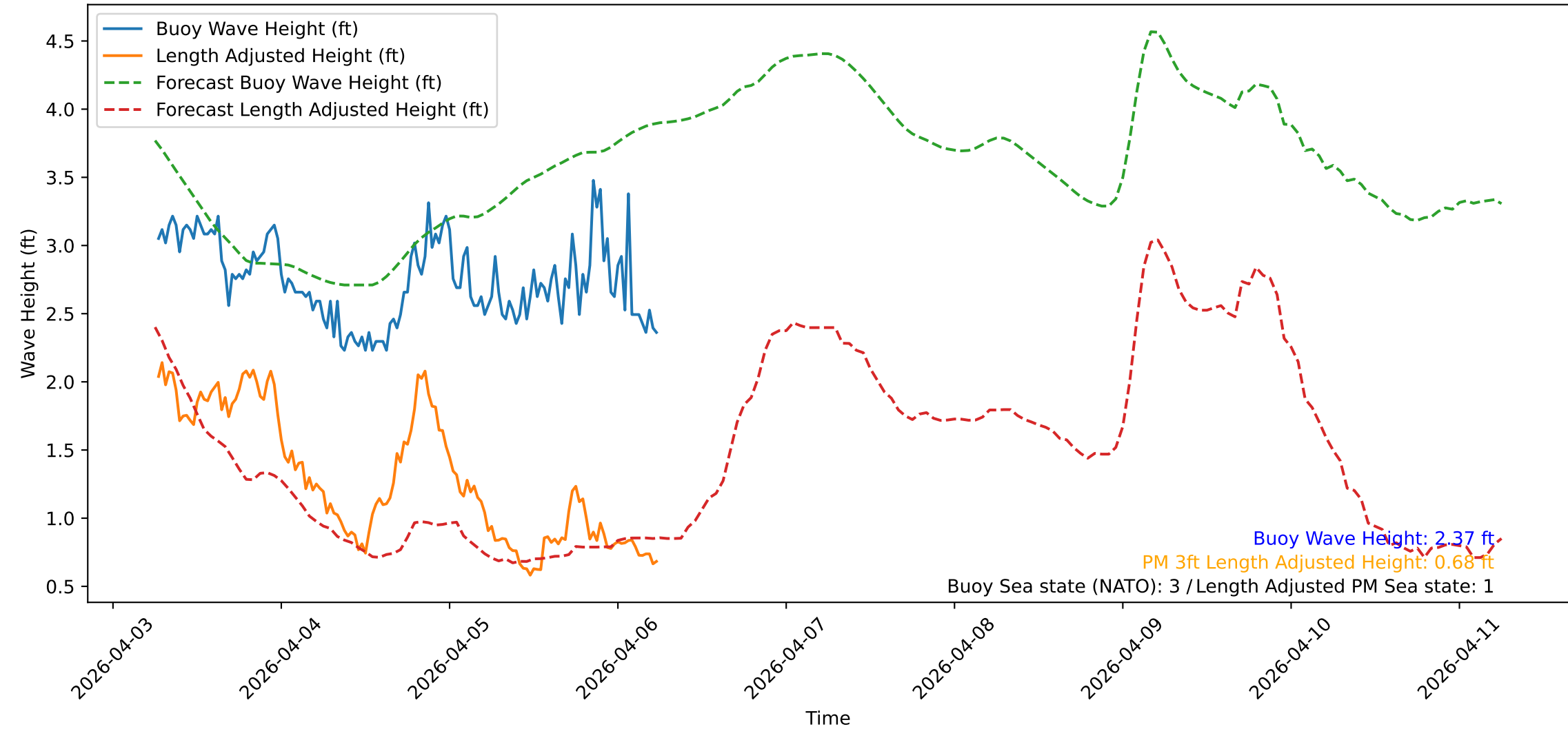
Wave Heights over Time for Green Beach at 2026-04-06 06:21:10
