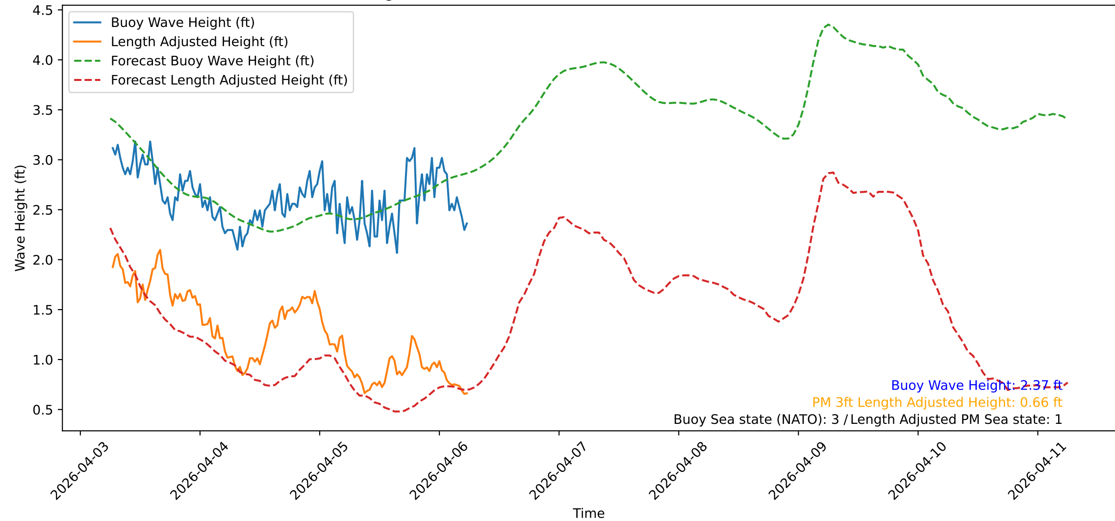
Wave Heights over Time for Oceanside Harbor at 2026-04-06 06:20:31
