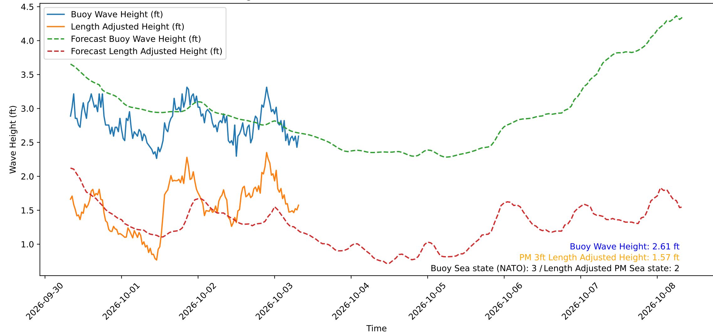
Wave Heights over Time for Oceanside Harbor at 2026-10-03 08:10:29
