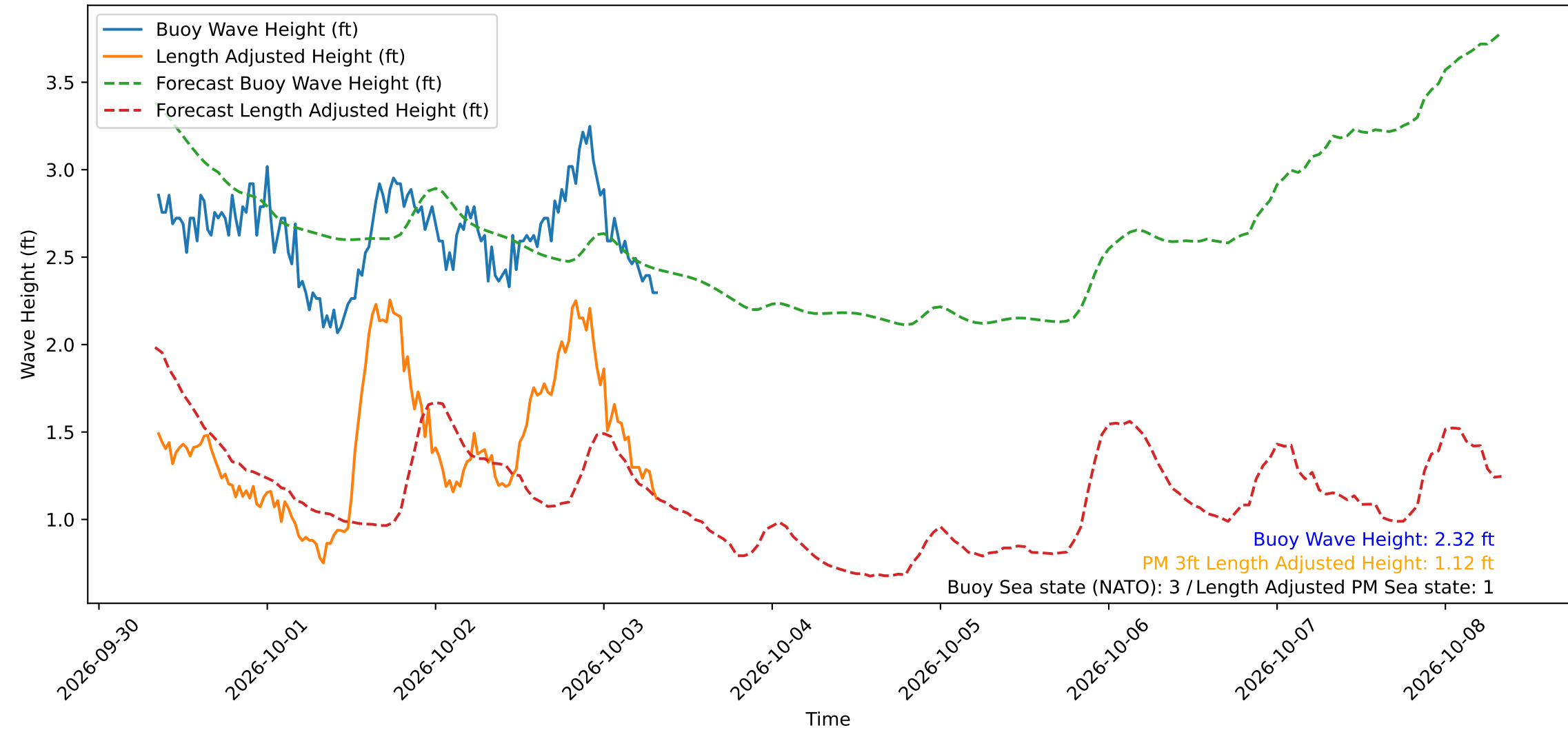
Wave Heights over Time for Red Beach at 2026-10-03 08:10:49
