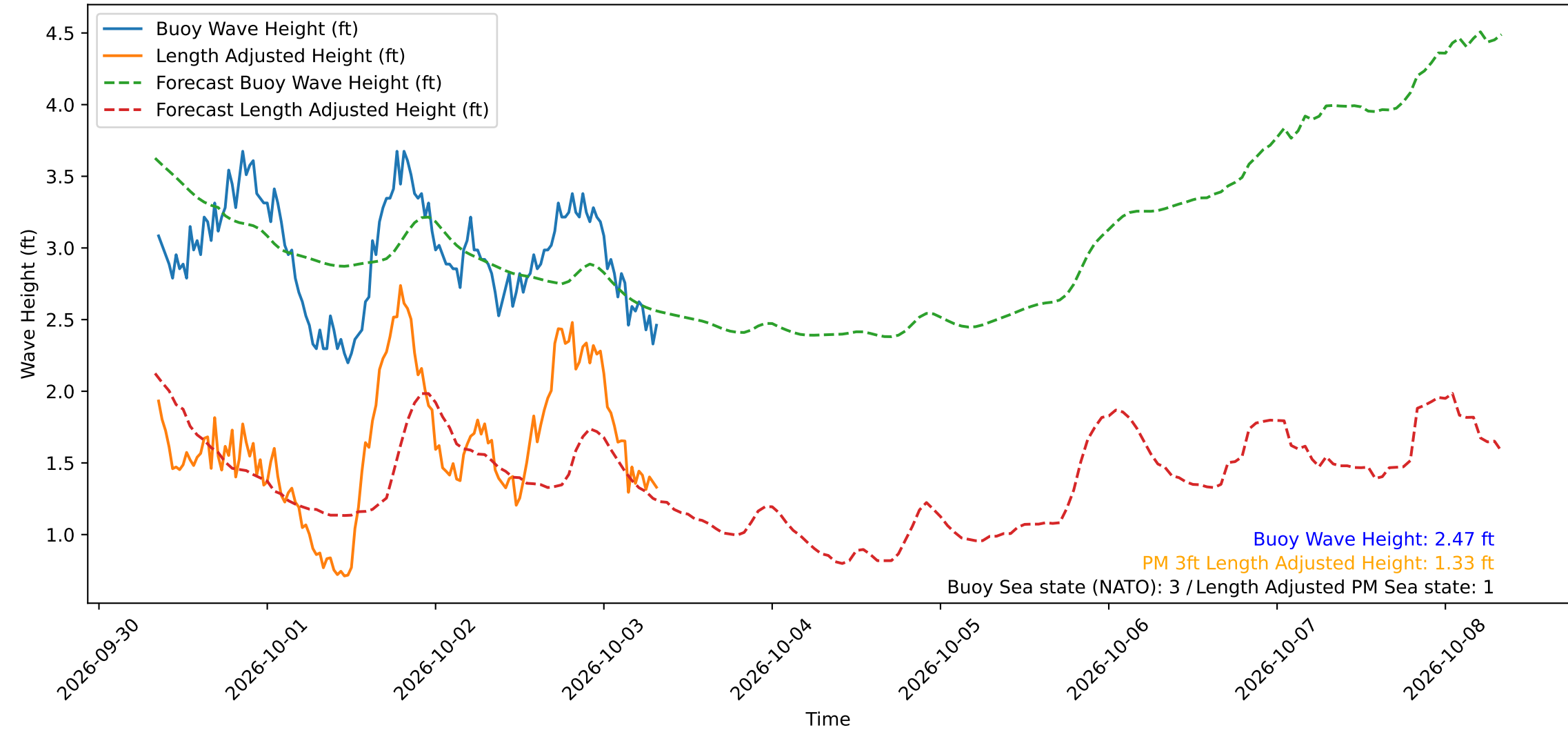
Wave Heights over Time for Green Beach at 2026-10-03 08:11:11
