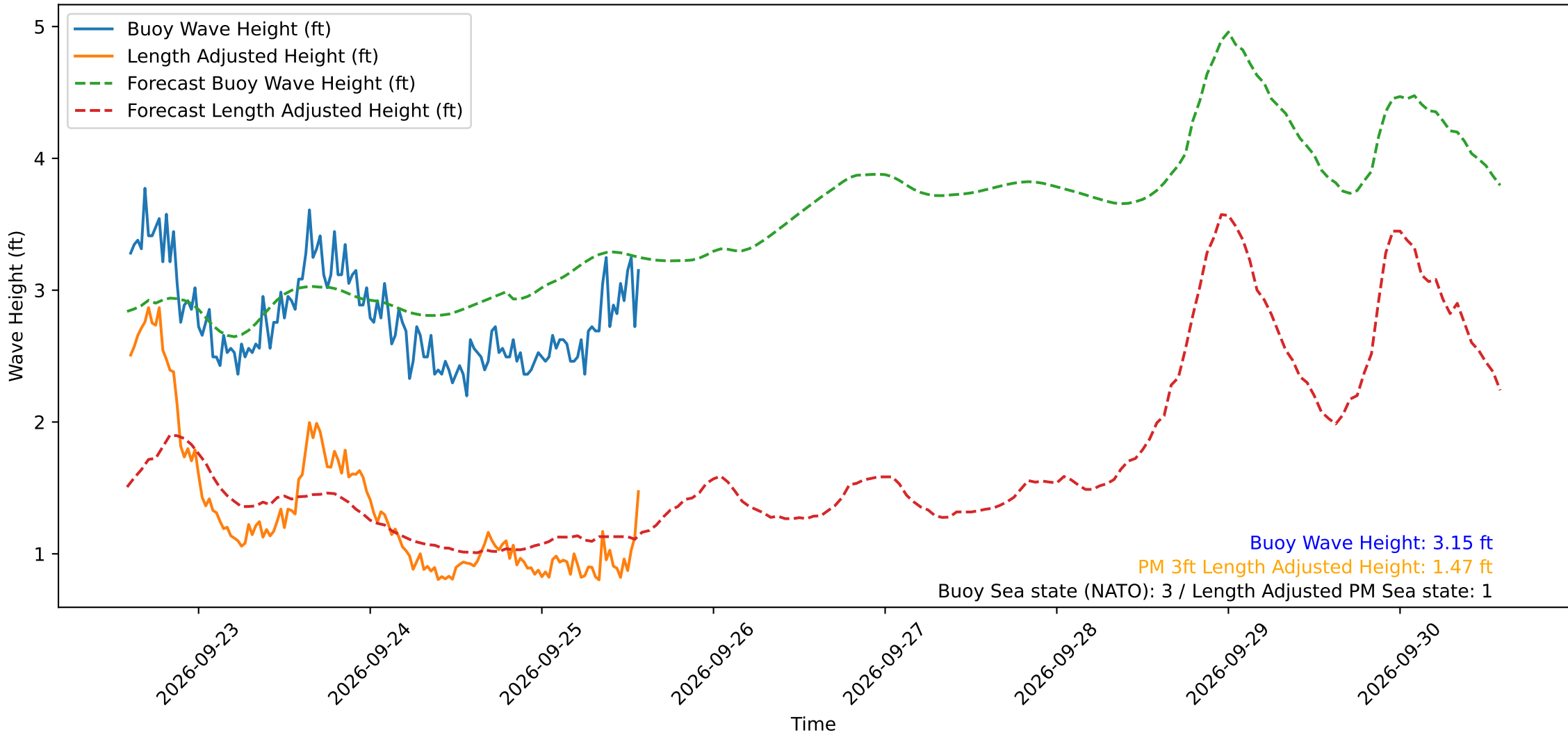
Wave Heights over Time for Oceanside Harbor at 2026-09-25 14:20:30
