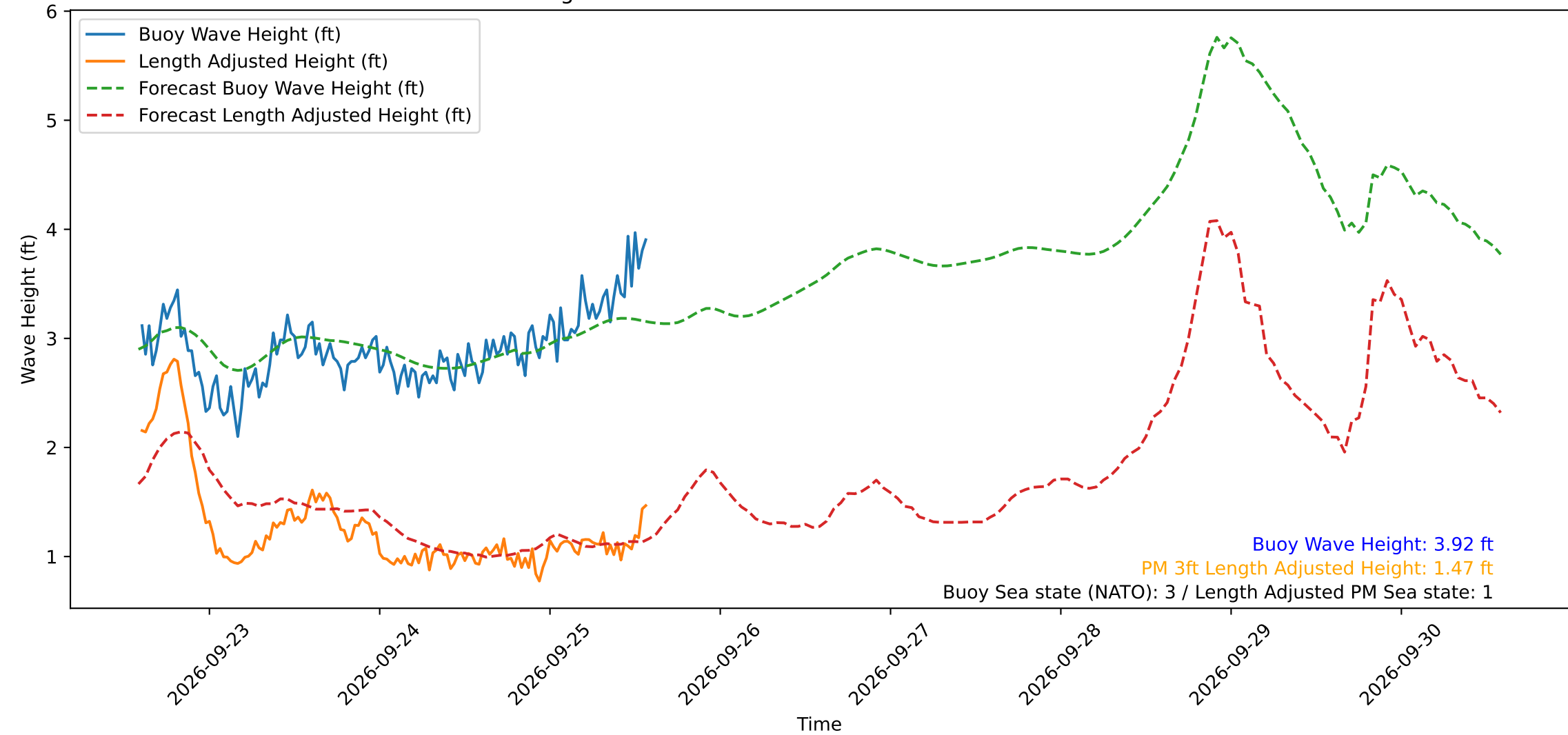
Wave Heights over Time for Green Beach at 2026-09-25 14:21:15
