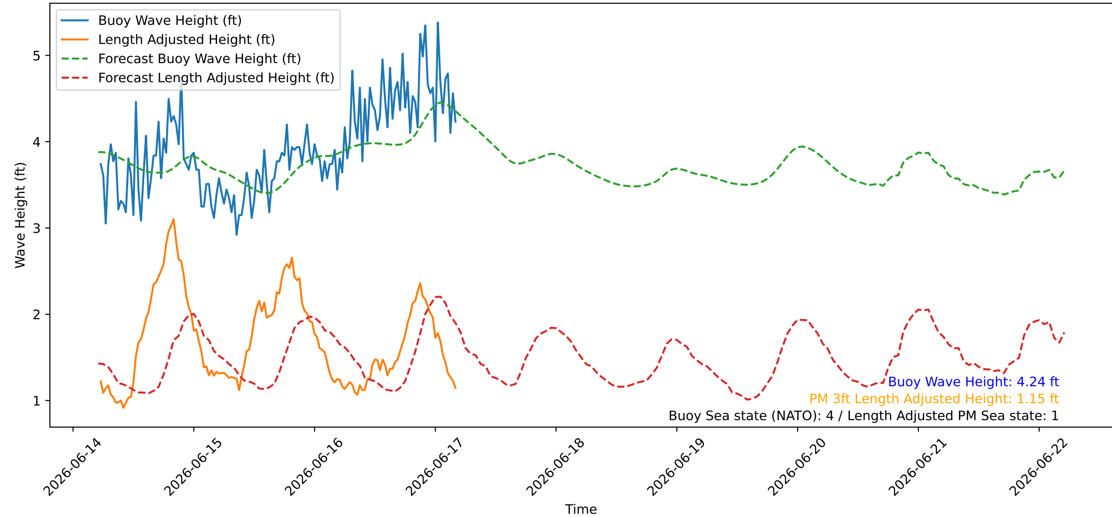
Wave Heights over Time for Red Beach at 2026-06-17 05:00:44
