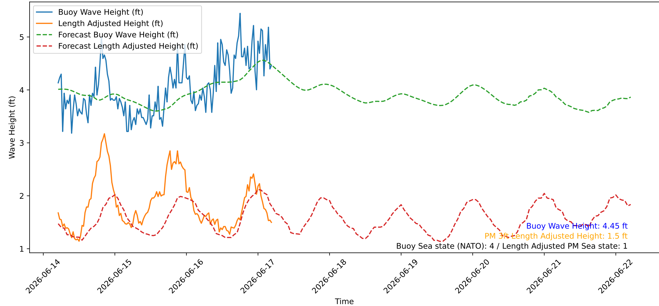
Wave Heights over Time for Oceanside Harbor at 2026-06-17 05:00:26
