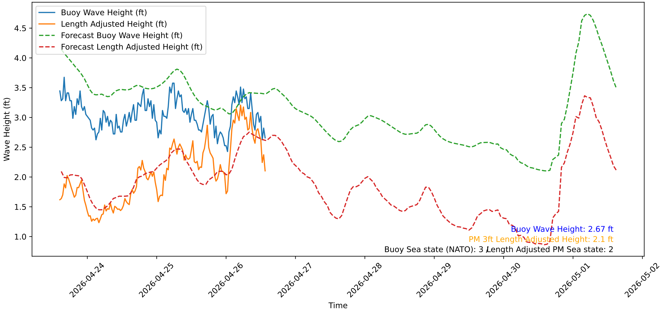
Wave Heights over Time for Green Beach at 2026-04-26 14:31:13
