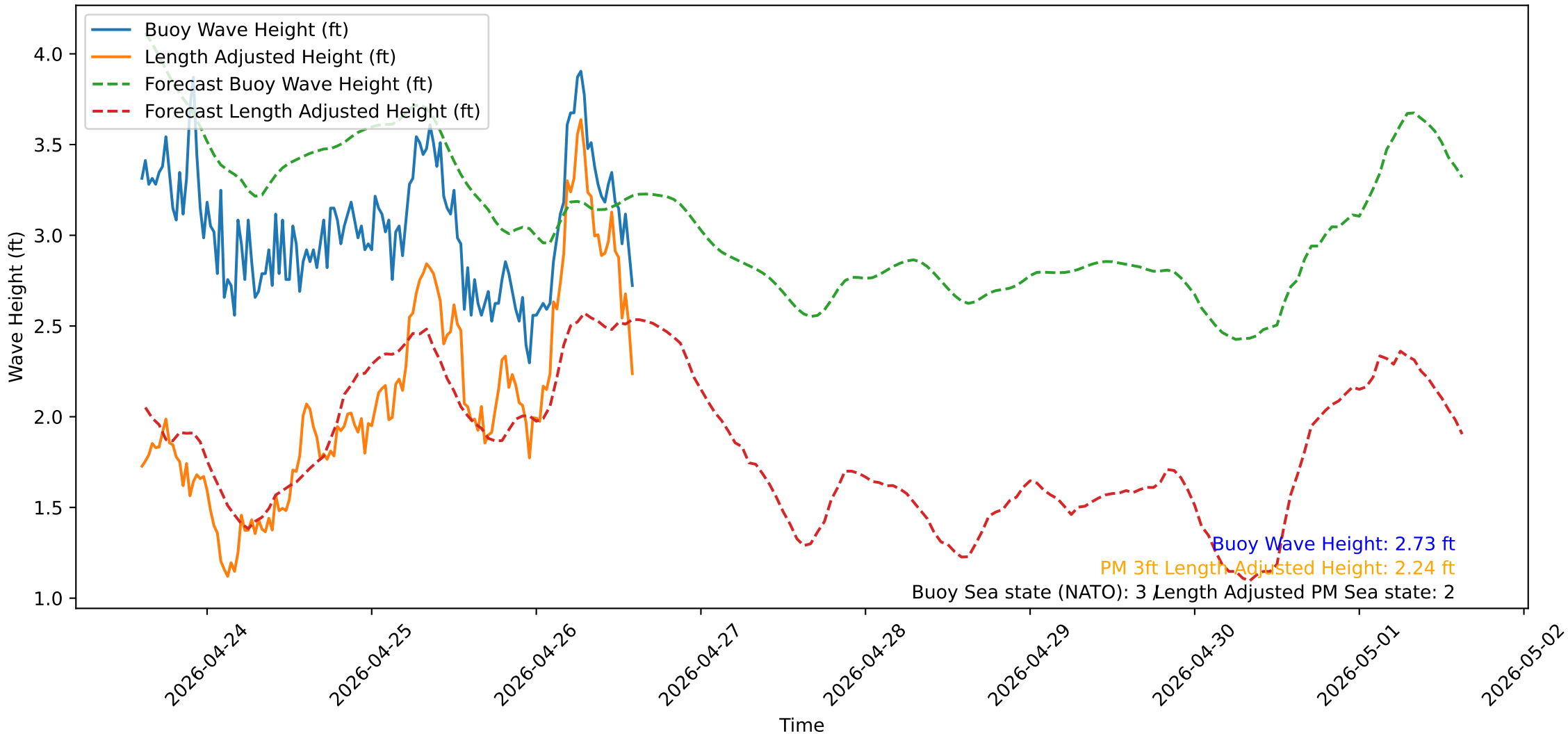
Wave Heights over Time for Oceanside Harbor at 2026-04-26 14:30:31
