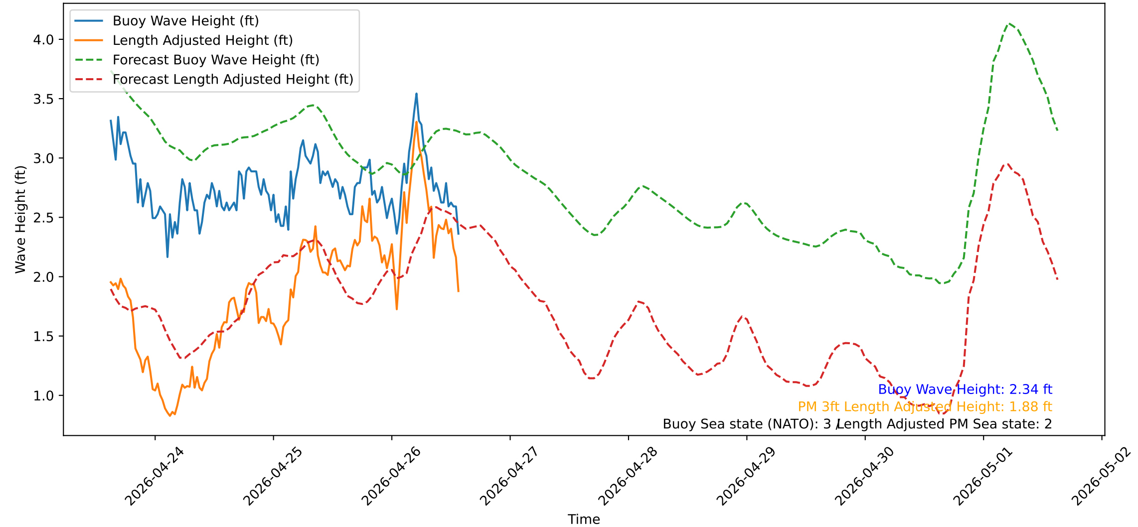
Wave Heights over Time for Red Beach at 2026-04-26 14:30:50
