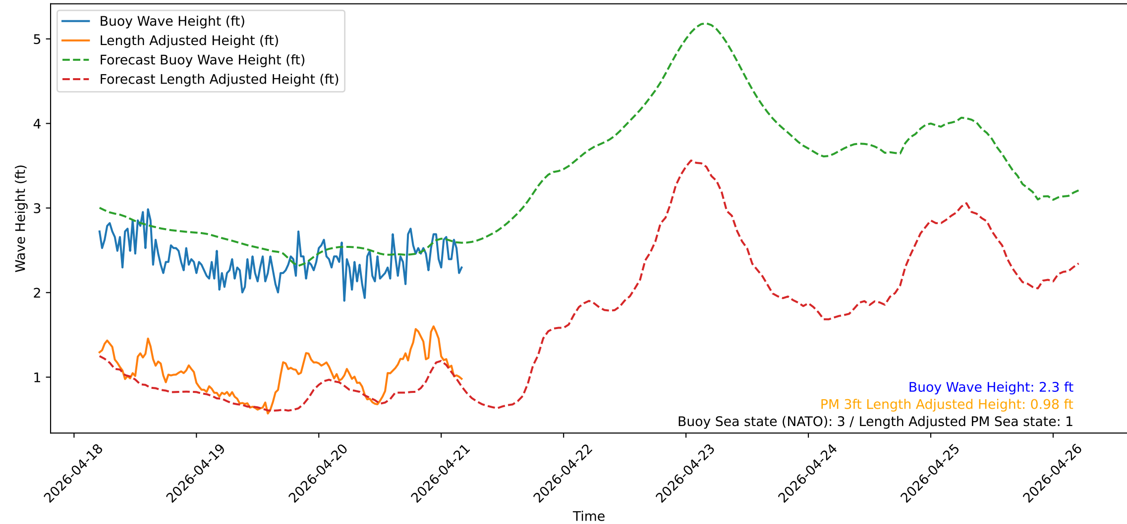
Wave Heights over Time for Oceanside Harbor at 2026-04-21 04:50:31
