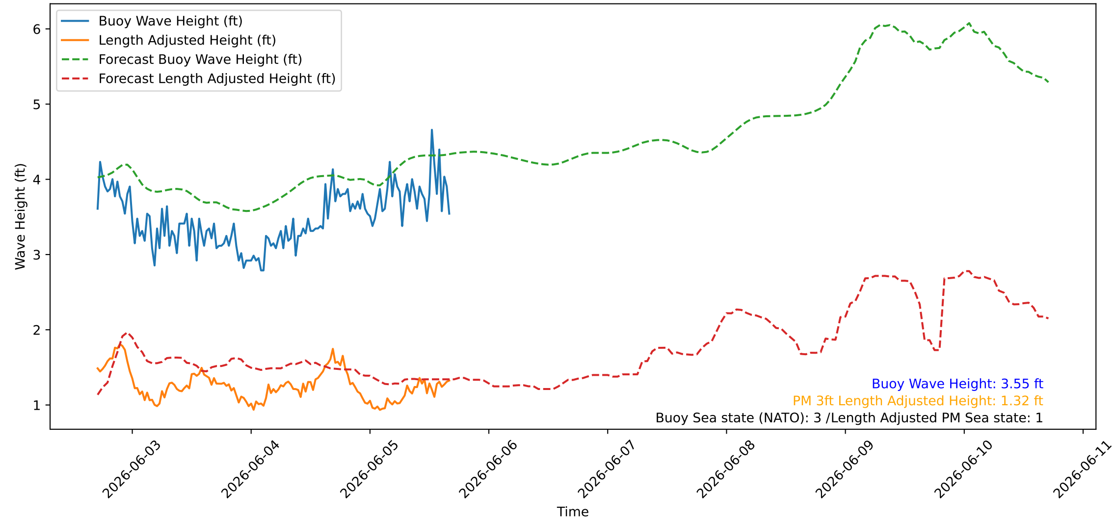
Wave Heights over Time for Green Beach at 2026-06-05 16:51:08
