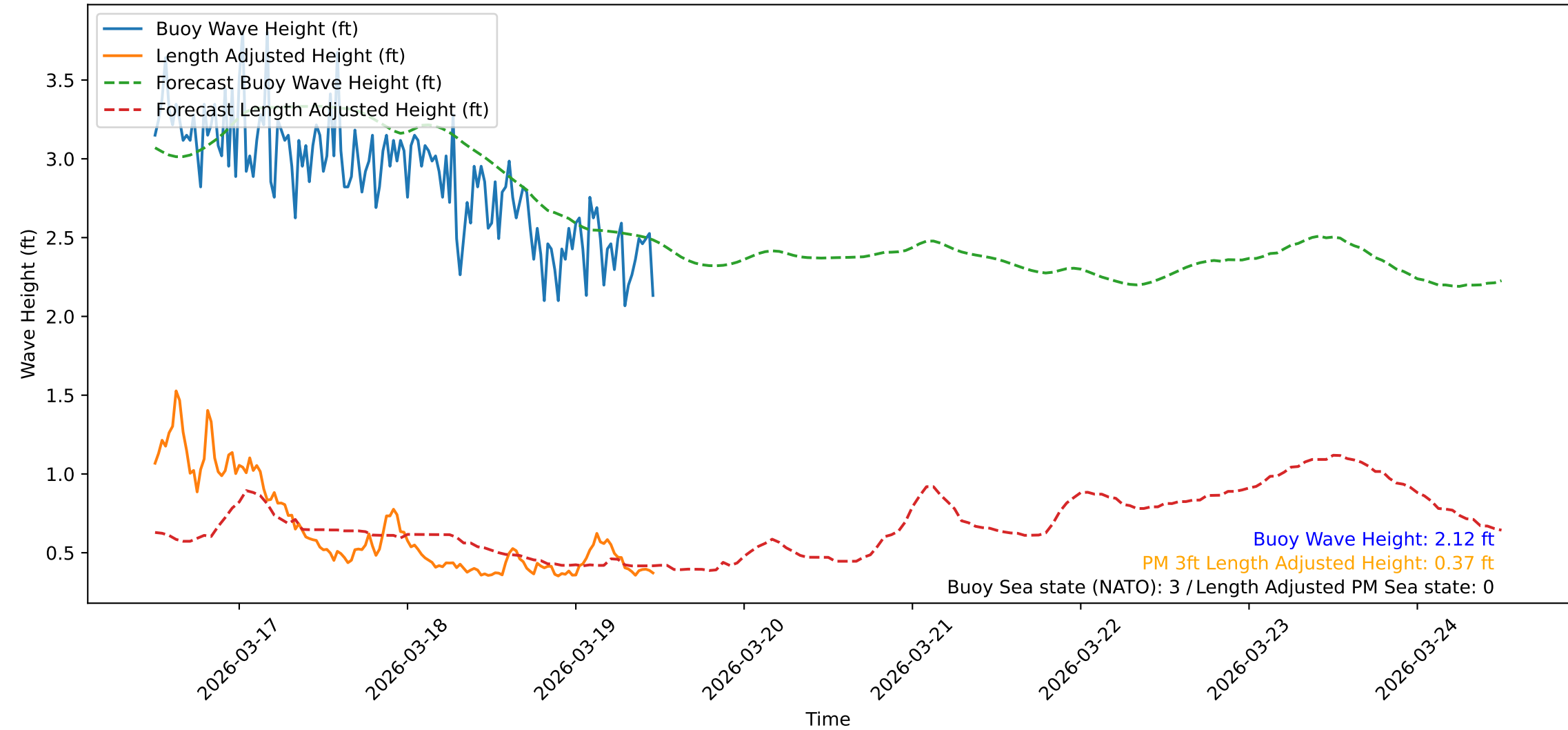
Wave Heights over Time for Red Beach at 2026-03-19 11:50:47
