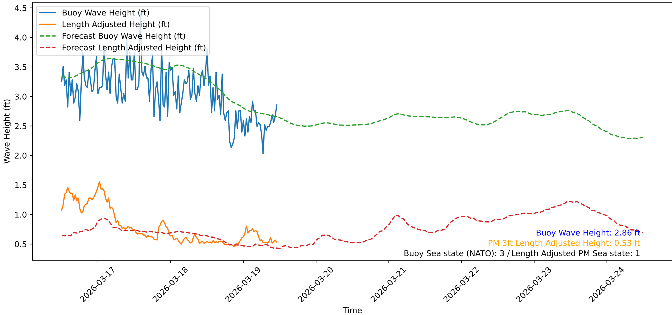
Wave Heights over Time for Oceanside Harbor at 2026-03-19 11:50:31
