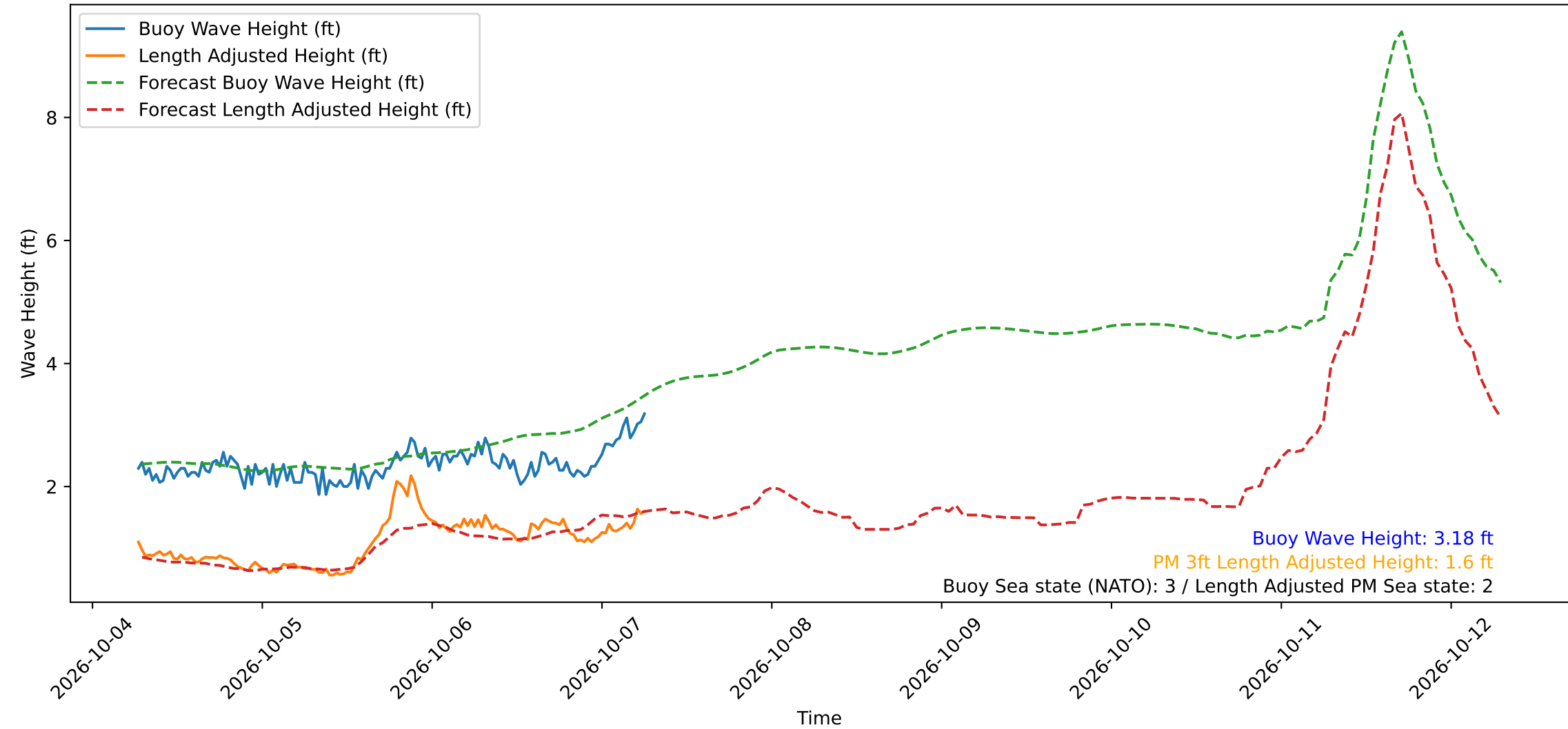
Wave Heights over Time for Oceanside Harbor at 2026-10-07 06:40:29
