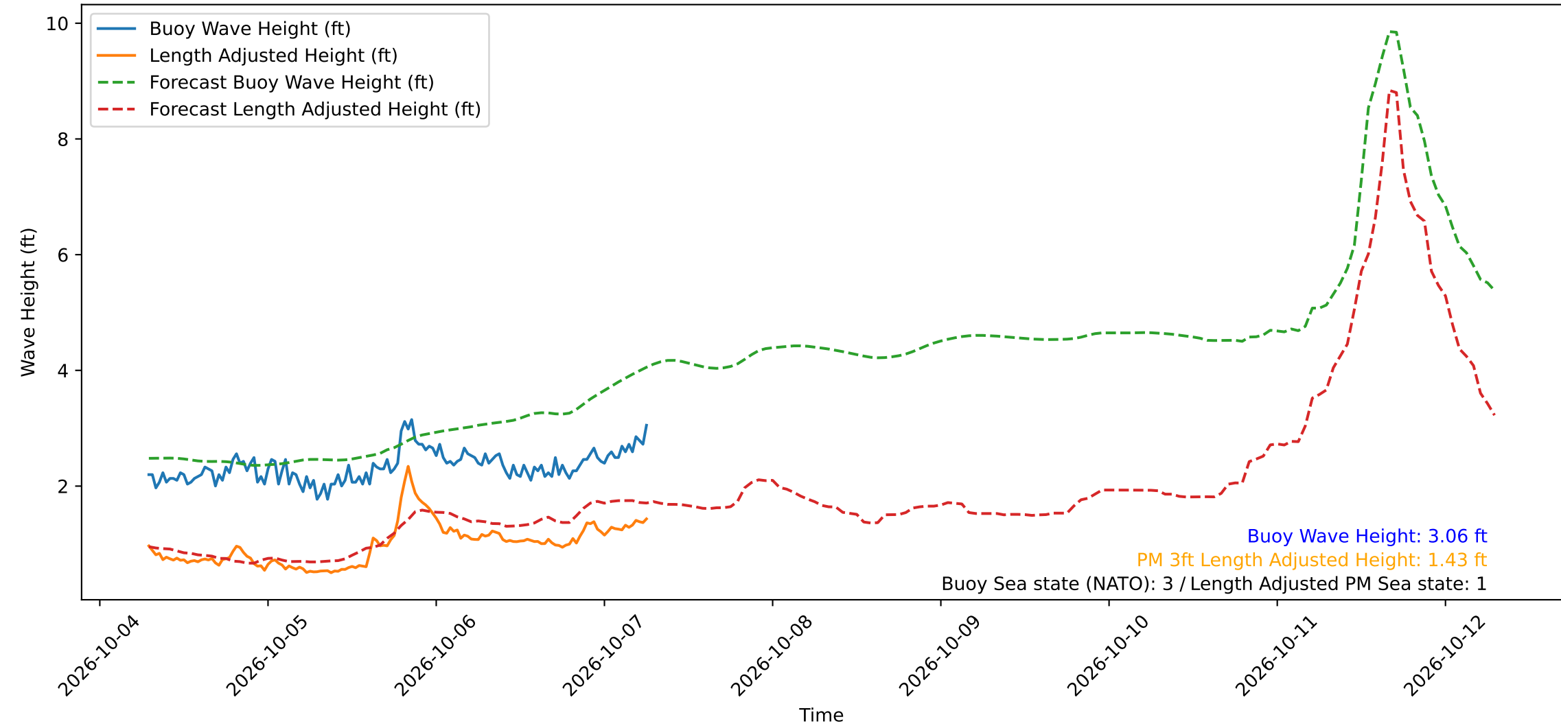
Wave Heights over Time for Green Beach at 2026-10-07 06:41:12
