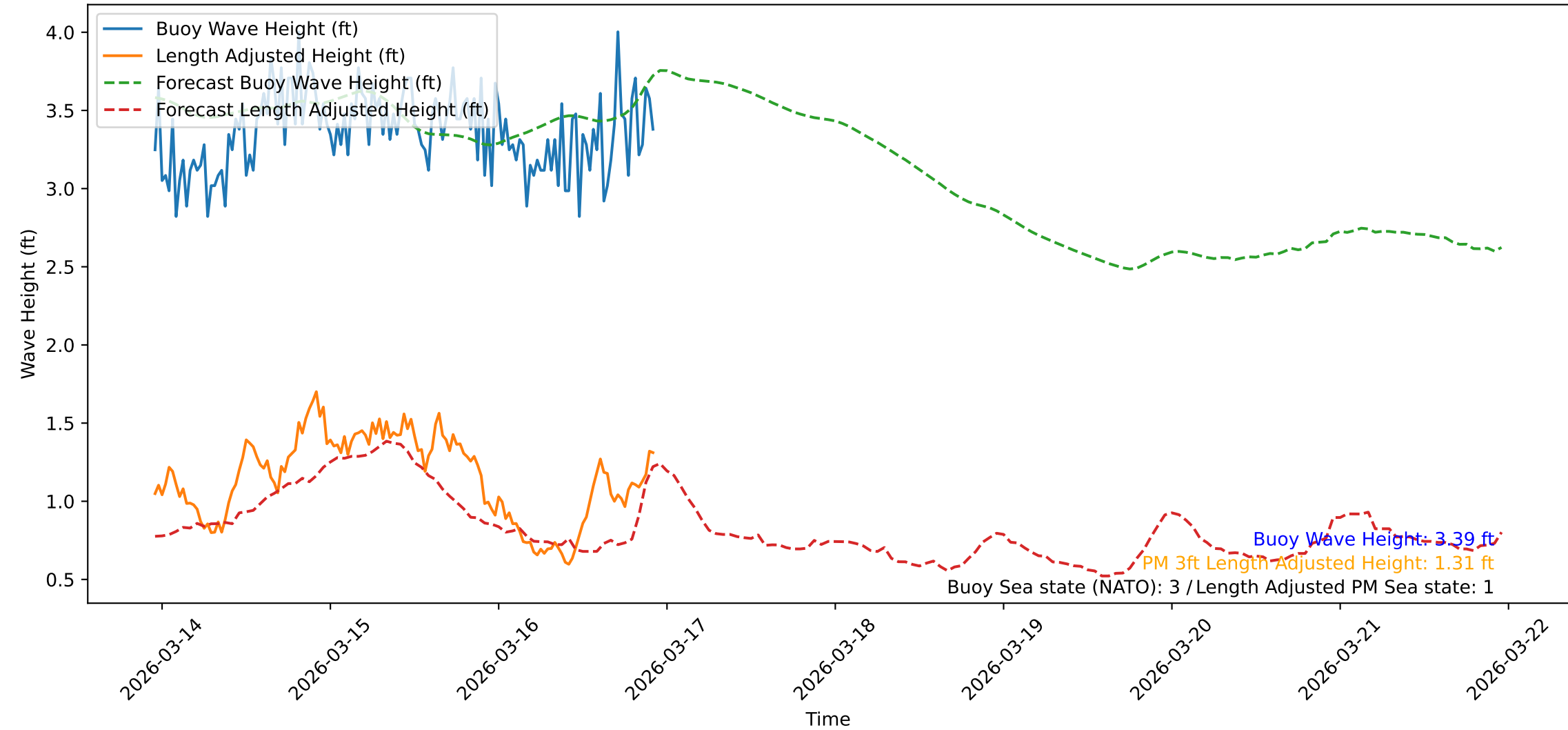
Wave Heights over Time for Green Beach at 2026-03-16 23:11:38
