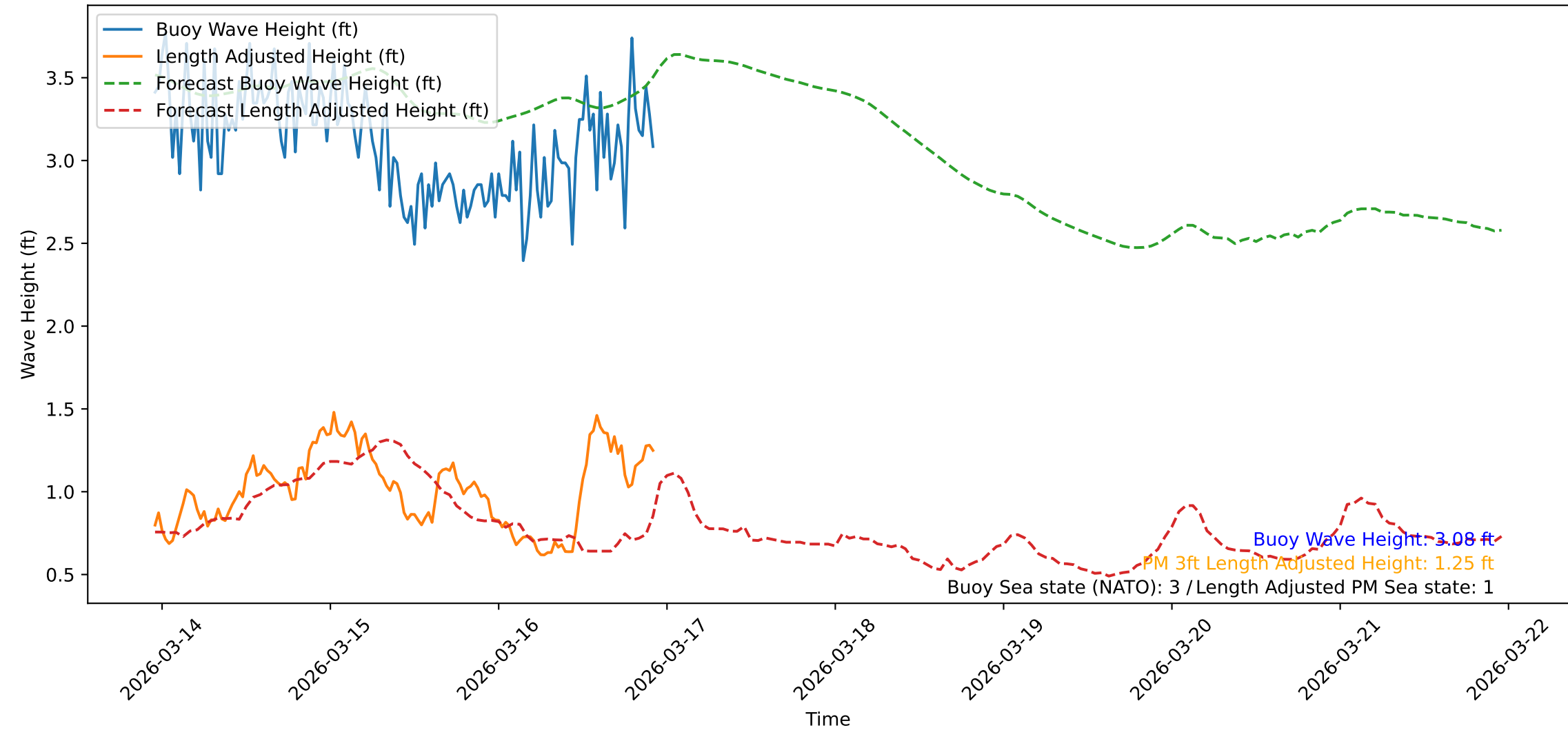
Wave Heights over Time for Oceanside Harbor at 2026-03-16 23:10:42
