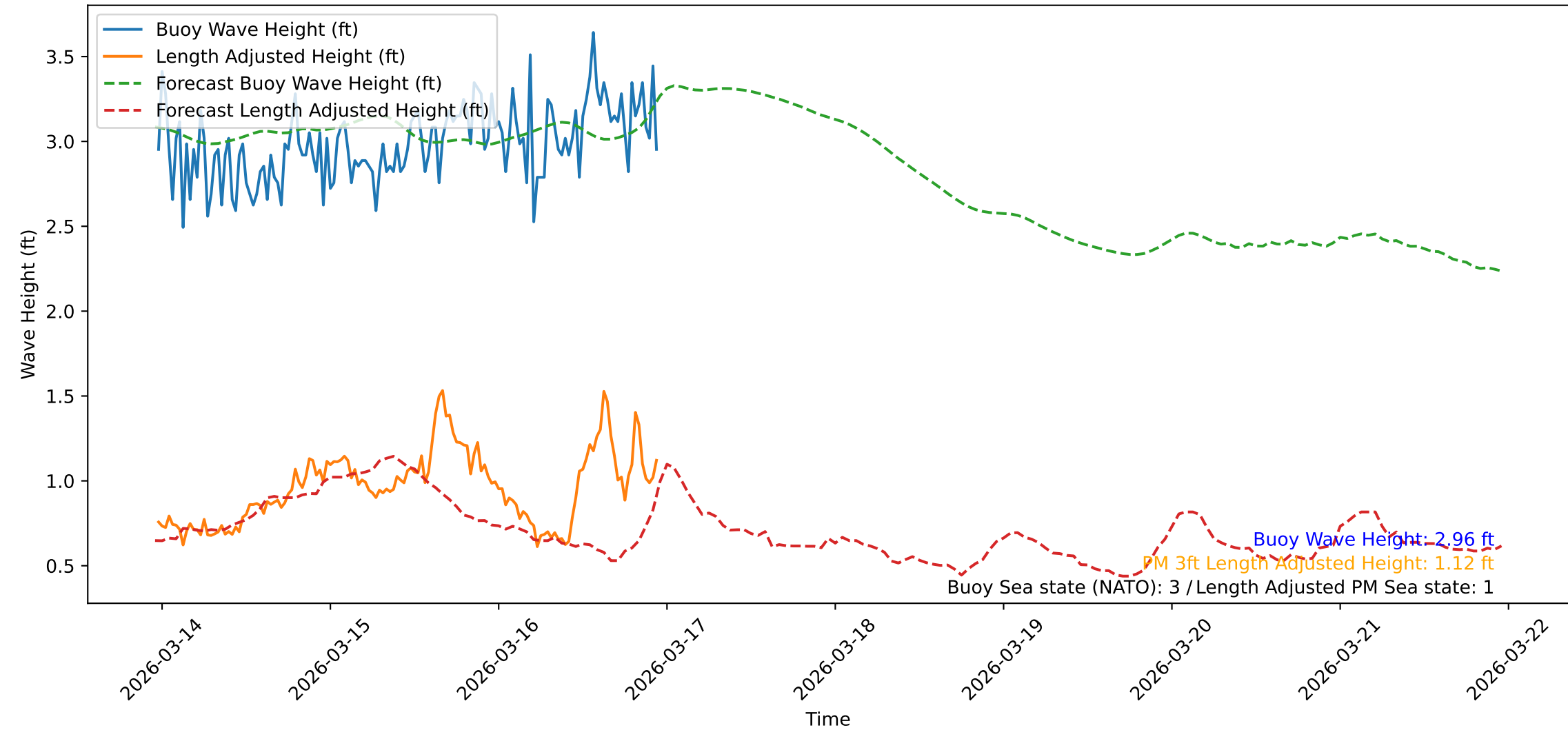
Wave Heights over Time for Red Beach at 2026-03-16 23:11:04
