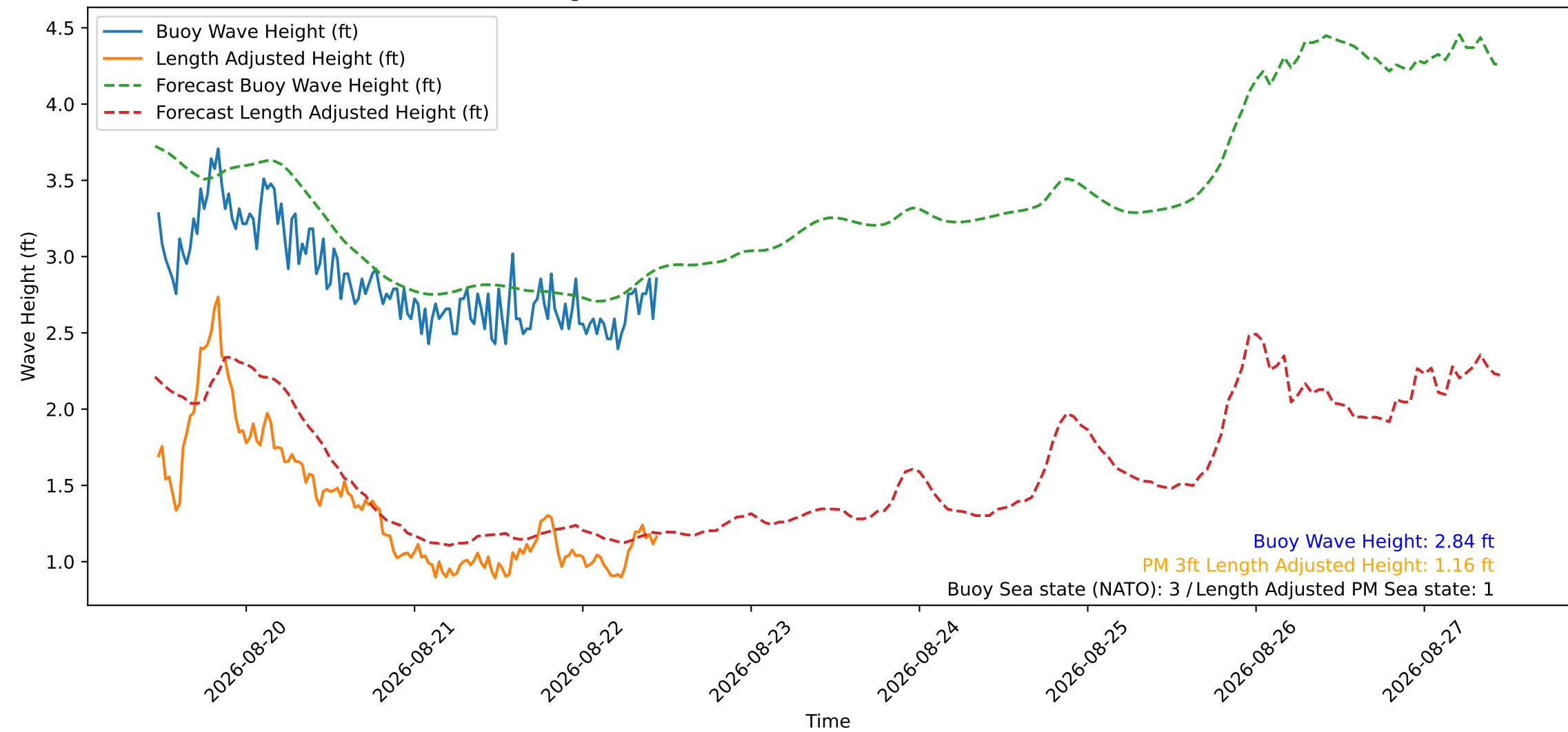
Wave Heights over Time for Green Beach at 2026-08-22 11:11:11
