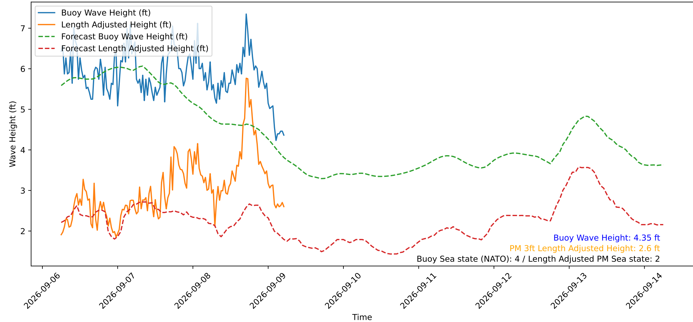
Wave Heights over Time for Oceanside Harbor at 2026-09-09 05:50:30
