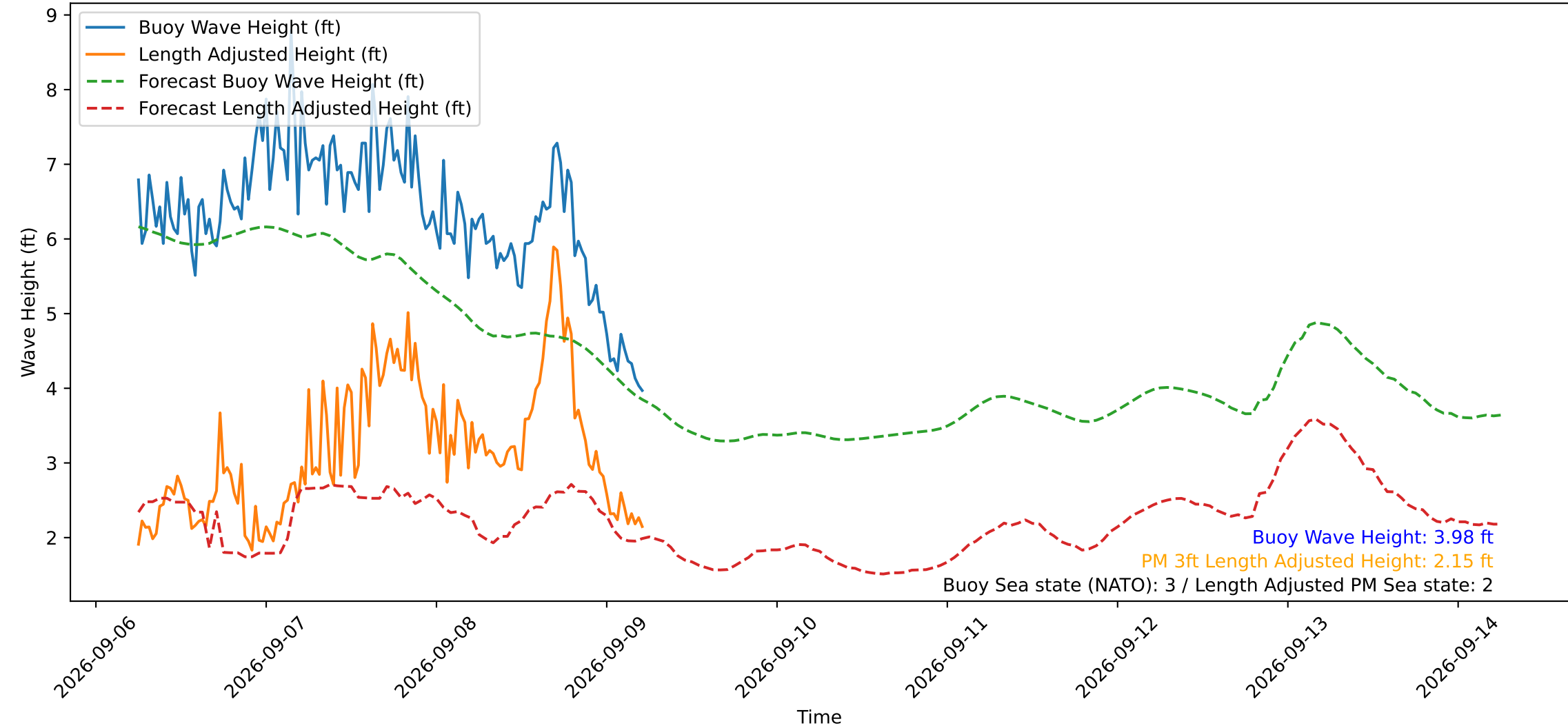
Wave Heights over Time for Green Beach at 2026-09-09 05:51:14
