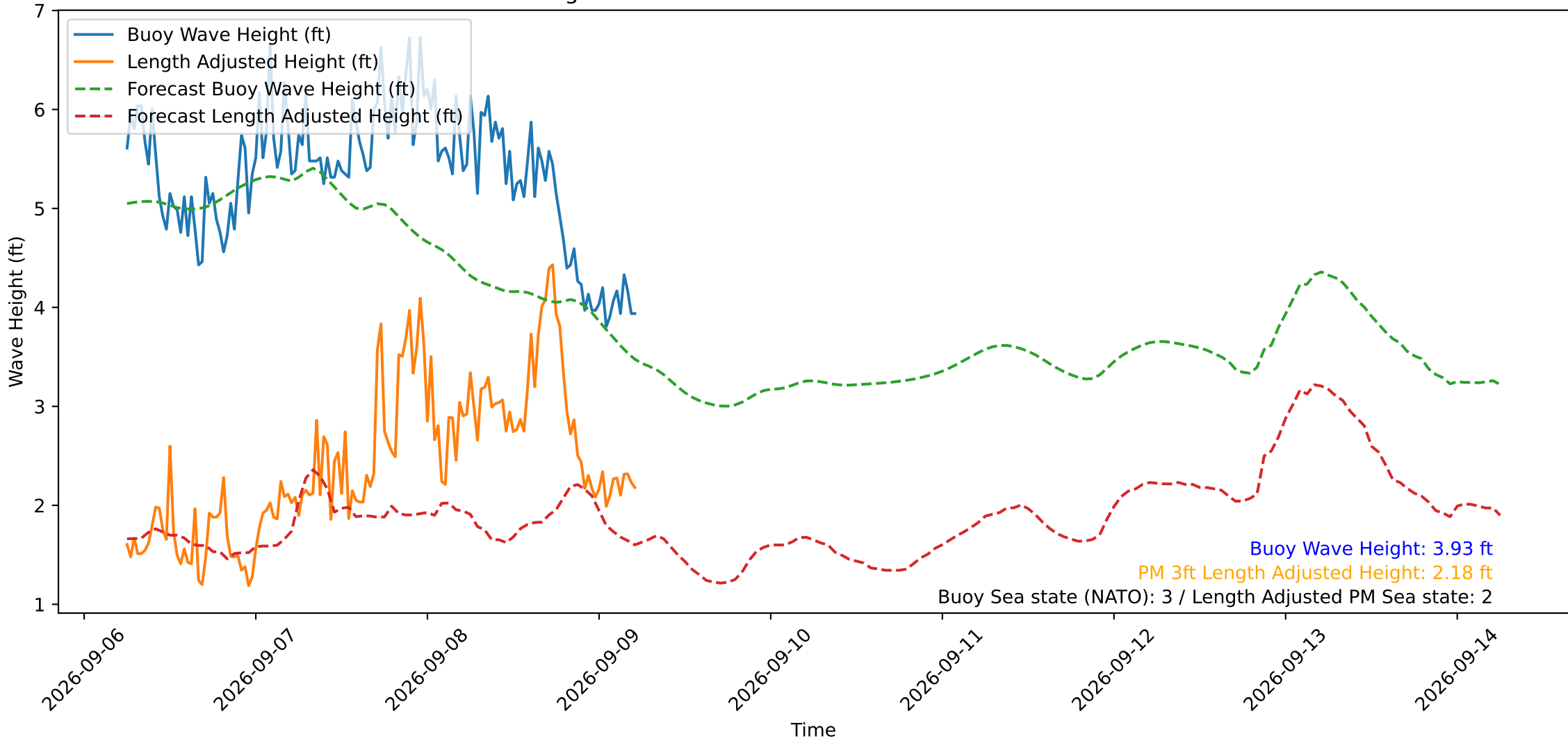
Wave Heights over Time for Red Beach at 2026-09-09 05:50:51
