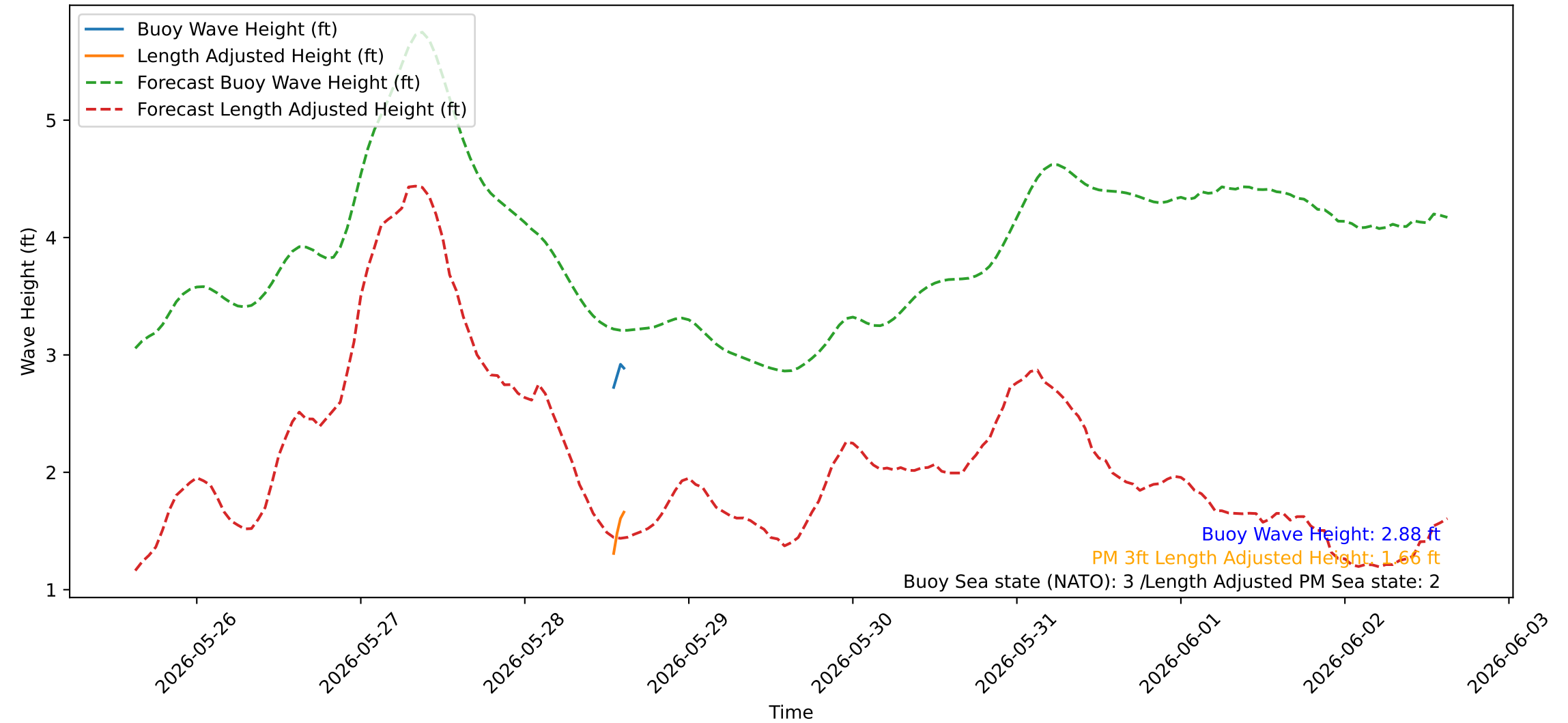
Wave Heights over Time for Oceanside Harbor at 2026-05-28 15:20:19
