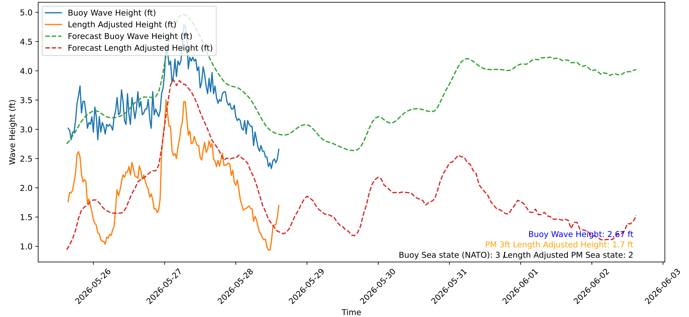
Wave Heights over Time for Red Beach at 2026-05-28 15:20:39
