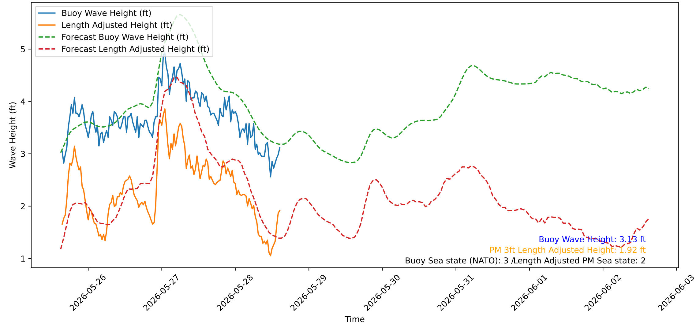
Wave Heights over Time for Green Beach at 2026-05-28 15:21:01
