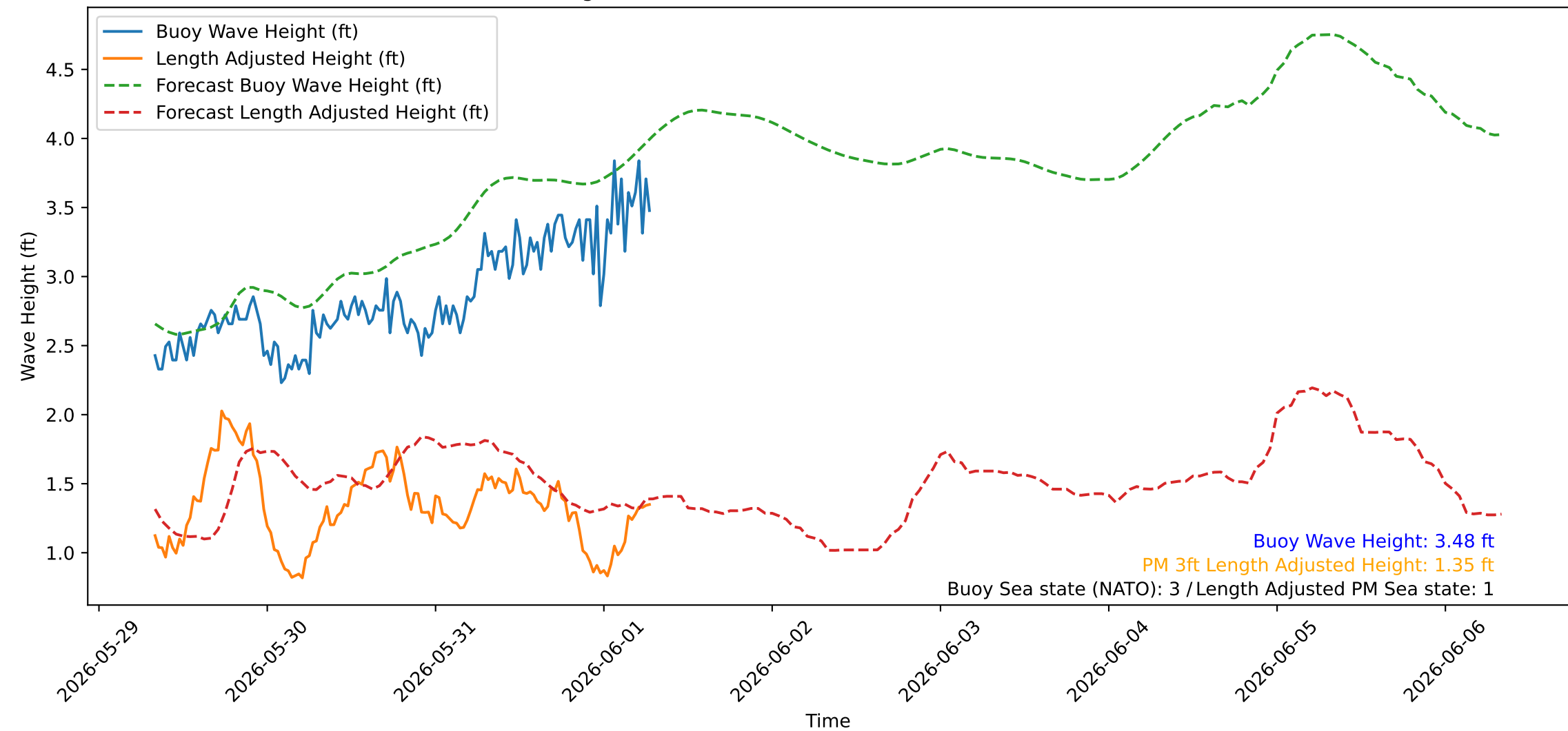
Wave Heights over Time for Red Beach at 2026-06-01 07:30:44
