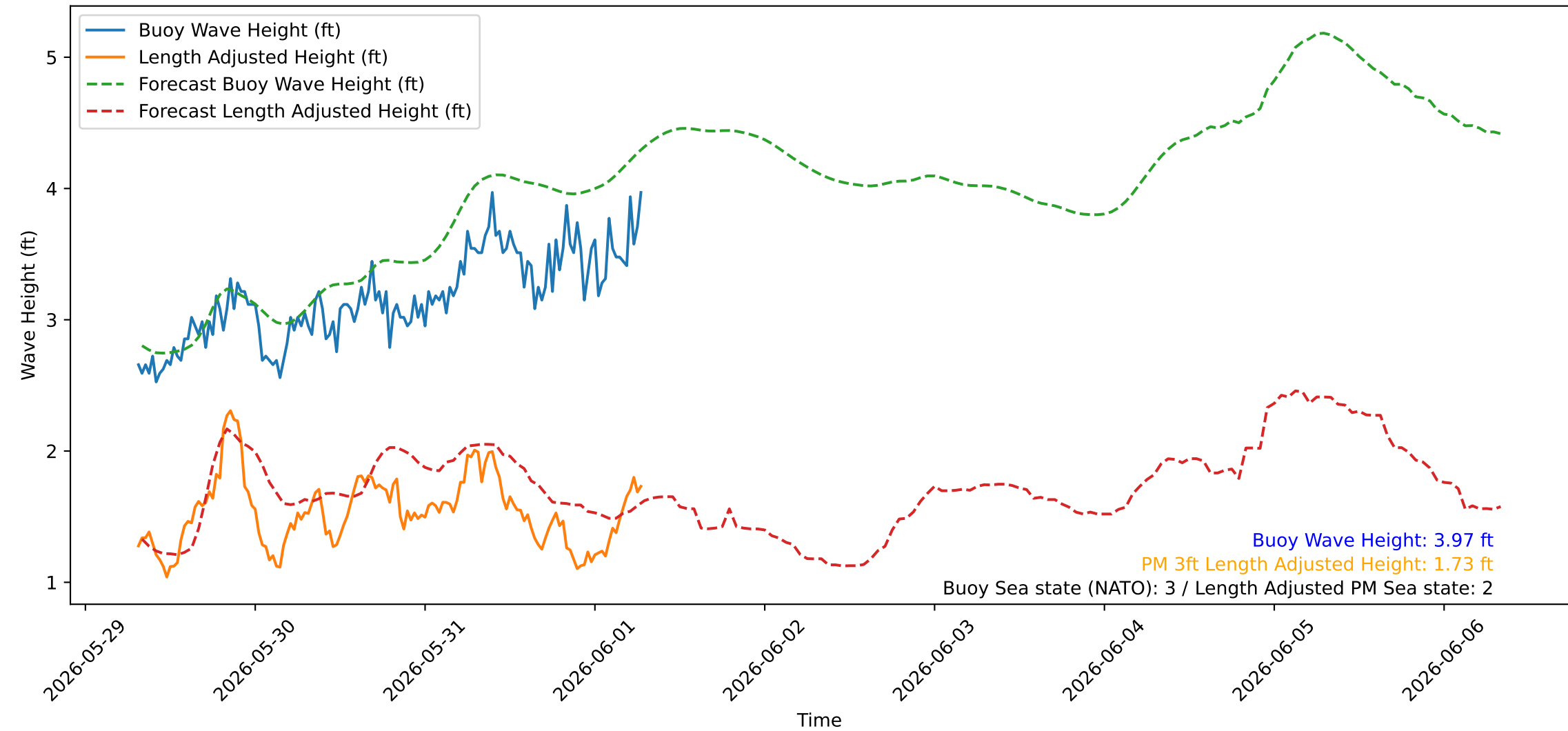
Wave Heights over Time for Green Beach at 2026-06-01 07:31:07
