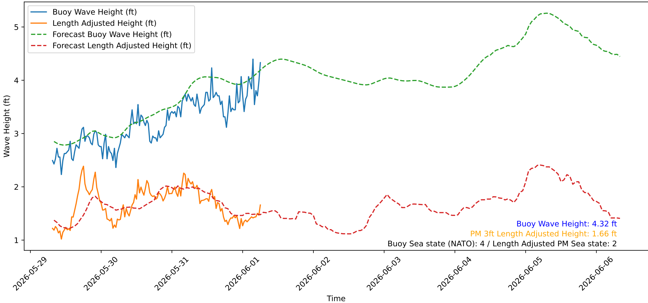
Wave Heights over Time for Oceanside Harbor at 2026-06-01 07:30:25
