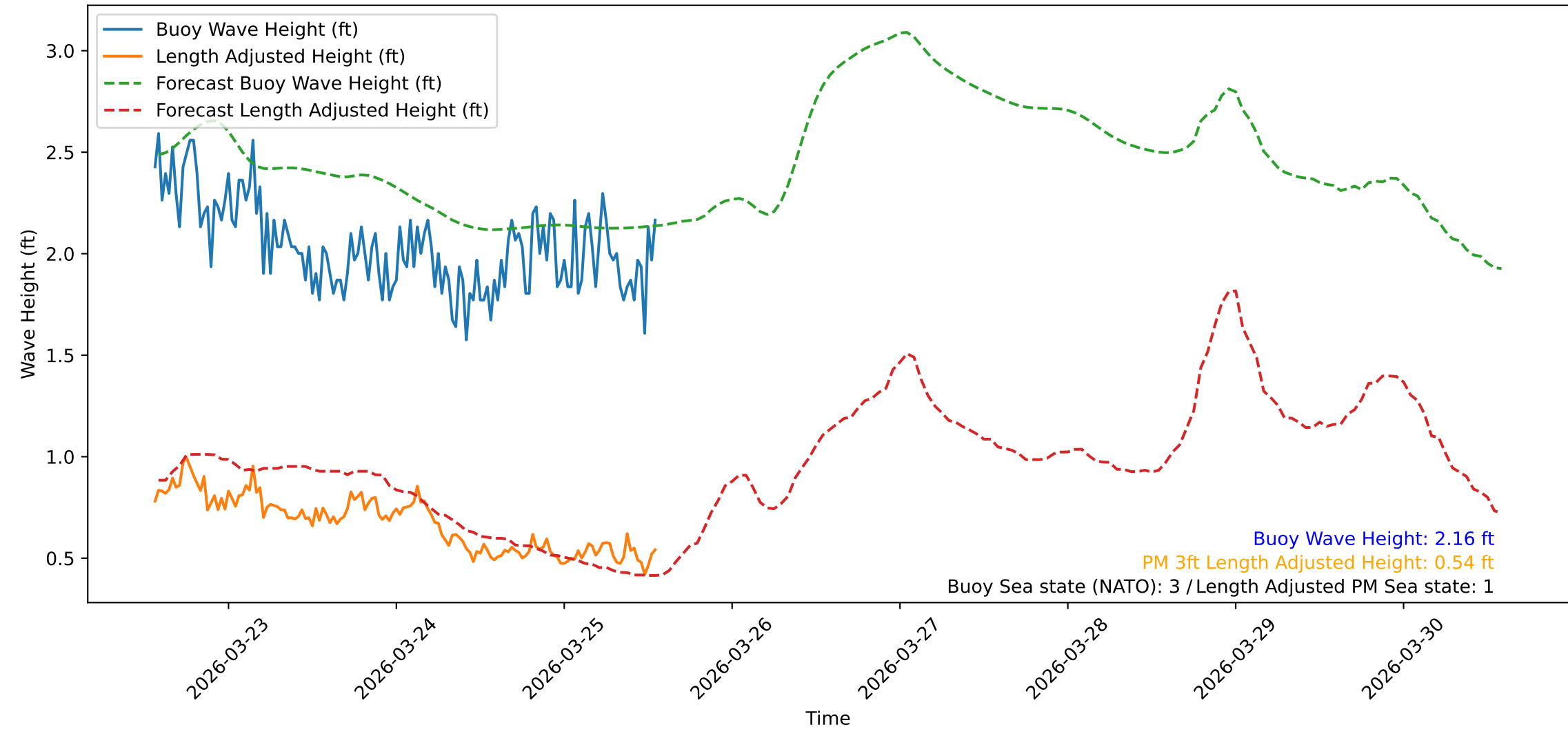
Wave Heights over Time for Oceanside Harbor at 2026-03-25 13:40:31
