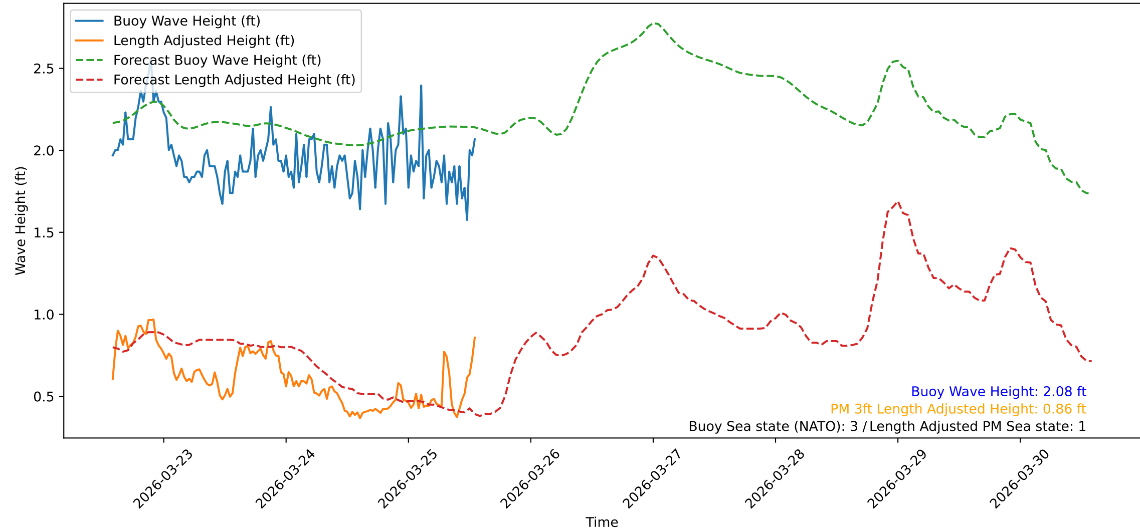
Wave Heights over Time for Red Beach at 2026-03-25 13:40:47
