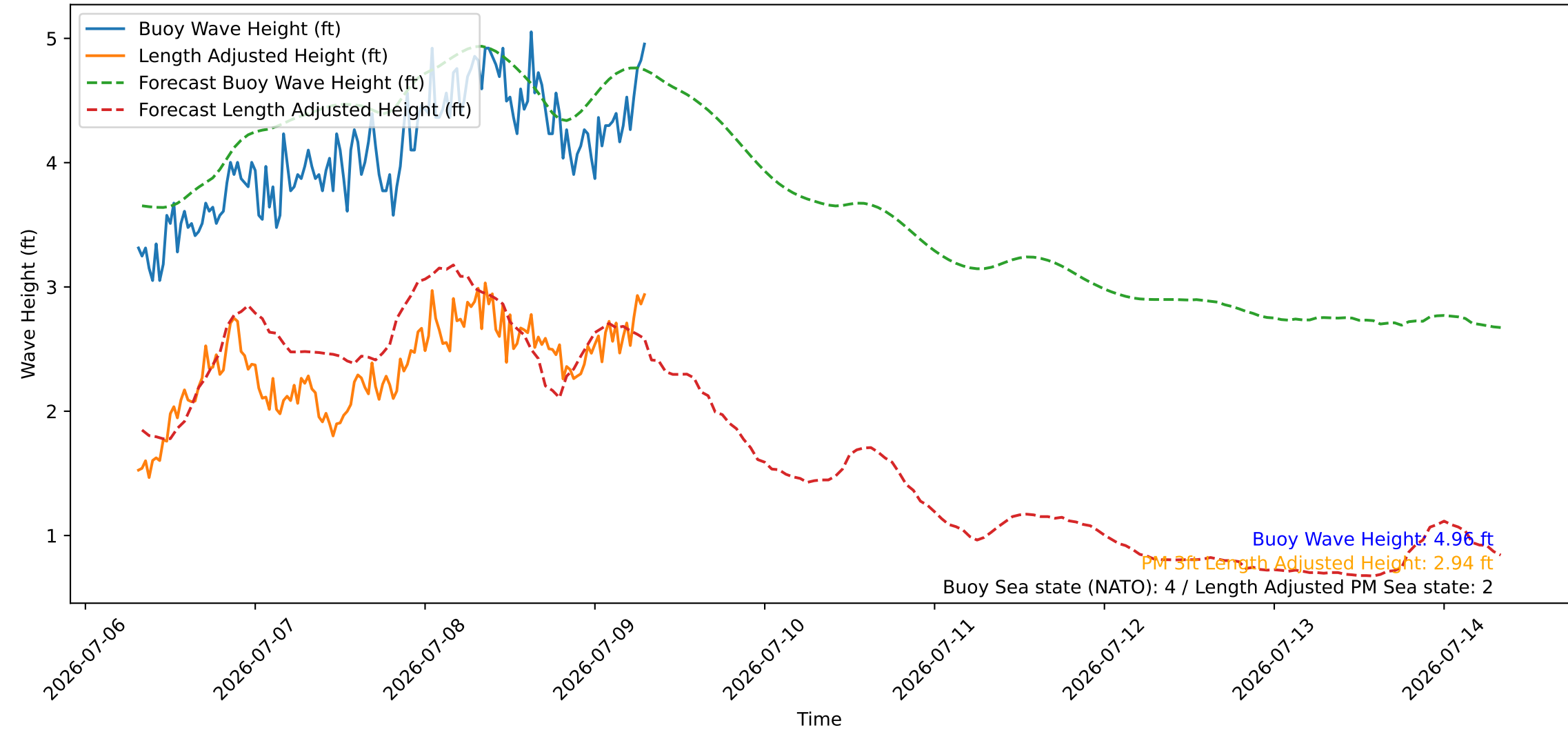
Wave Heights over Time for Oceanside Harbor at 2026-07-09 07:30:27
