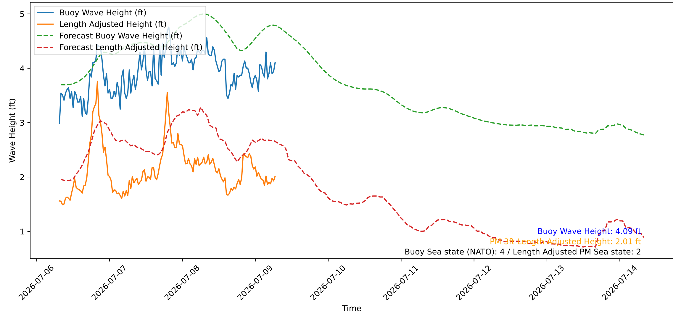
Wave Heights over Time for Green Beach at 2026-07-09 07:31:10
