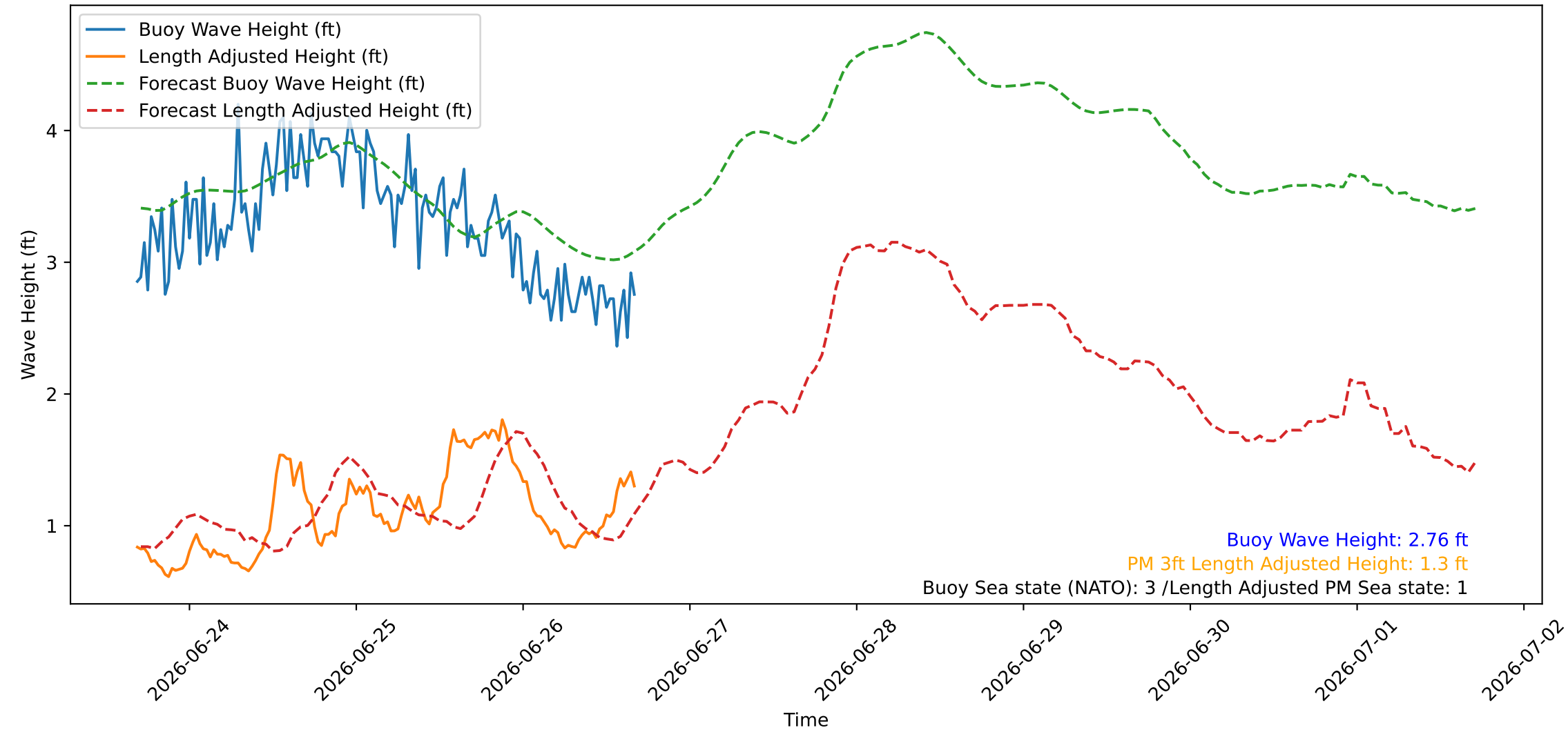
Wave Heights over Time for Green Beach at 2026-06-26 16:41:08
