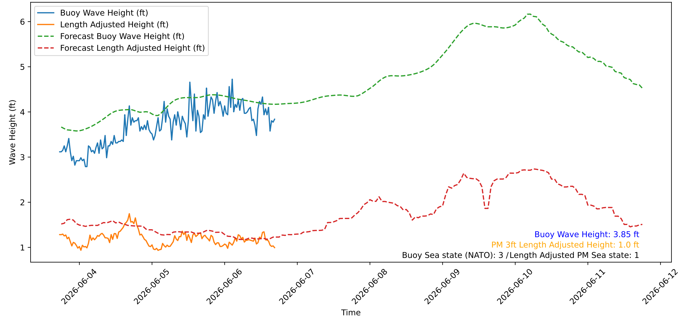
Wave Heights over Time for Green Beach at 2026-06-06 17:31:07
