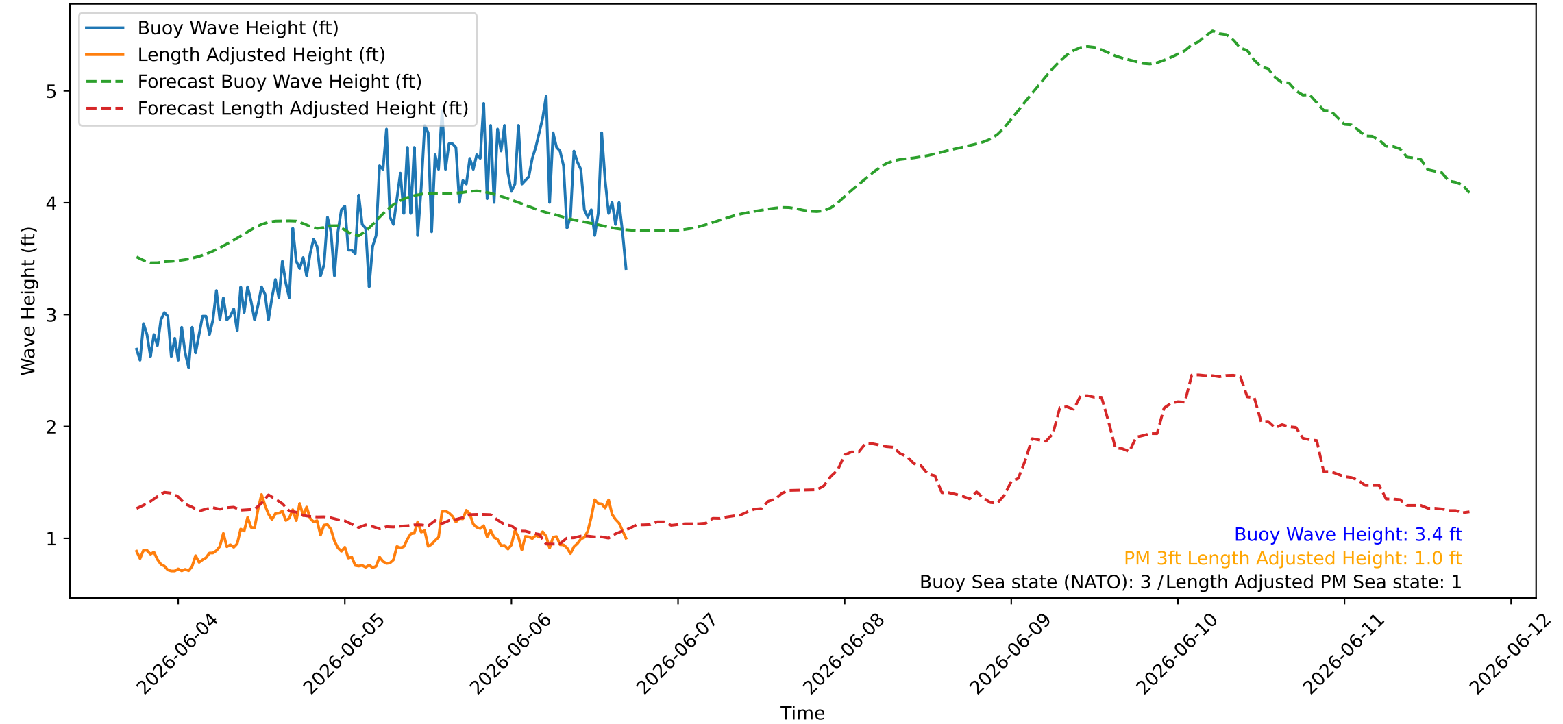
Wave Heights over Time for Red Beach at 2026-06-06 17:30:45
