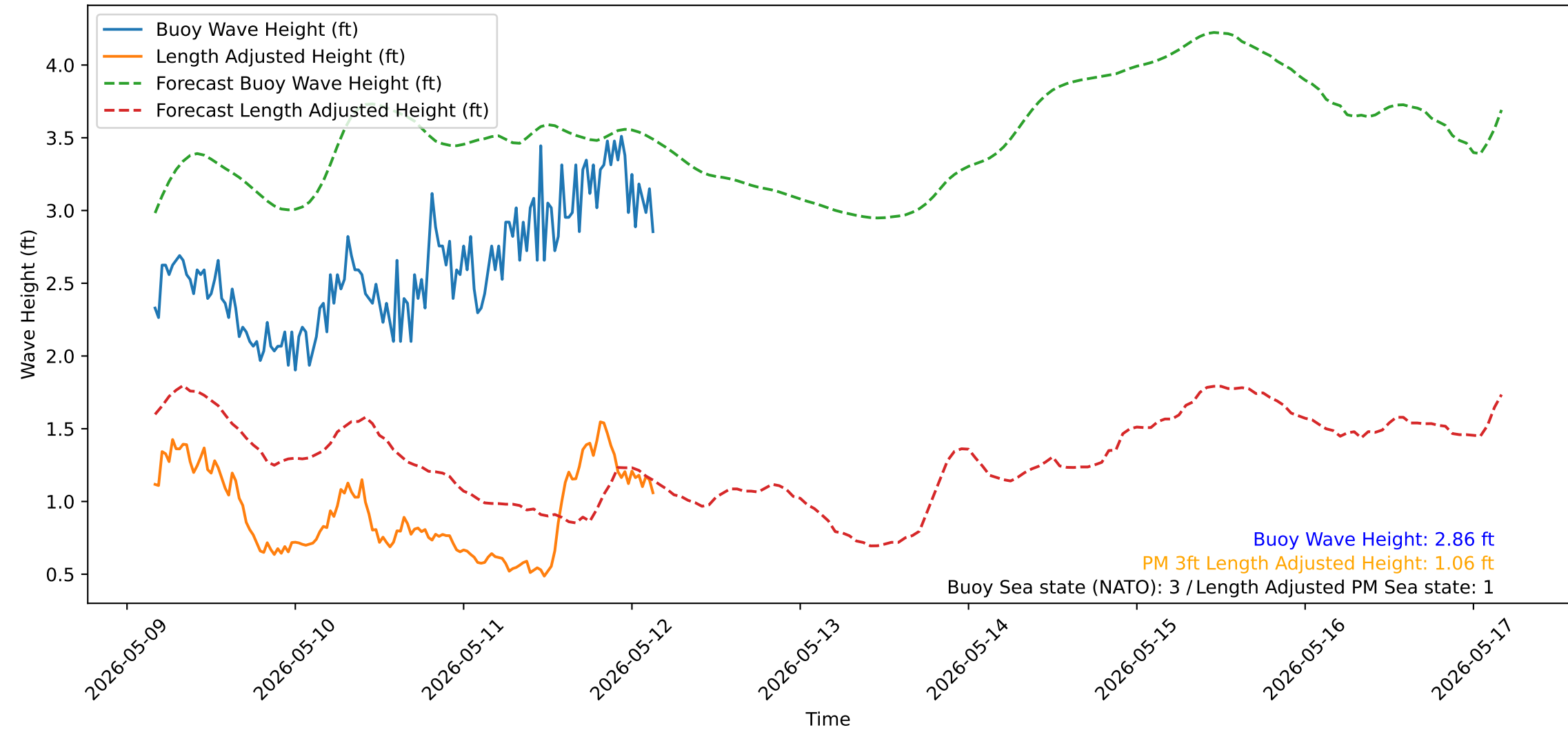
Wave Heights over Time for Green Beach at 2026-05-12 04:01:13
