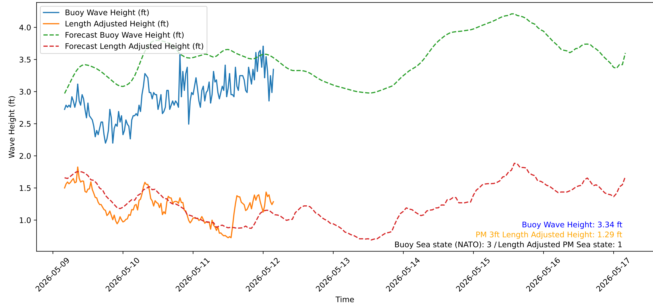
Wave Heights over Time for Oceanside Harbor at 2026-05-12 04:00:31
