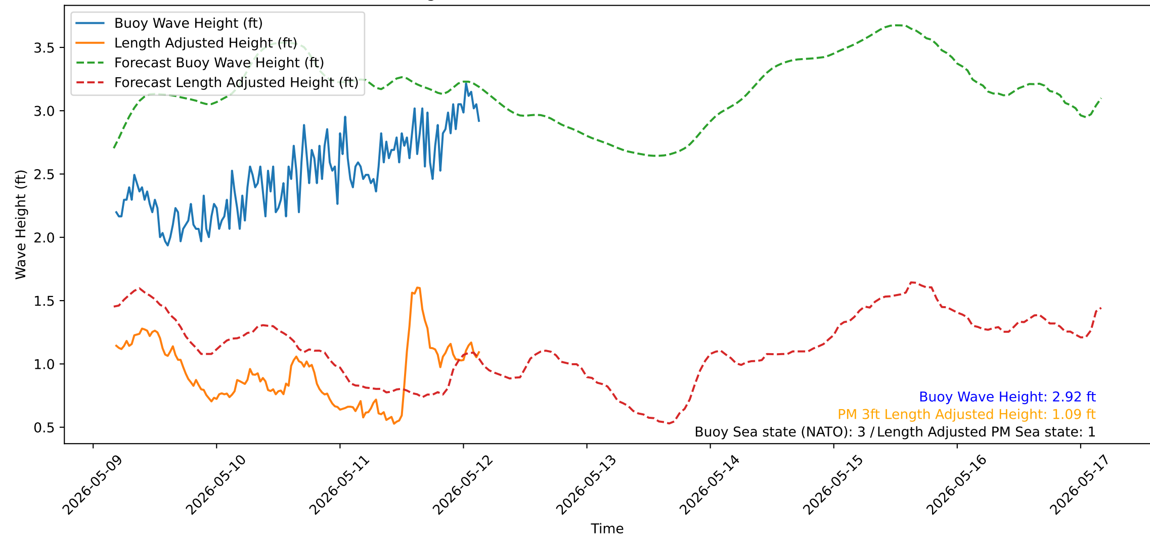
Wave Heights over Time for Red Beach at 2026-05-12 04:00:50
