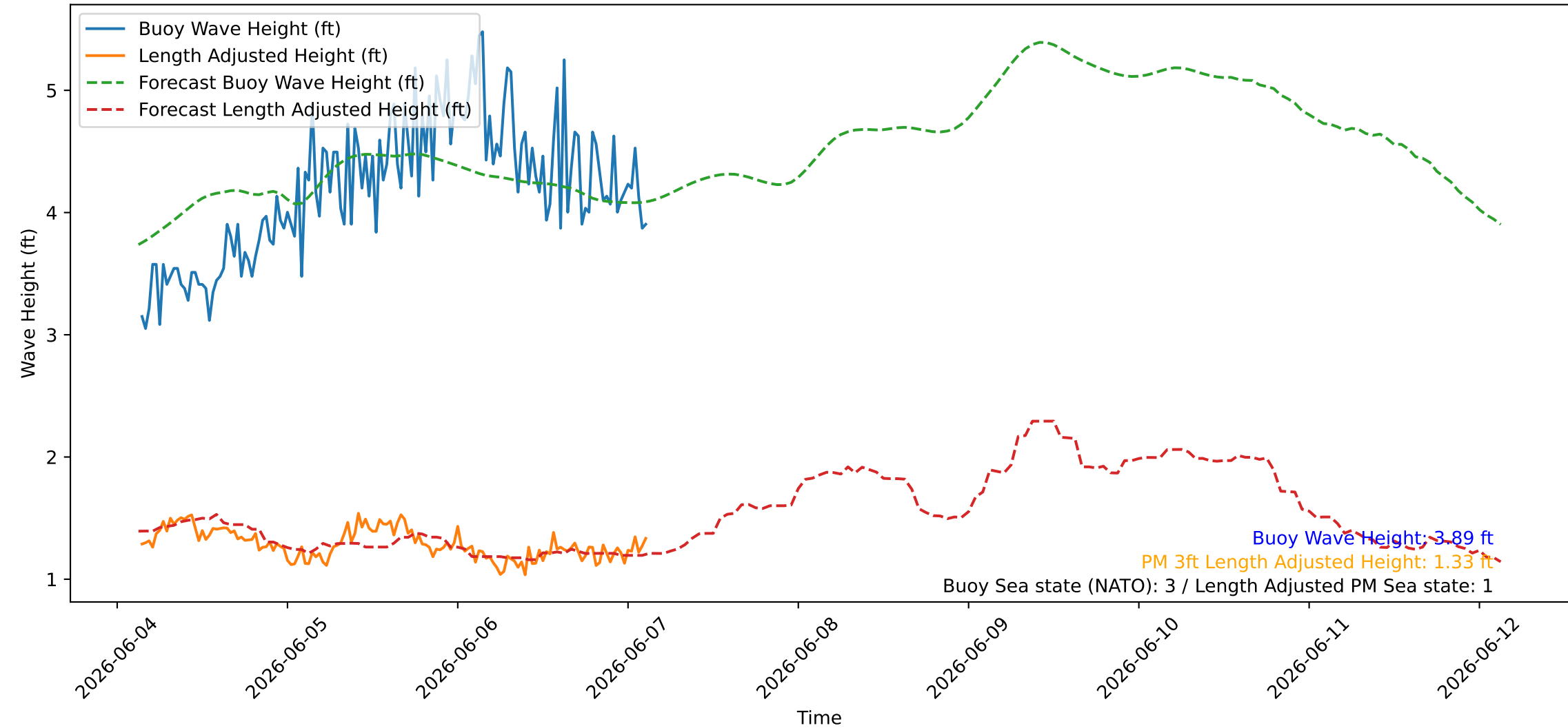
Wave Heights over Time for Oceanside Harbor at 2026-06-07 03:20:26
