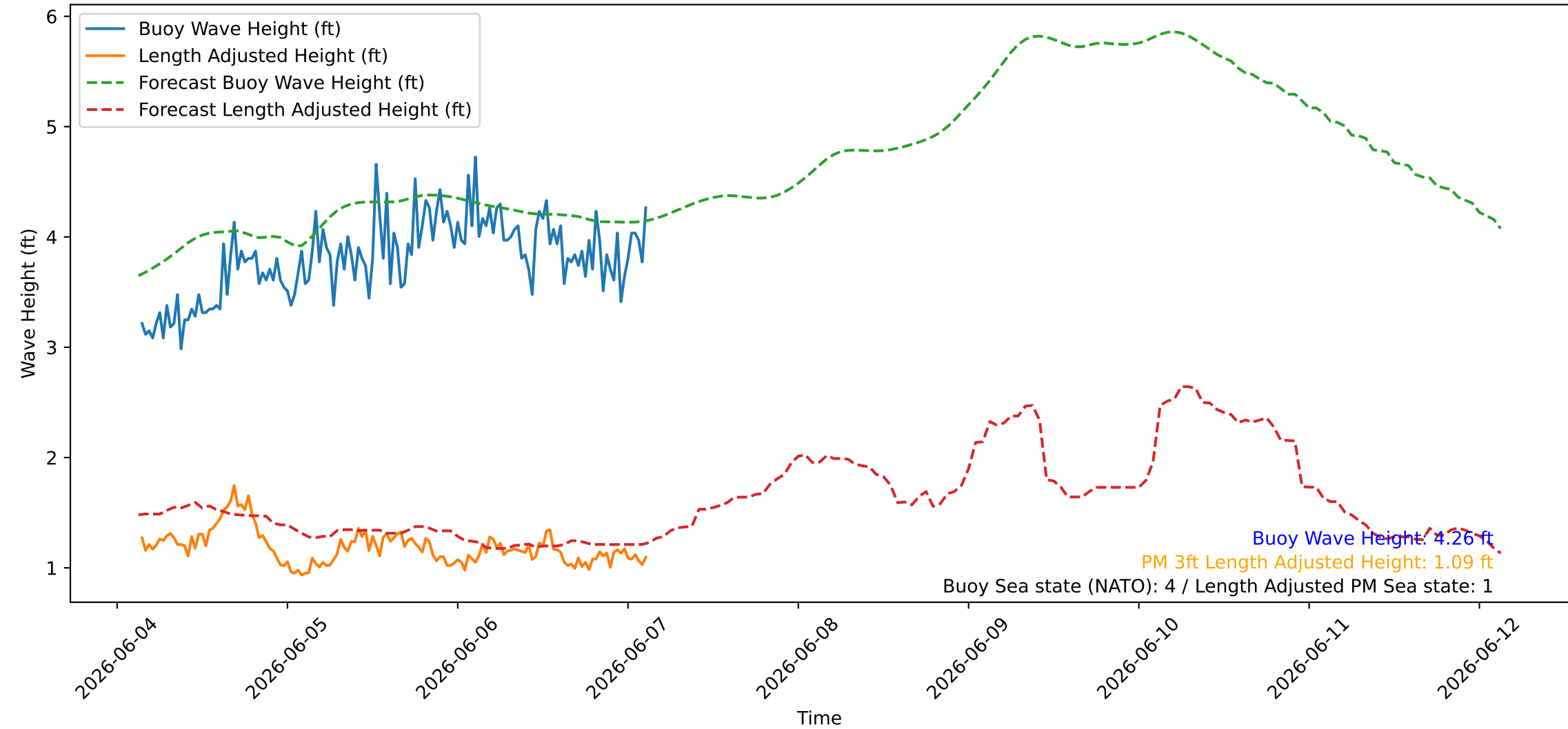
Wave Heights over Time for Green Beach at 2026-06-07 03:21:08
