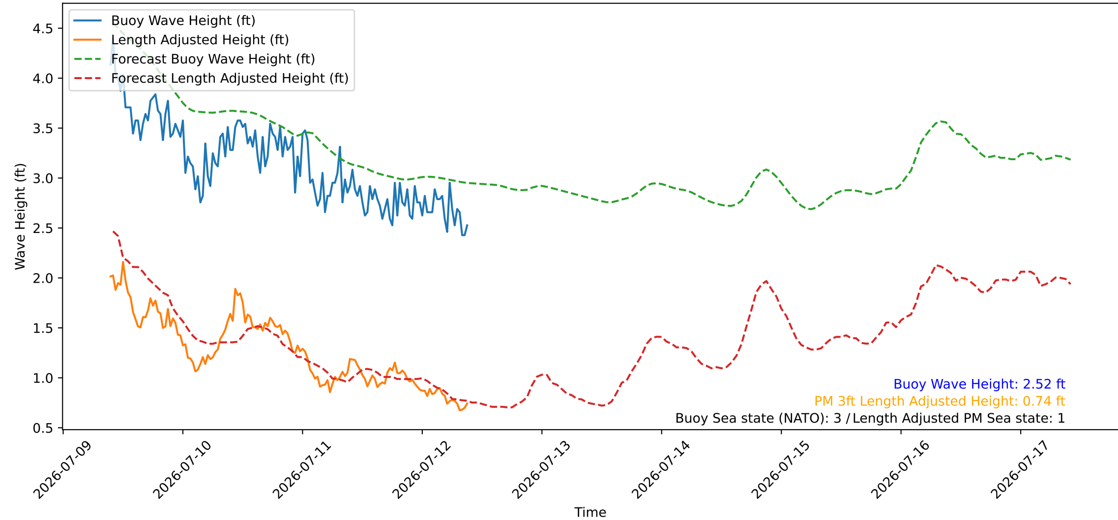
Wave Heights over Time for Green Beach at 2026-07-12 09:41:09
