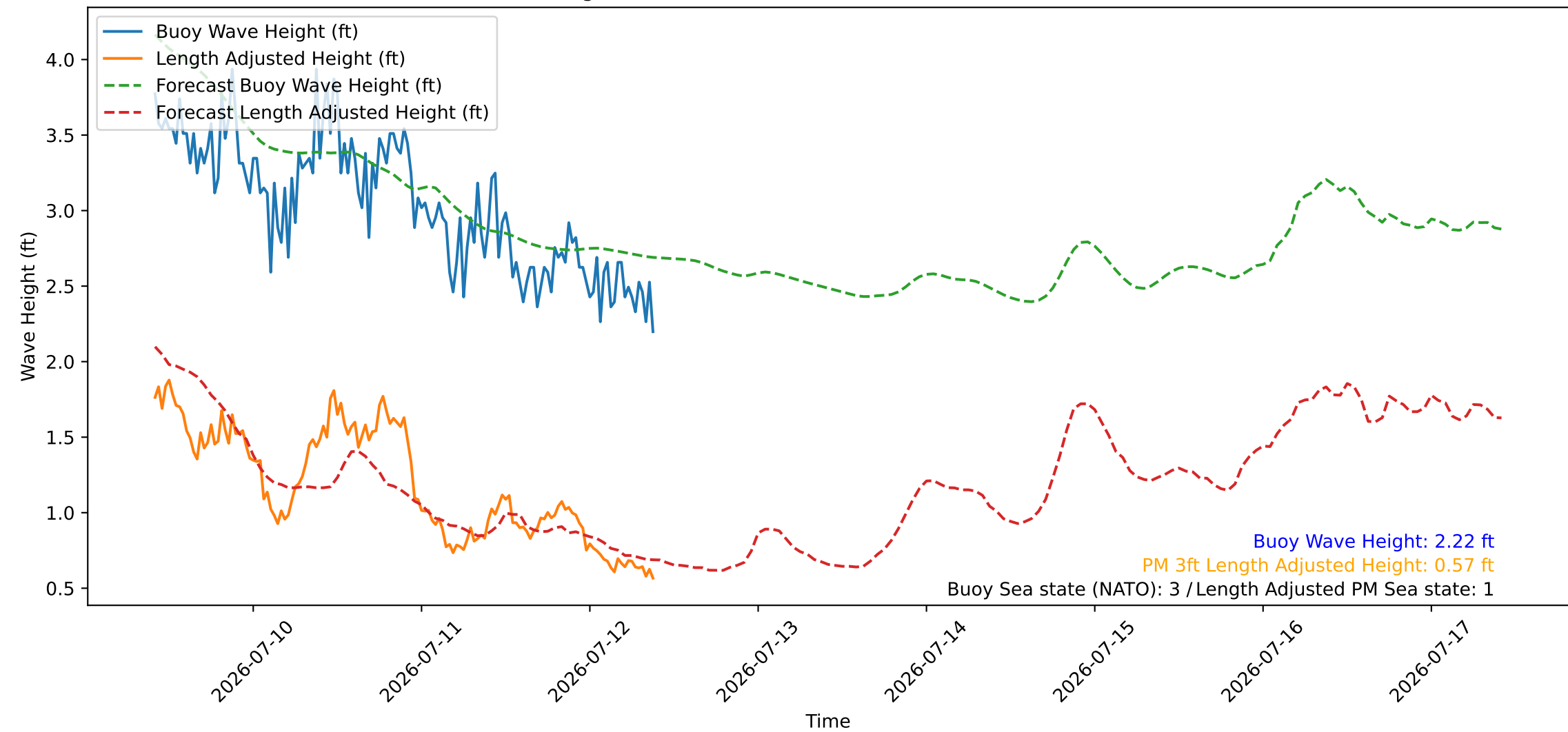
Wave Heights over Time for Red Beach at 2026-07-12 09:40:46
