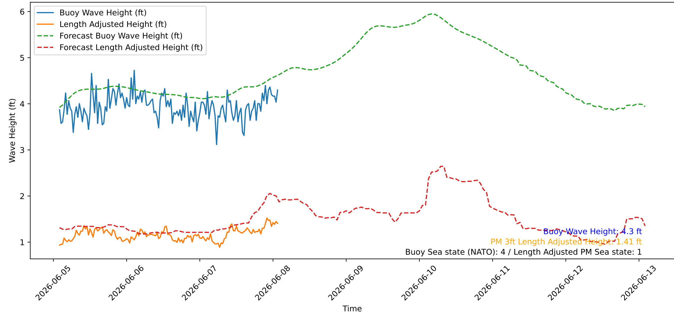
Wave Heights over Time for Green Beach at 2026-06-08 02:11:09
