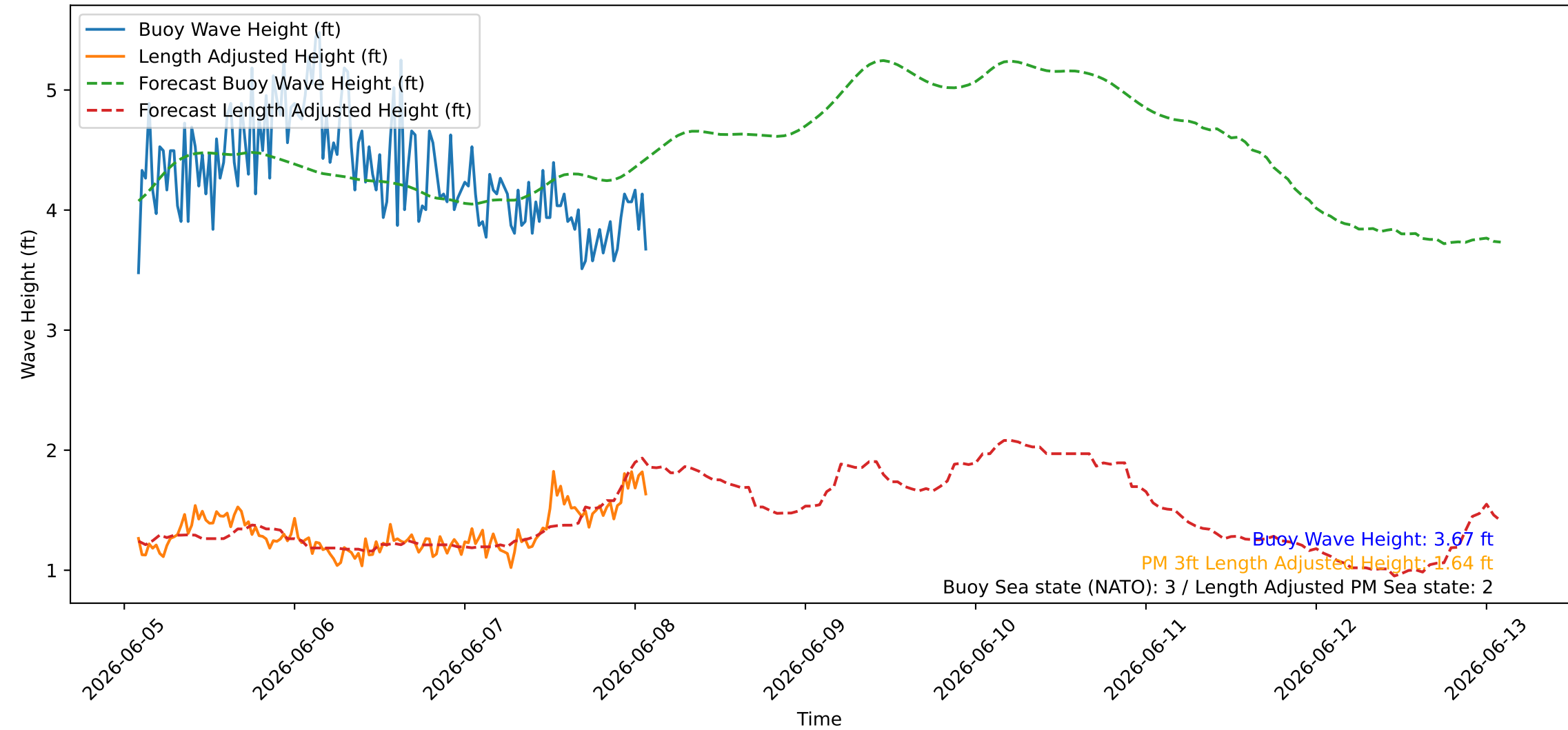
Wave Heights over Time for Oceanside Harbor at 2026-06-08 02:10:27
