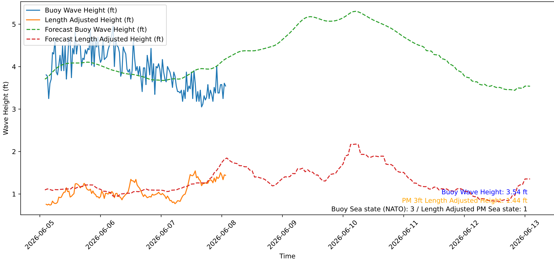
Wave Heights over Time for Red Beach at 2026-06-08 02:10:46
