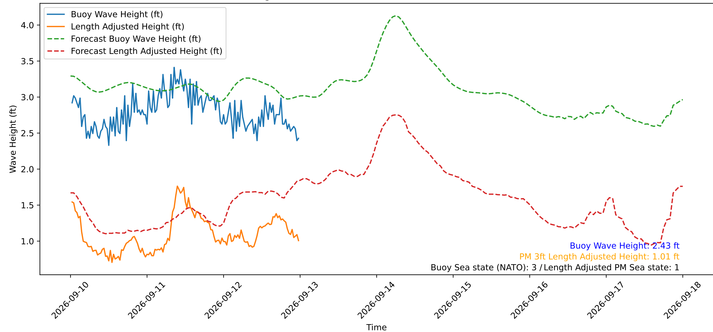
Wave Heights over Time for Red Beach at 2026-09-13 00:10:49
