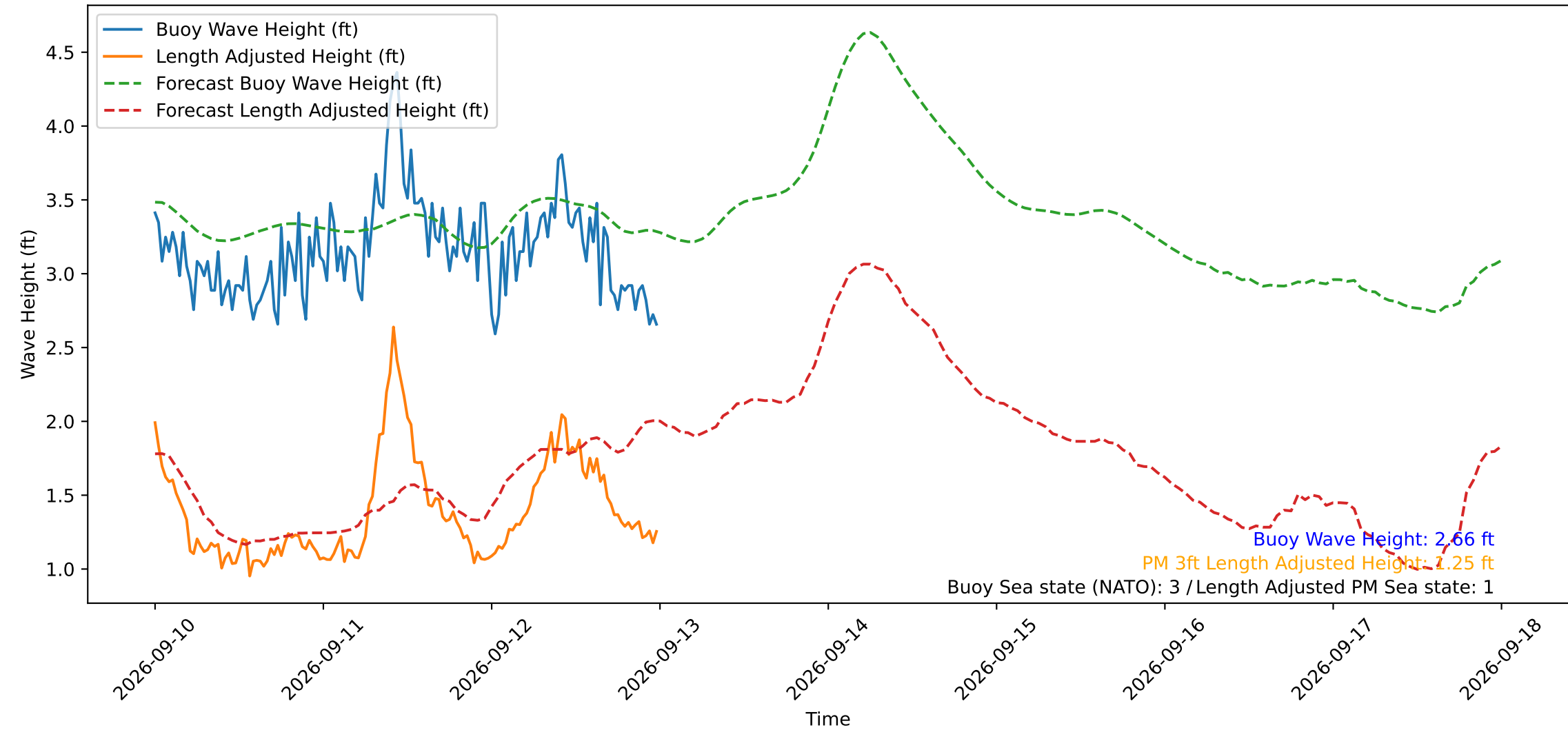
Wave Heights over Time for Oceanside Harbor at 2026-09-13 00:10:30
