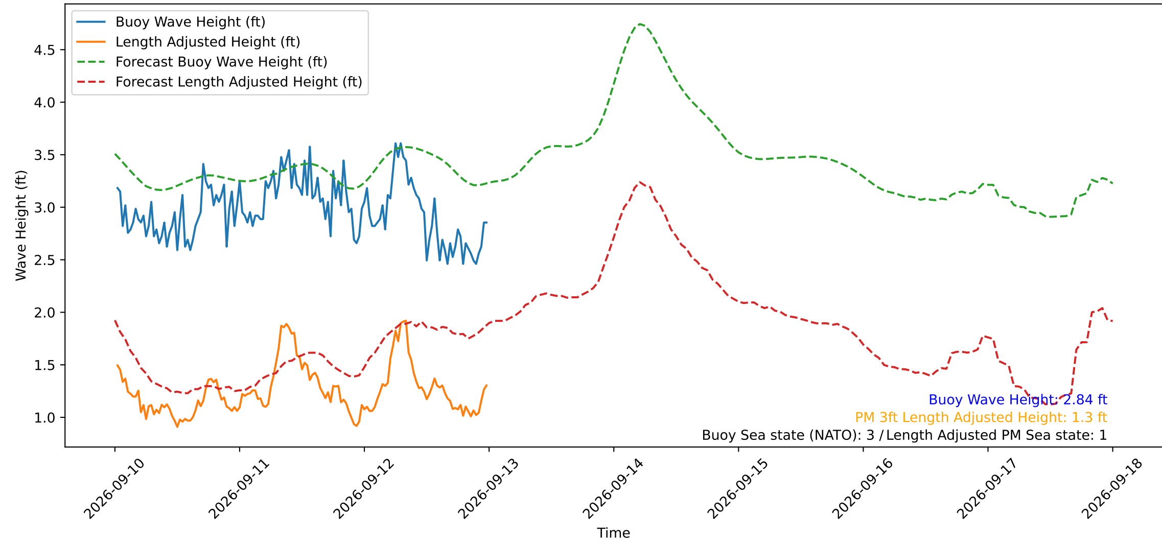
Wave Heights over Time for Green Beach at 2026-09-13 00:11:11
