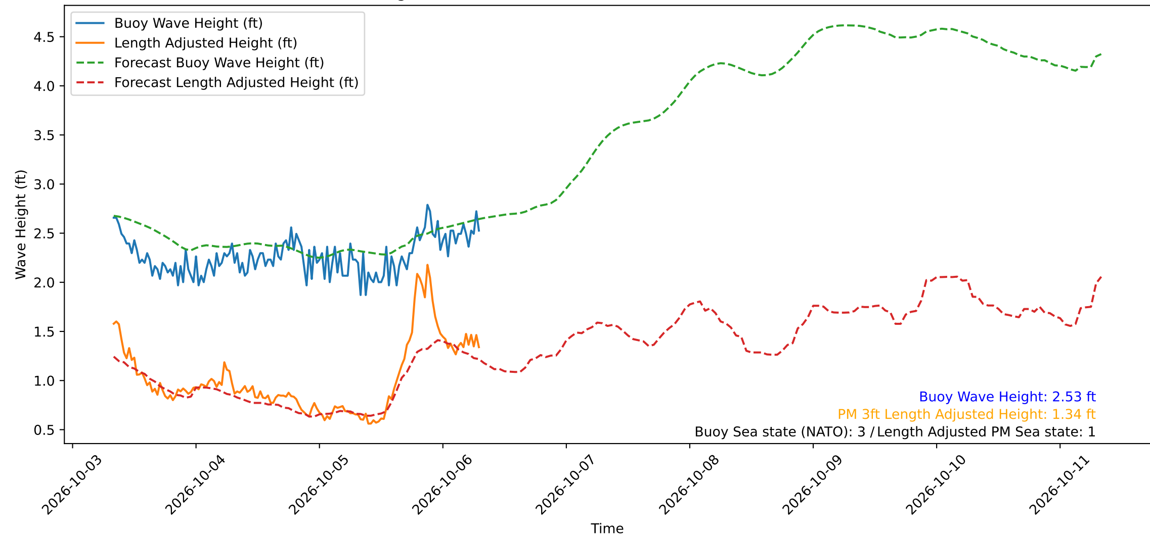
Wave Heights over Time for Oceanside Harbor at 2026-10-06 07:50:30
