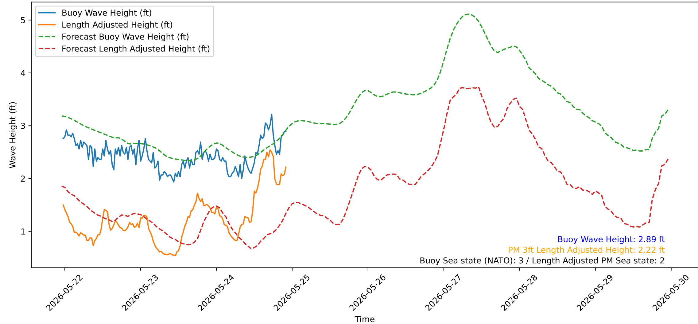
Wave Heights over Time for Red Beach at 2026-05-24 23:00:51
