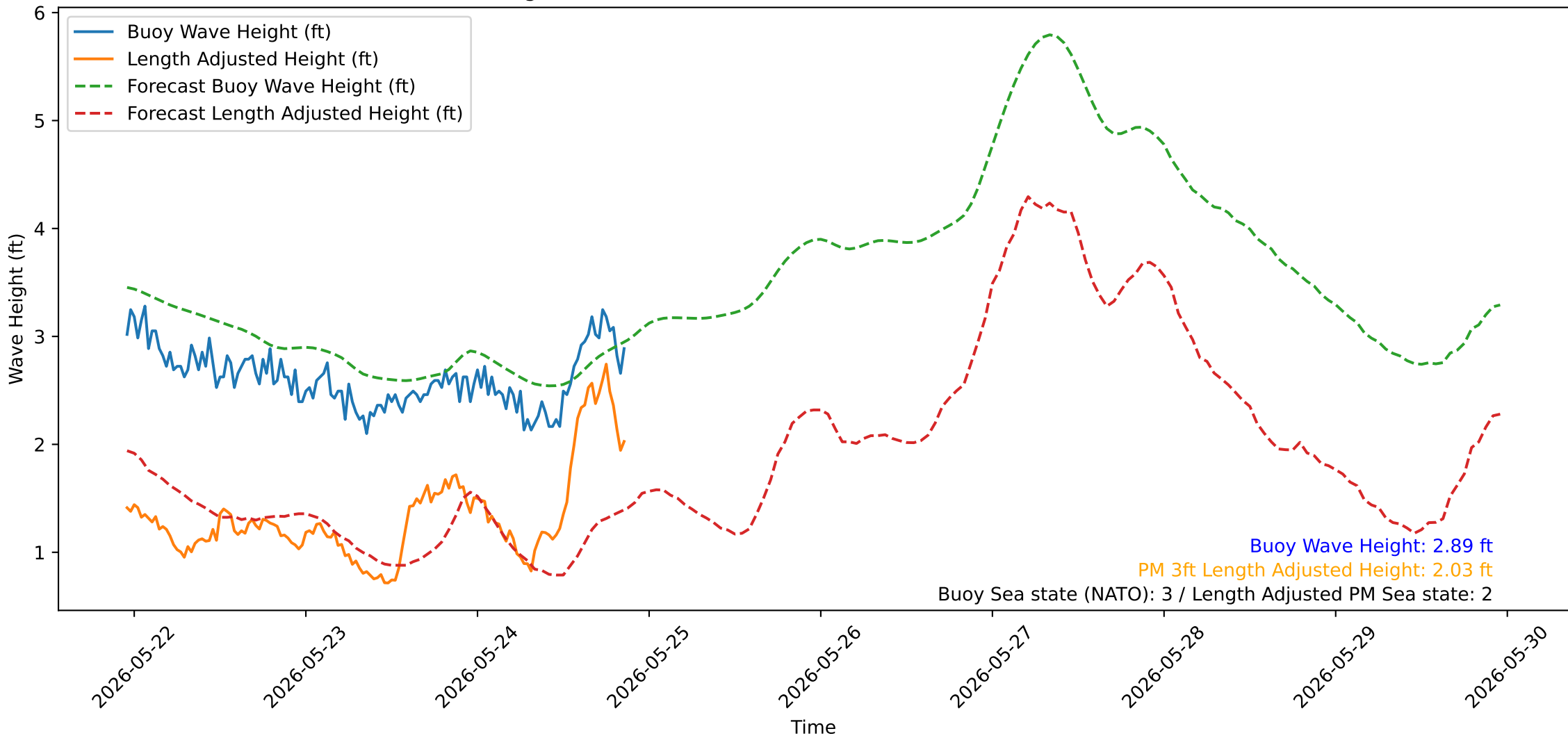
Wave Heights over Time for Oceanside Harbor at 2026-05-24 23:00:31
