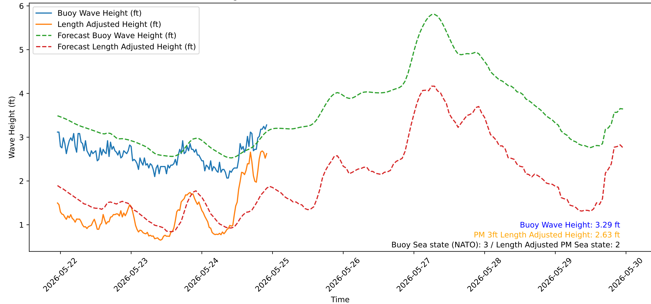
Wave Heights over Time for Green Beach at 2026-05-24 23:01:14
