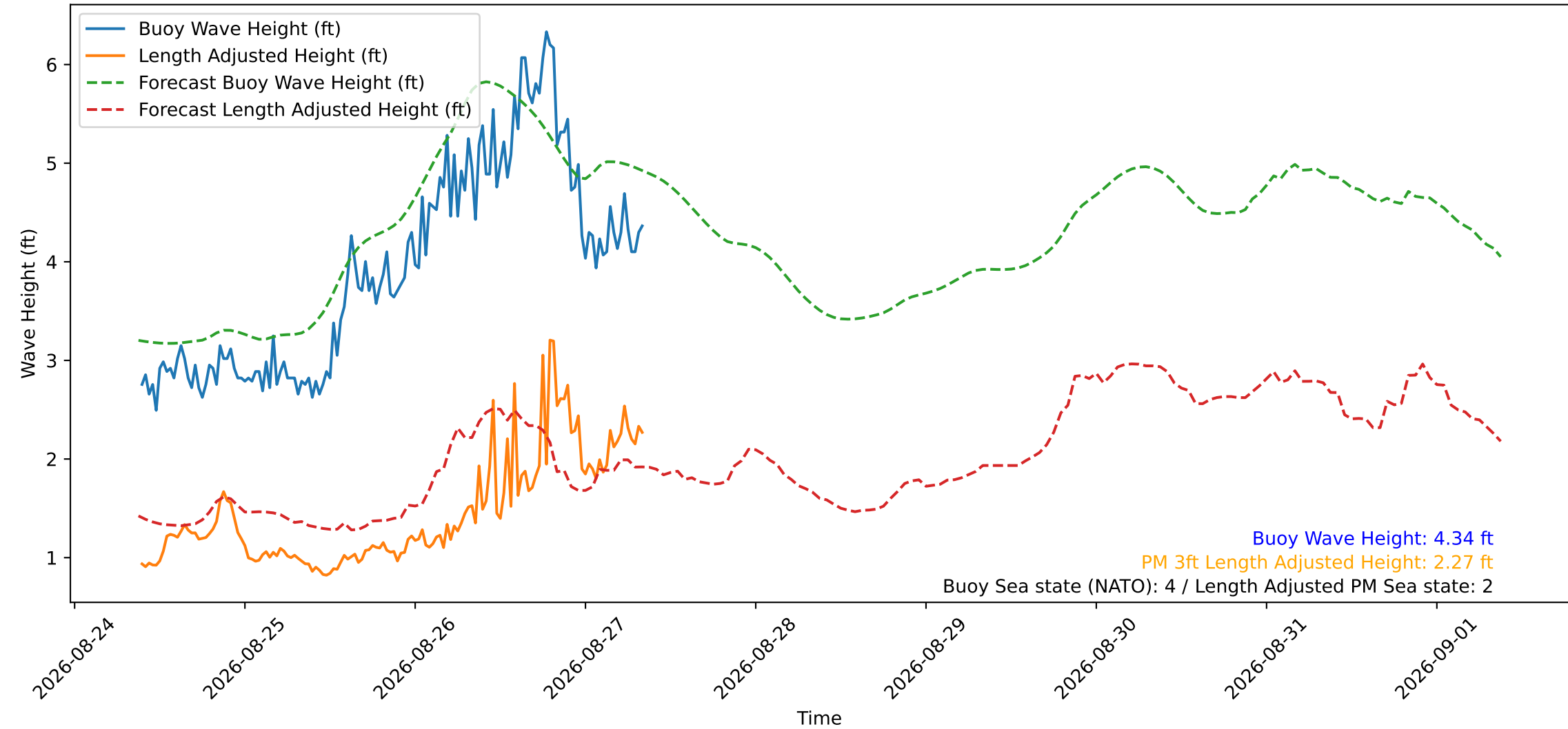
Wave Heights over Time for Green Beach at 2026-08-27 09:01:13
