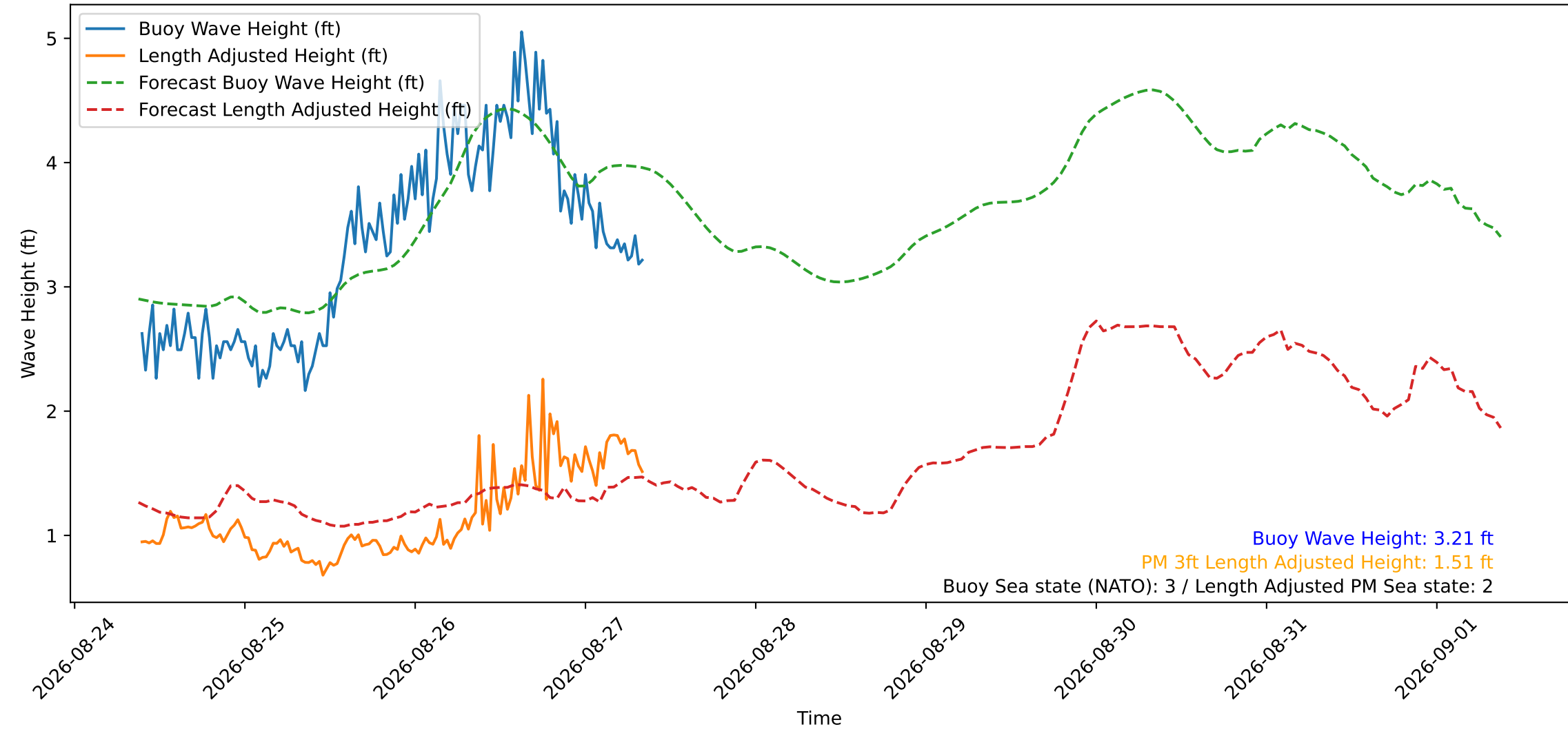
Wave Heights over Time for Red Beach at 2026-08-27 09:00:50
