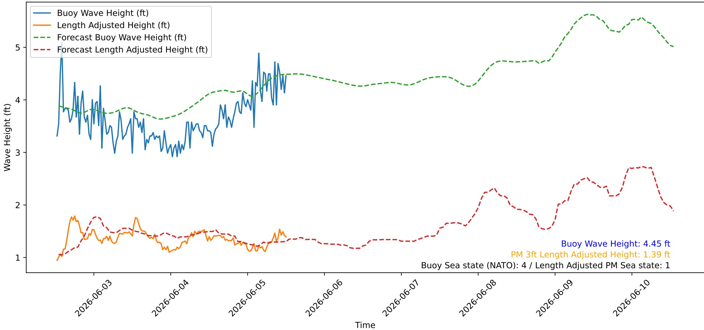
Wave Heights over Time for Oceanside Harbor at 2026-06-05 12:30:26
