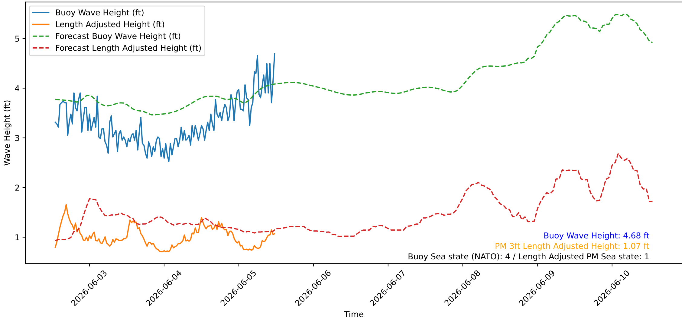
Wave Heights over Time for Red Beach at 2026-06-05 12:30:45
