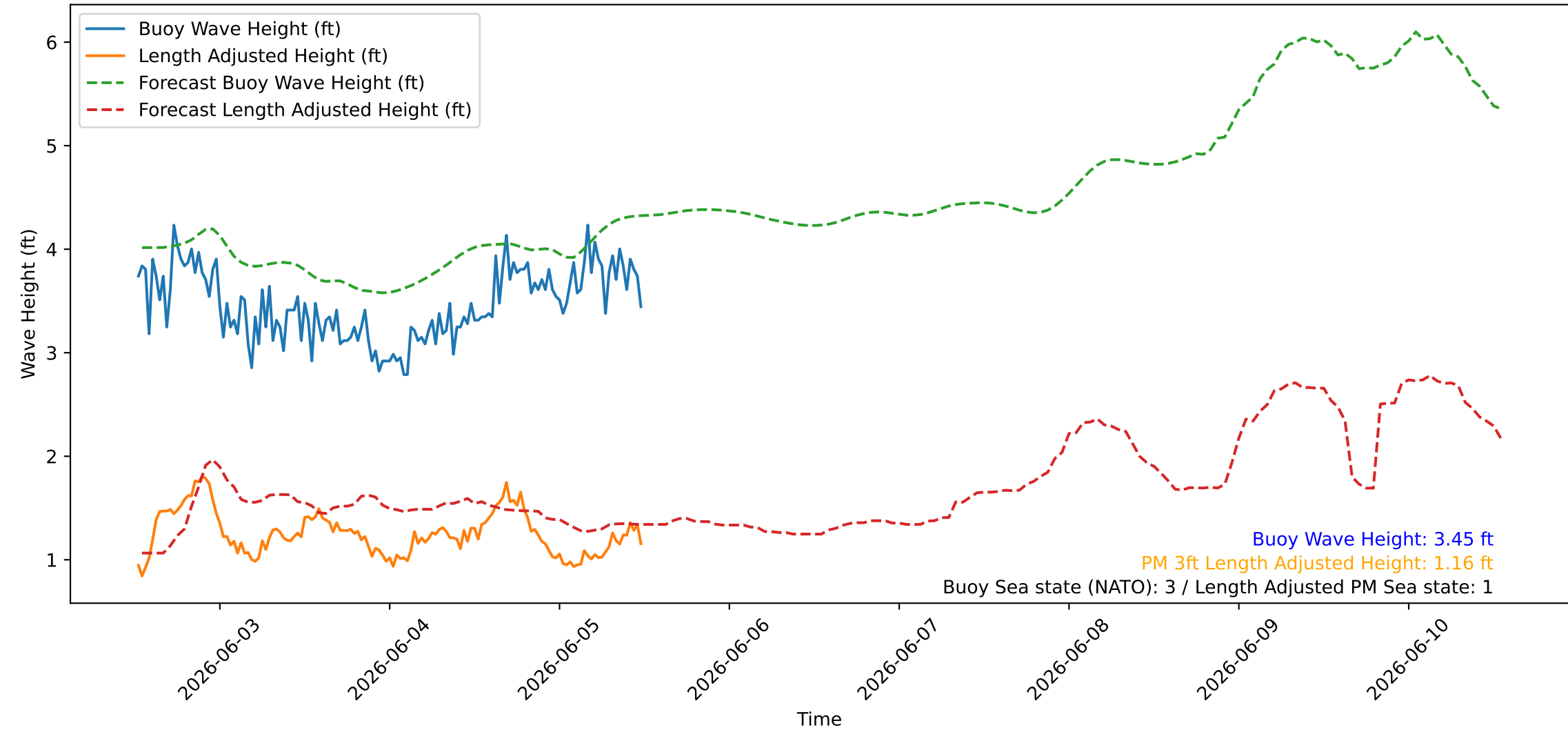
Wave Heights over Time for Green Beach at 2026-06-05 12:31:07
