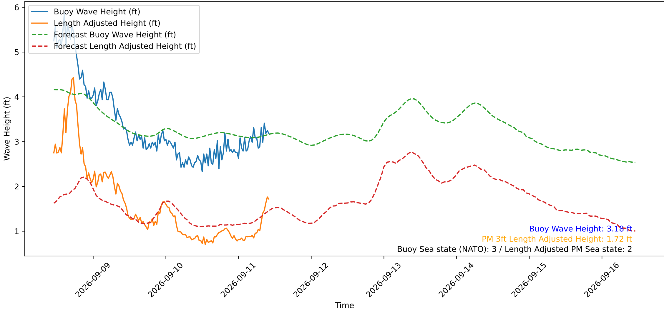
Wave Heights over Time for Red Beach at 2026-09-11 10:40:49
