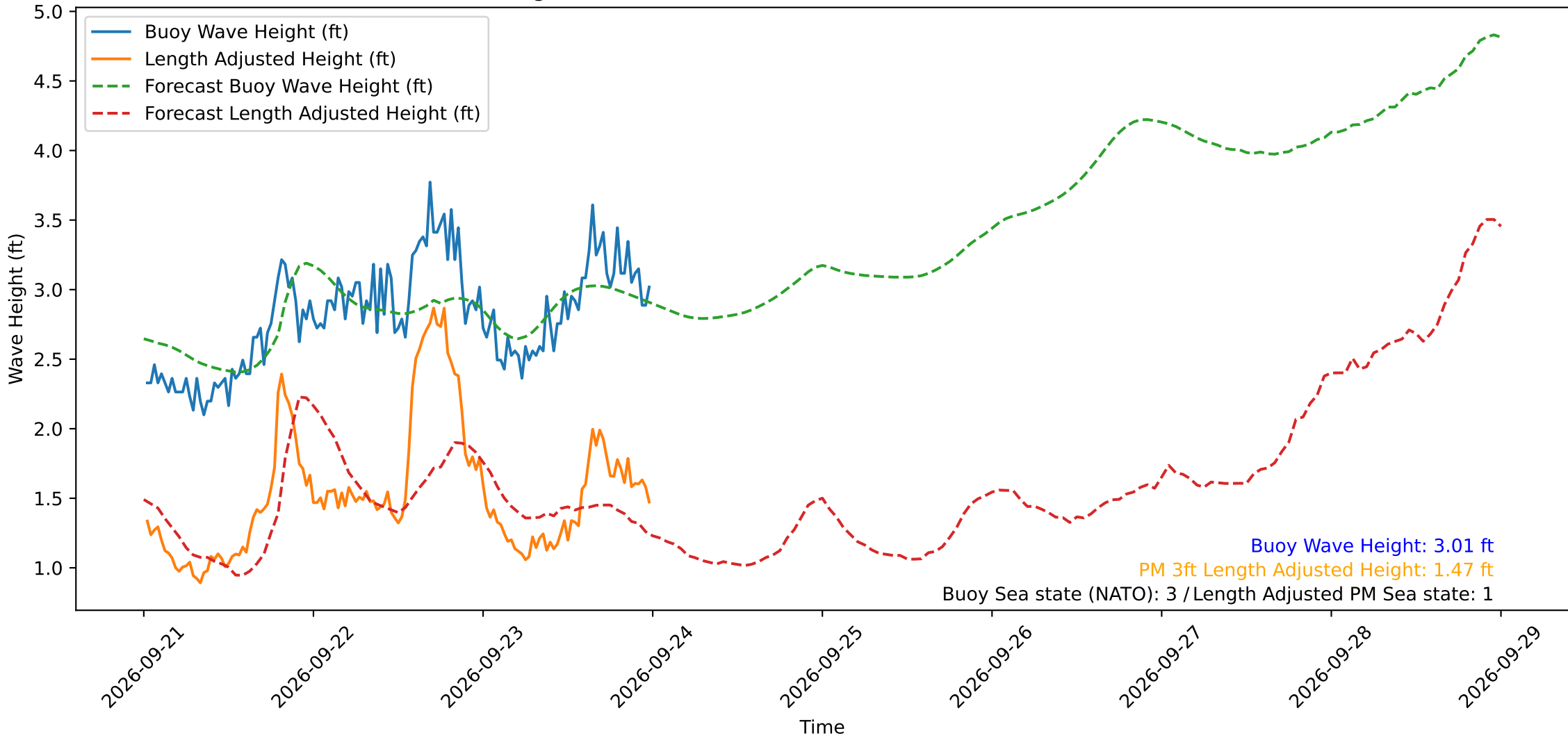
Wave Heights over Time for Oceanside Harbor at 2026-09-24 00:20:30
