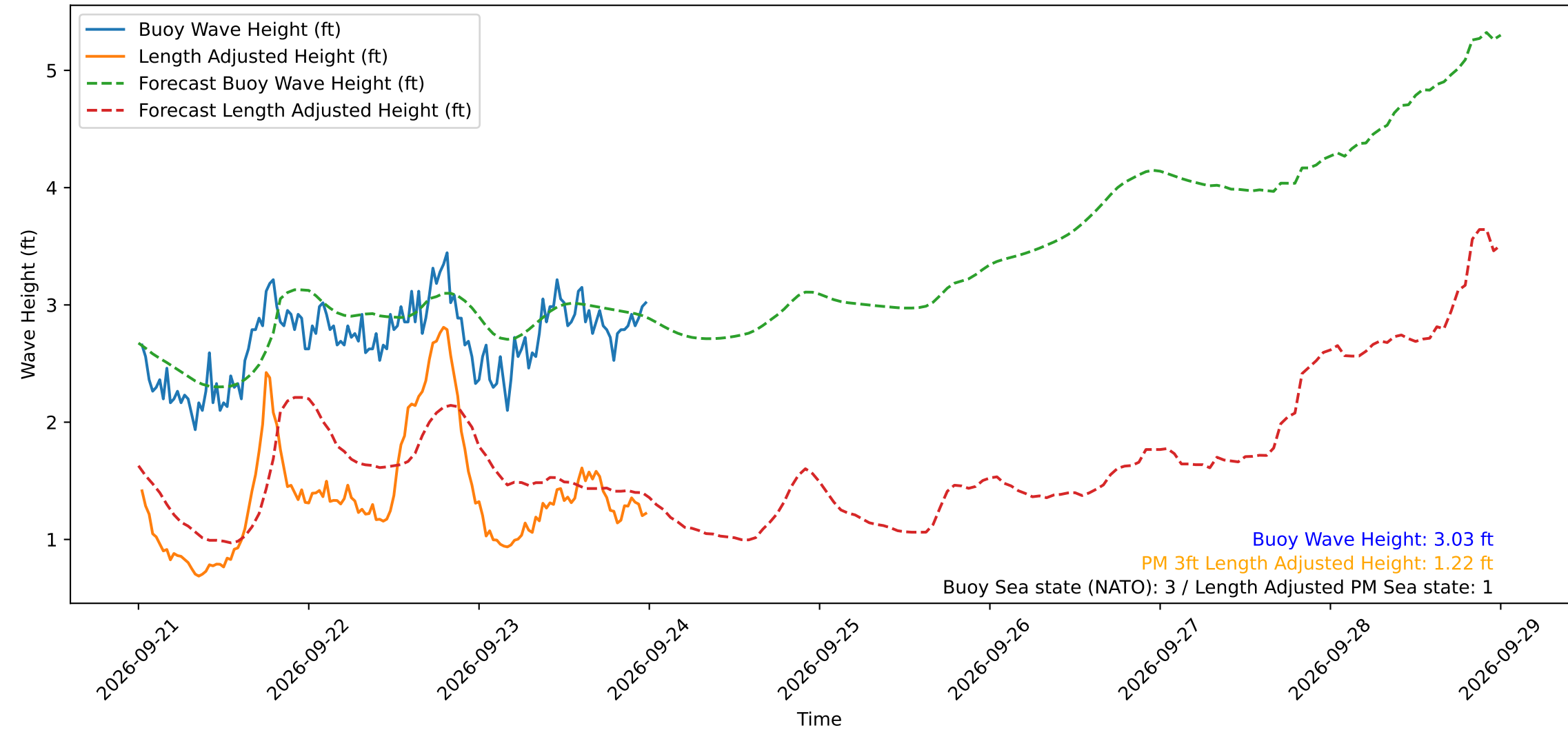
Wave Heights over Time for Green Beach at 2026-09-24 00:21:15
