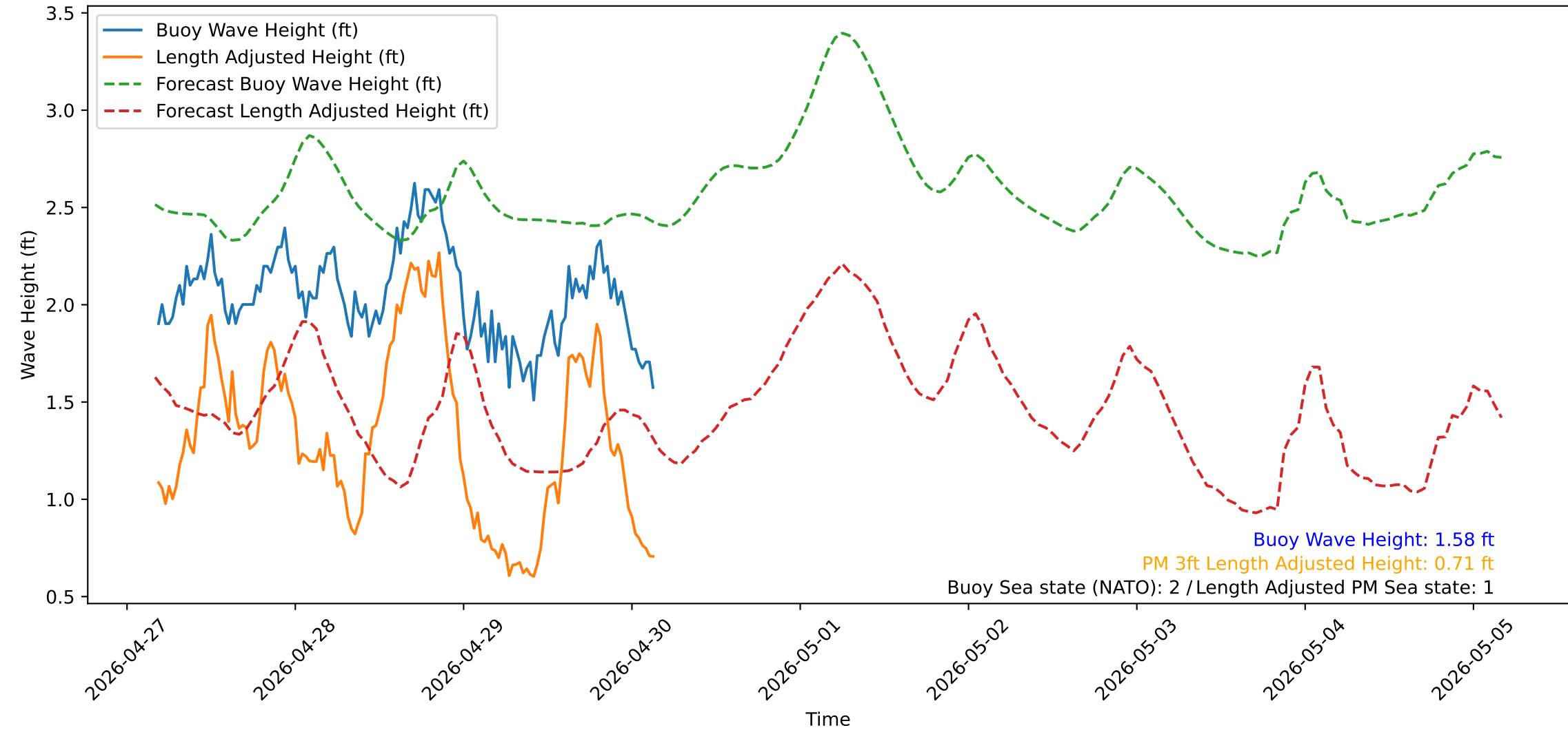
Wave Heights over Time for Red Beach at 2026-04-30 04:00:51
