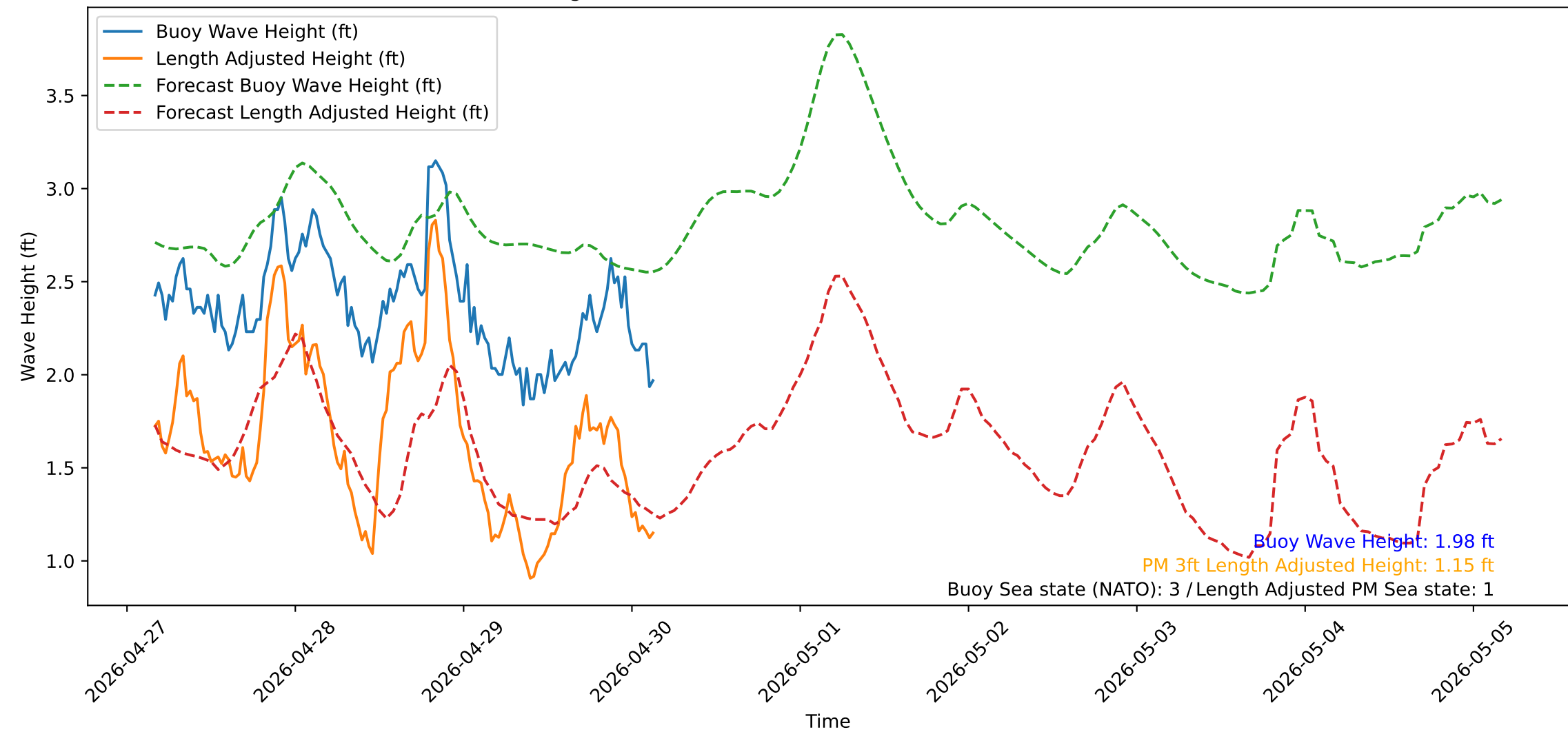
Wave Heights over Time for Green Beach at 2026-04-30 04:01:13
