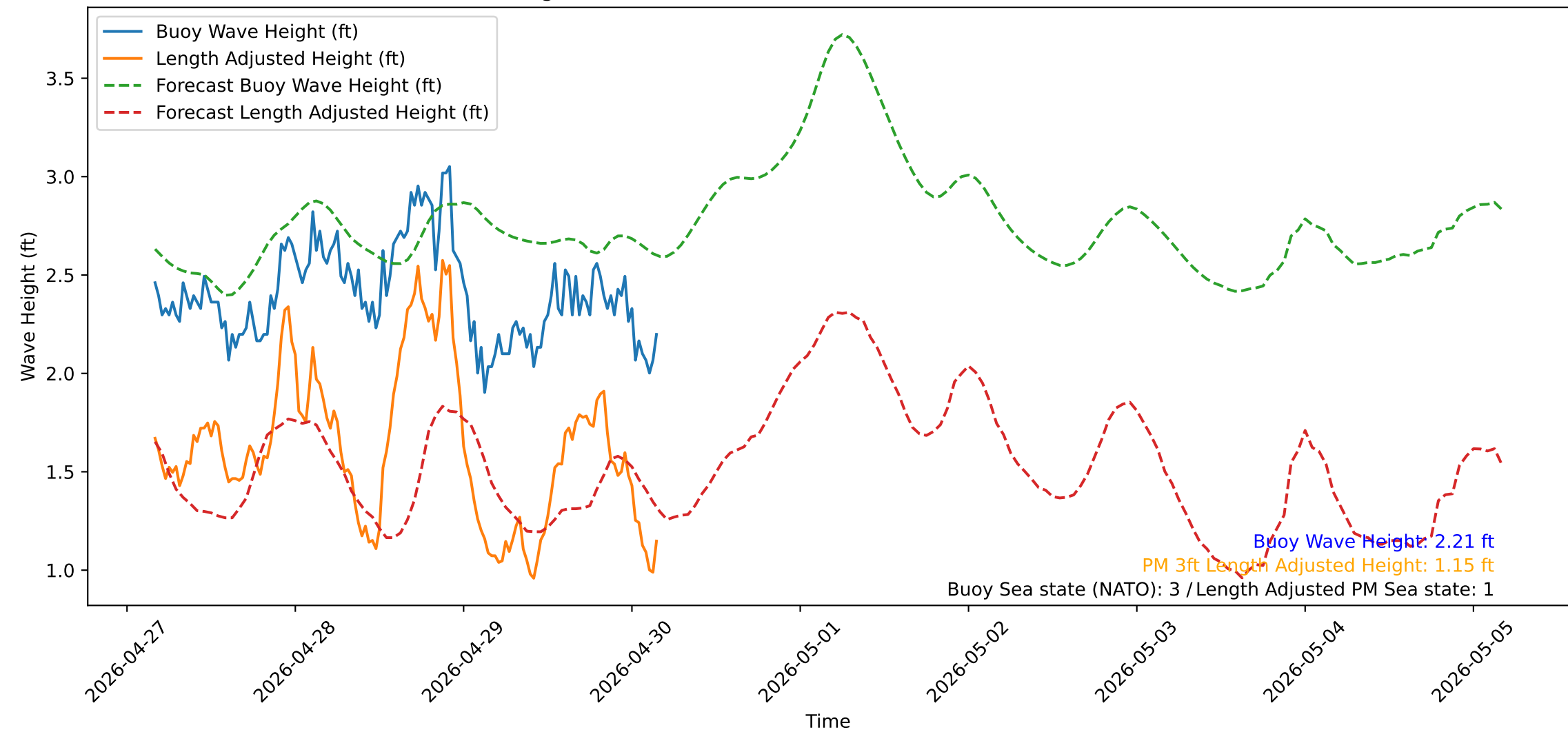
Wave Heights over Time for Oceanside Harbor at 2026-04-30 04:00:31
