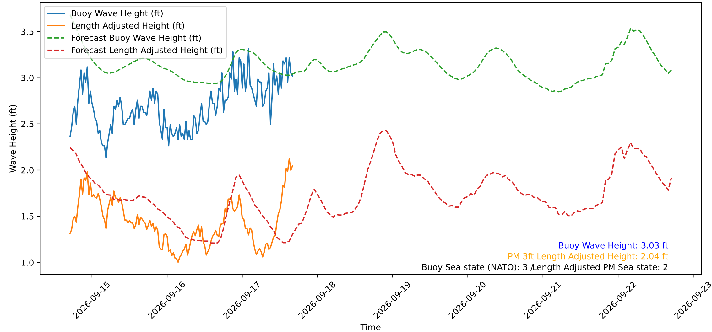
Wave Heights over Time for Green Beach at 2026-09-17 16:51:14
