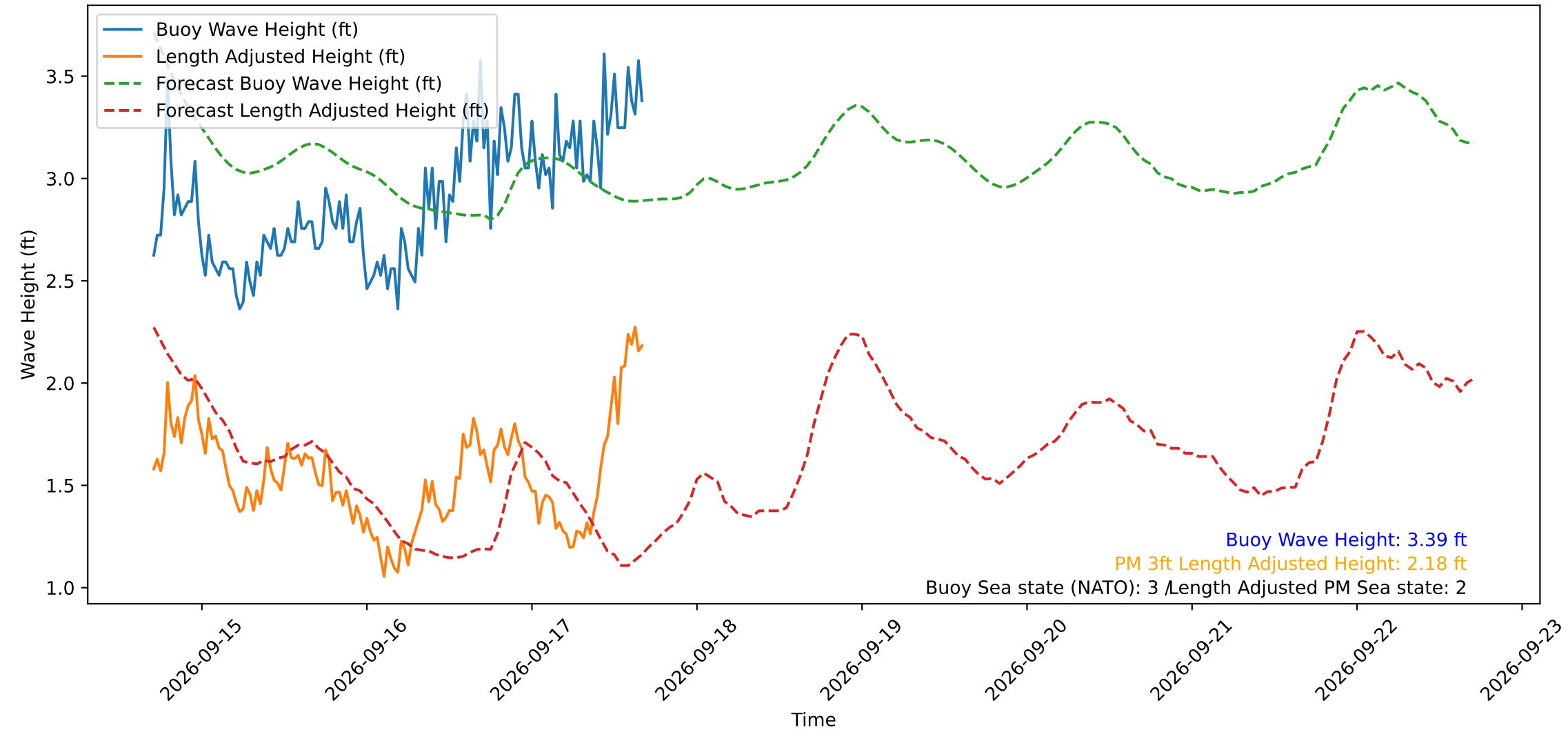
Wave Heights over Time for Oceanside Harbor at 2026-09-17 16:50:29
