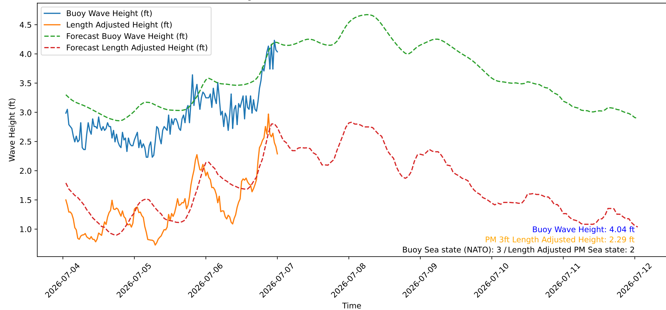
Wave Heights over Time for Red Beach at 2026-07-07 00:40:46
