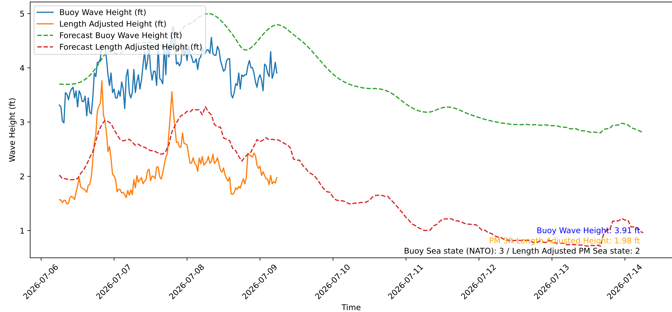
Wave Heights over Time for Green Beach at 2026-07-09 06:11:09
