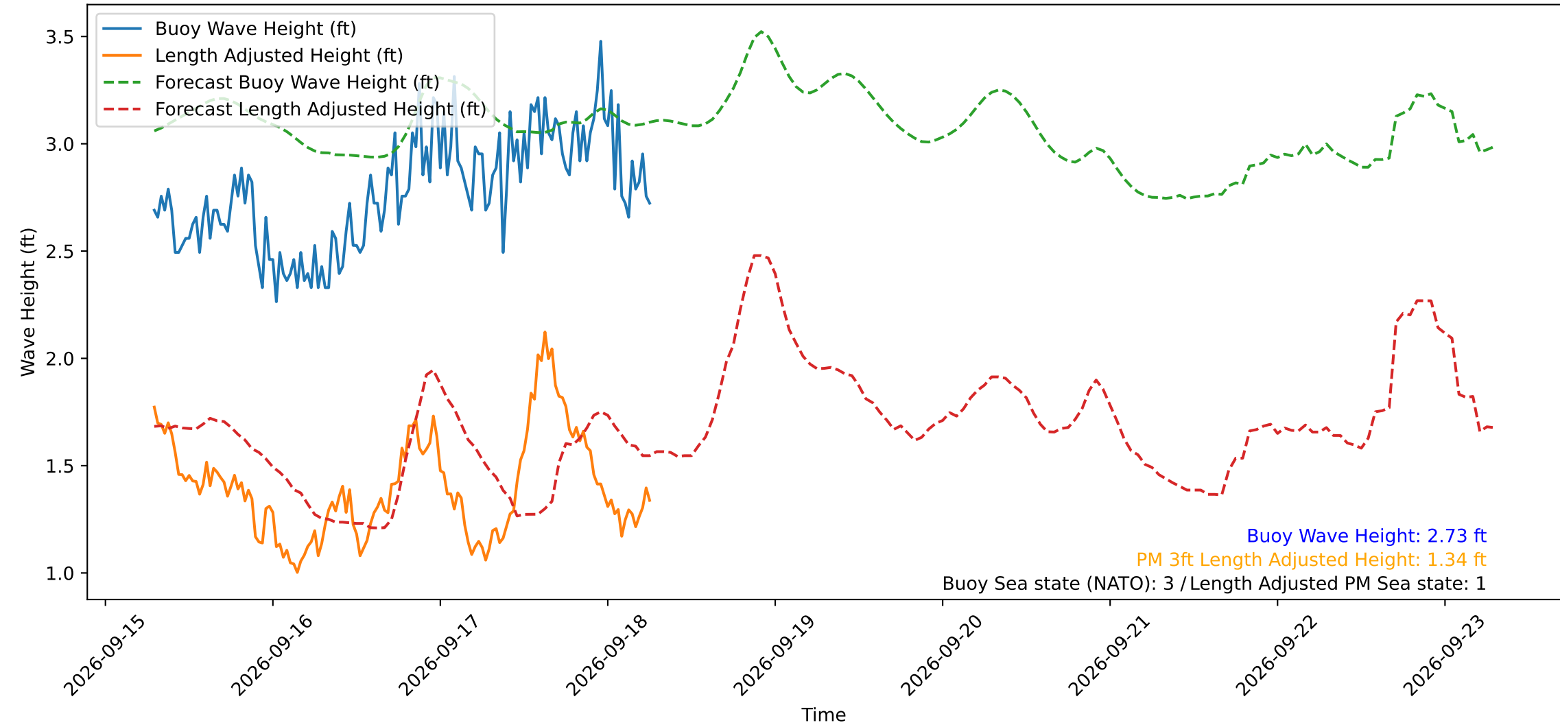
Wave Heights over Time for Green Beach at 2026-09-18 06:51:14
