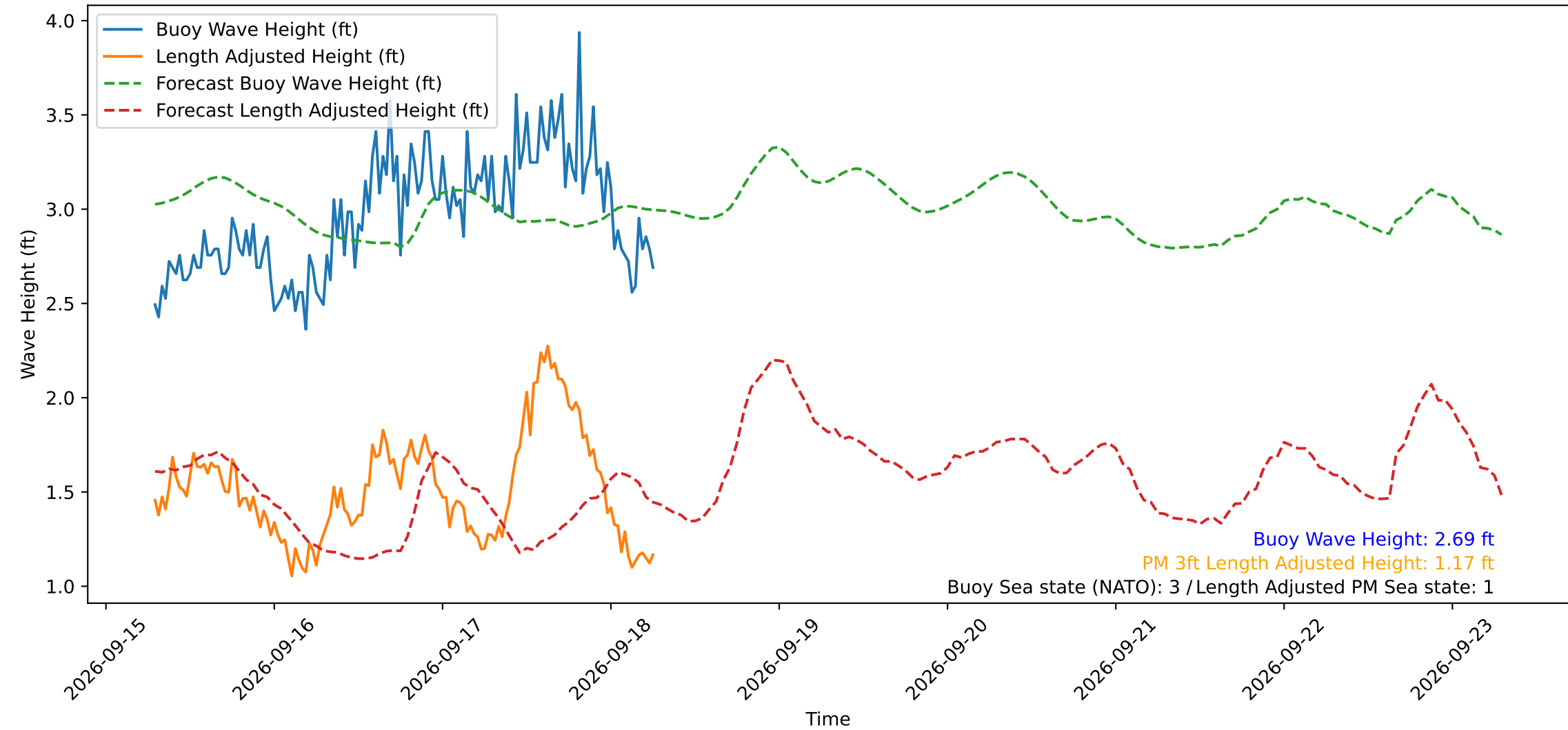
Wave Heights over Time for Oceanside Harbor at 2026-09-18 06:50:30
