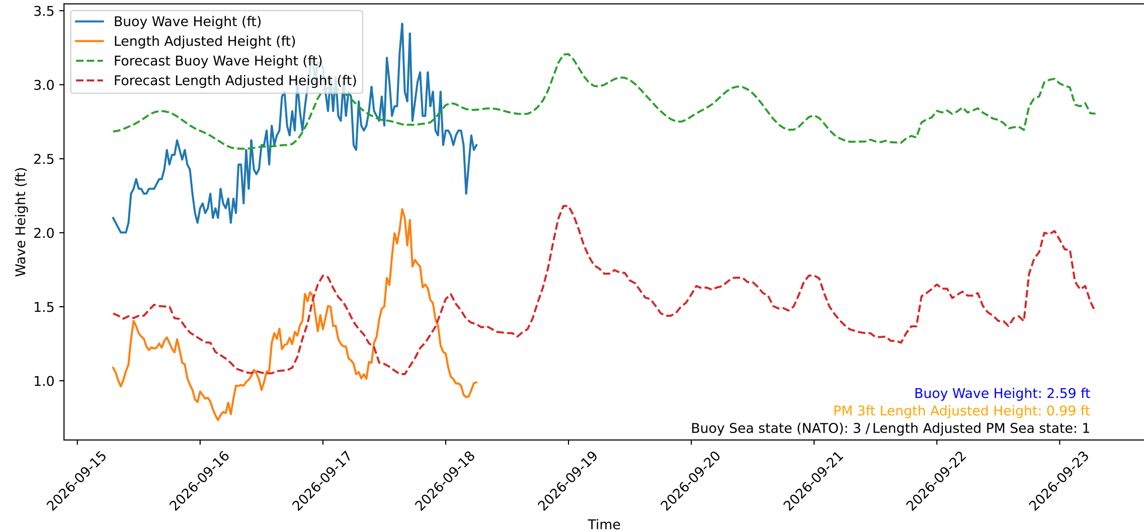
Wave Heights over Time for Red Beach at 2026-09-18 06:50:50
