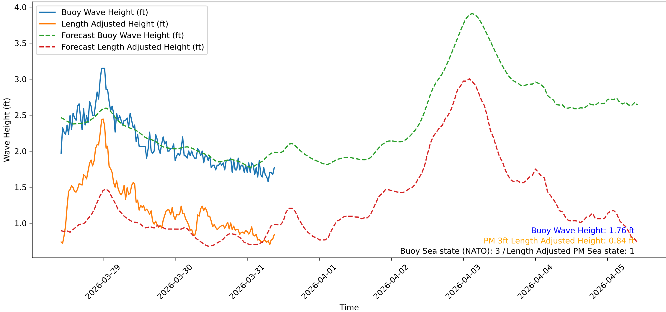
Wave Heights over Time for Oceanside Harbor at 2026-03-31 09:50:32
