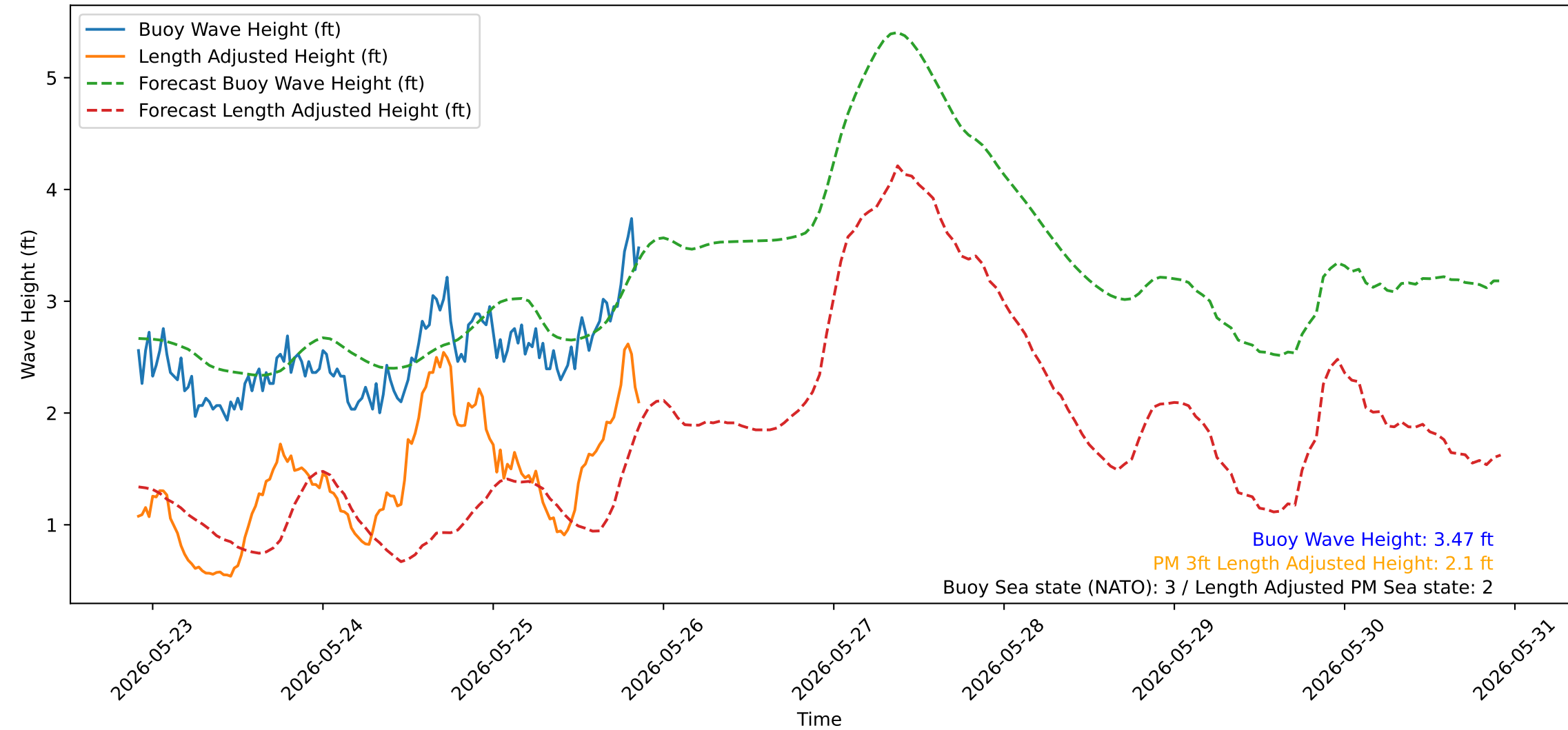
Wave Heights over Time for Red Beach at 2026-05-25 21:50:50
