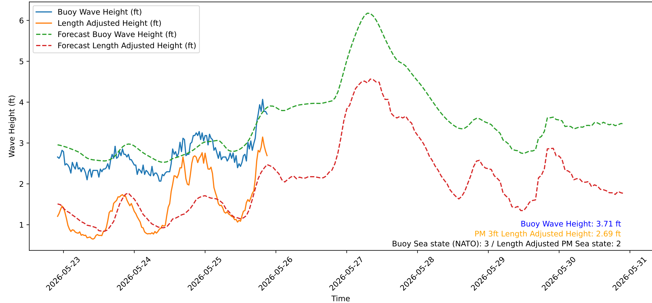
Wave Heights over Time for Green Beach at 2026-05-25 21:51:12
