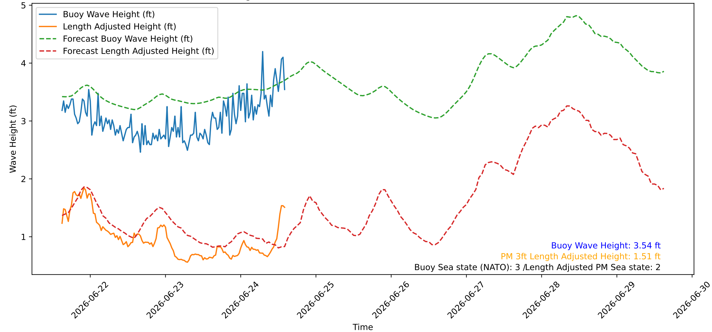
Wave Heights over Time for Green Beach at 2026-06-24 14:51:08
