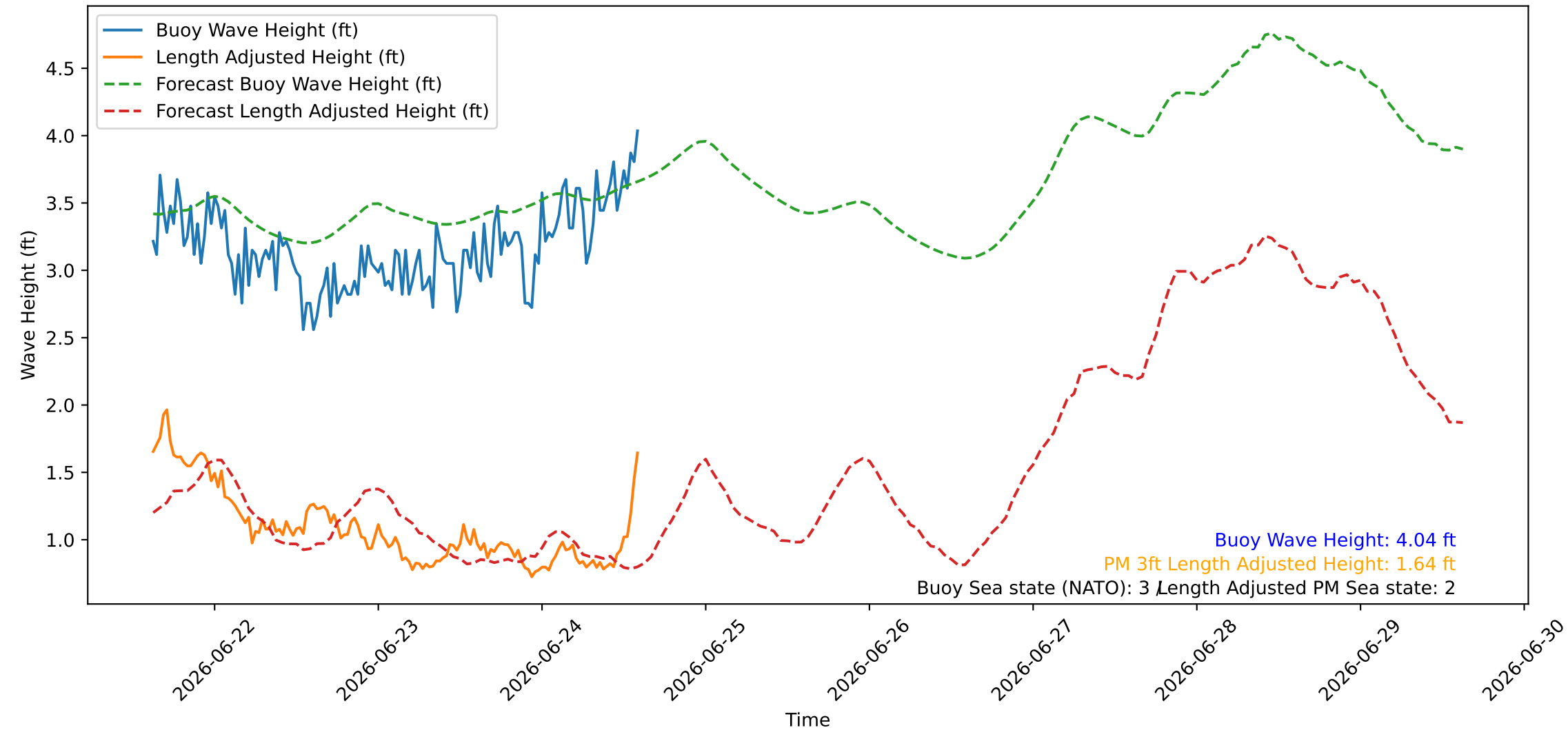
Wave Heights over Time for Oceanside Harbor at 2026-06-24 14:50:25
