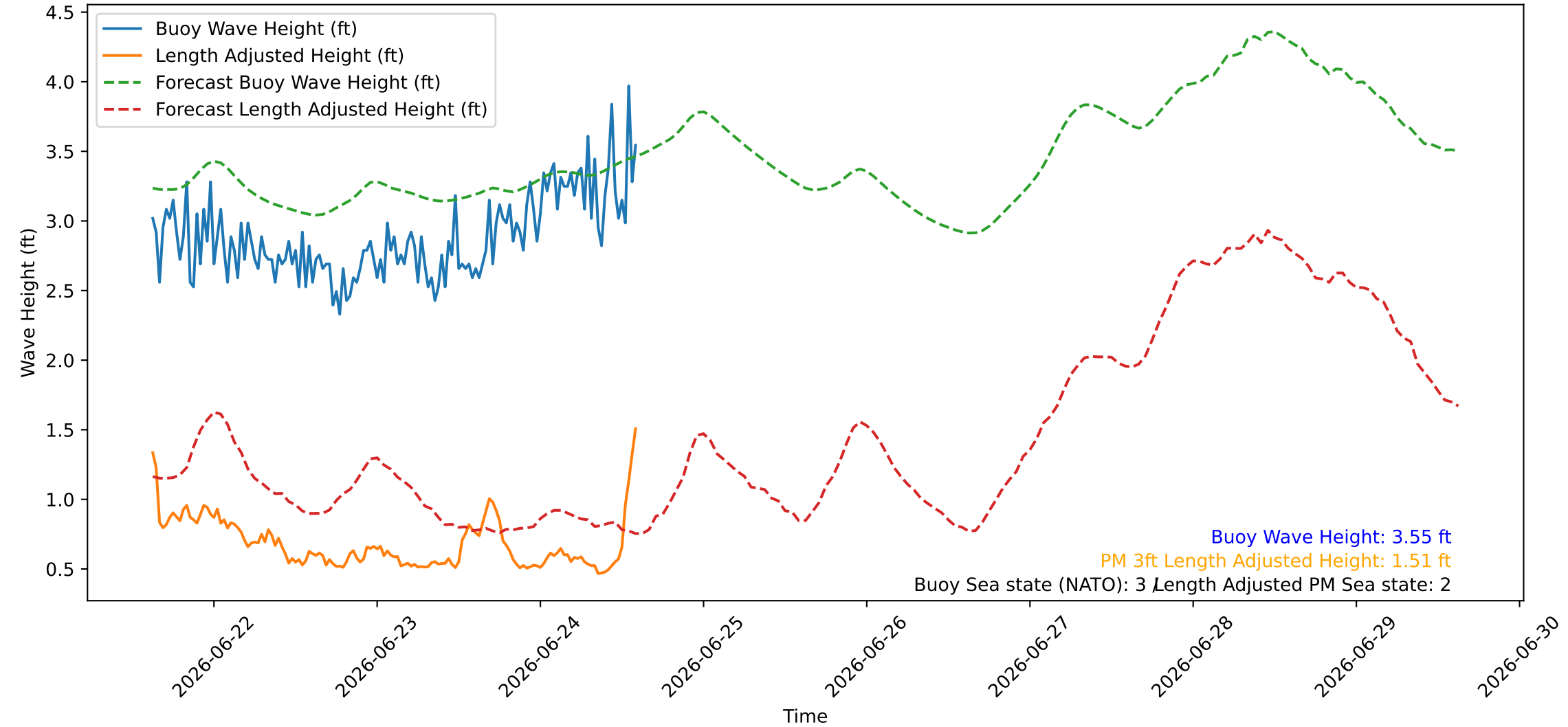
Wave Heights over Time for Red Beach at 2026-06-24 14:50:46
