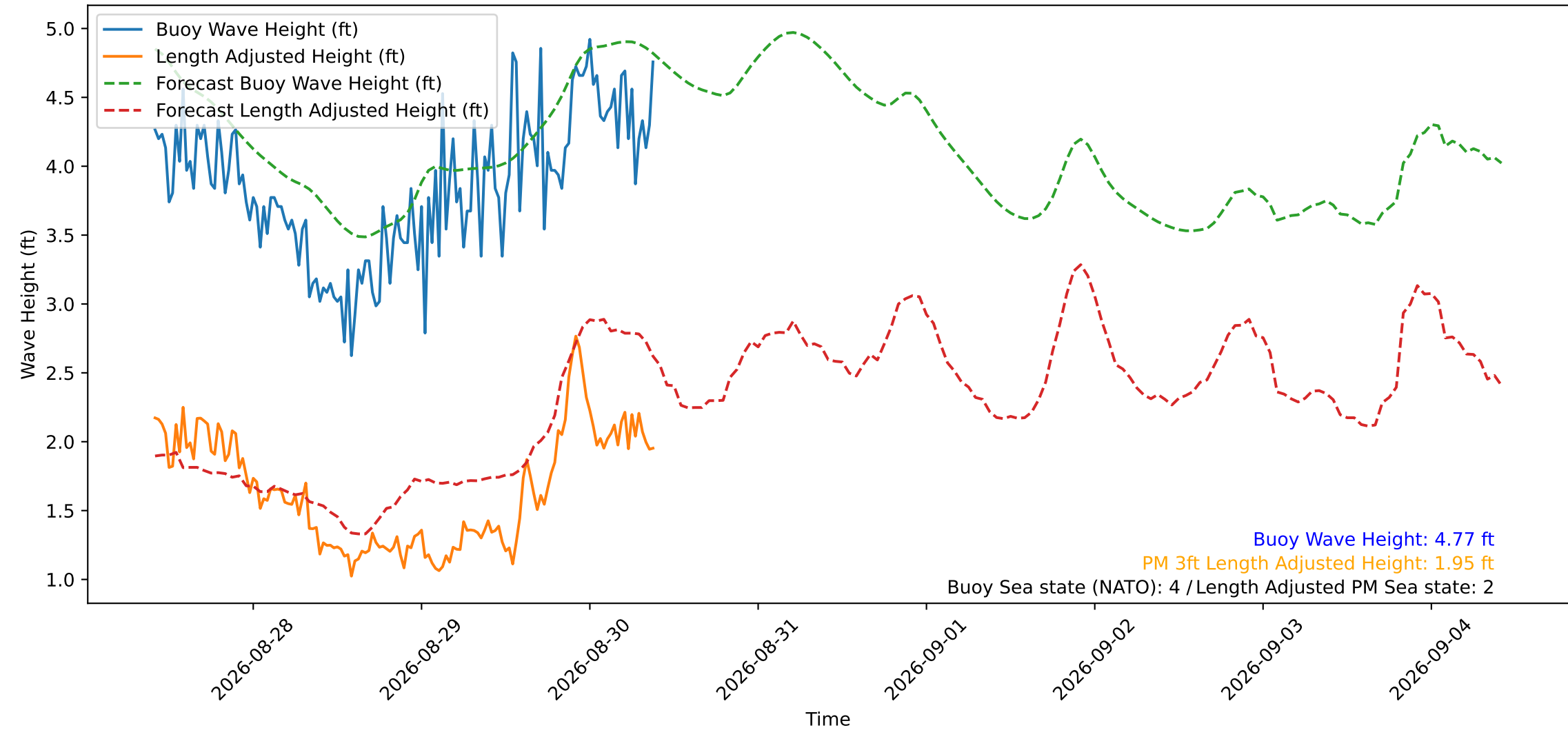
Wave Heights over Time for Green Beach at 2026-08-30 09:41:12
