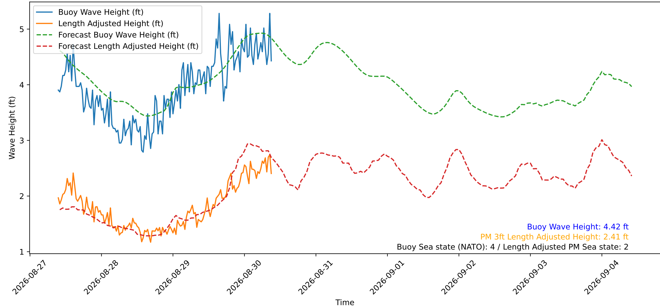
Wave Heights over Time for Oceanside Harbor at 2026-08-30 09:40:29
