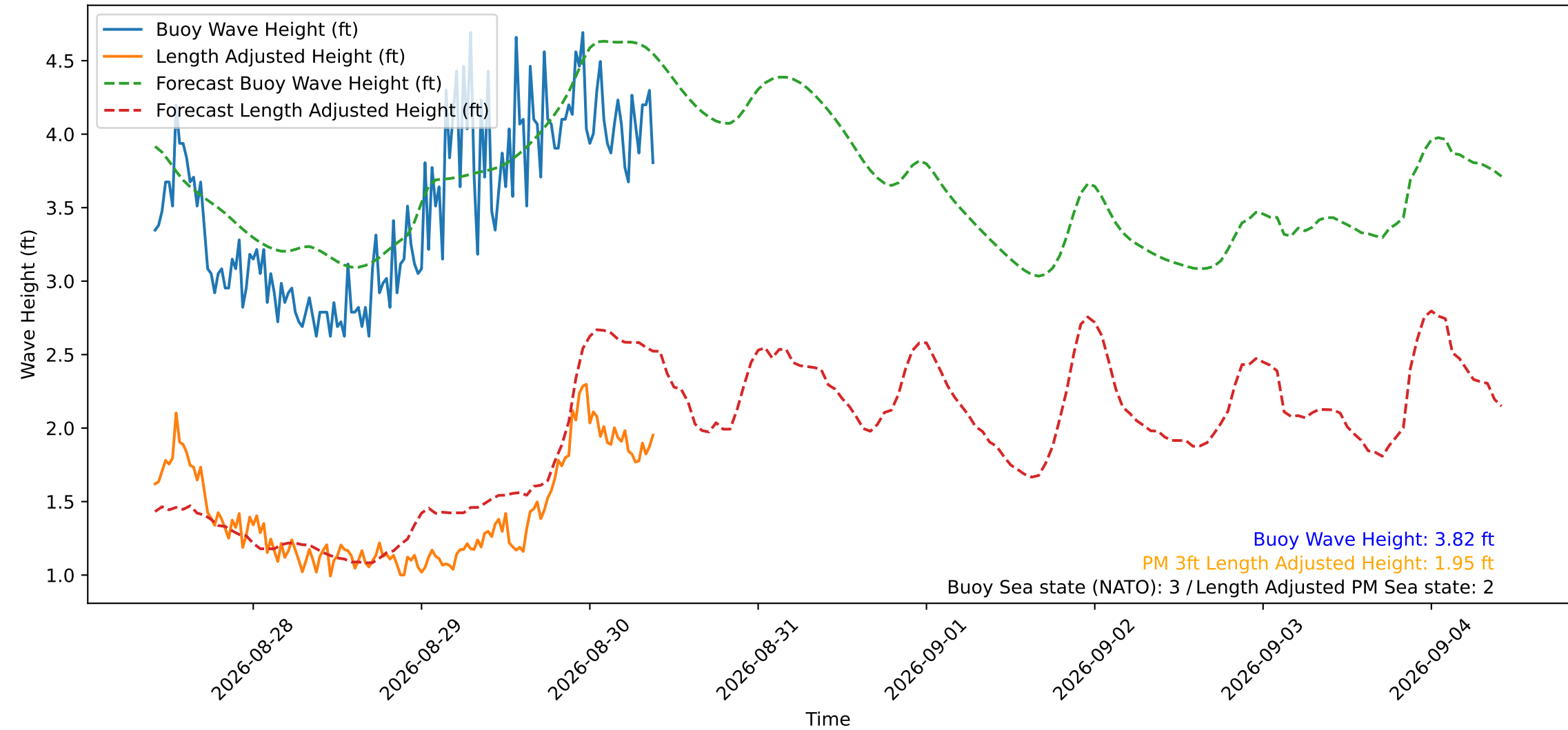
Wave Heights over Time for Red Beach at 2026-08-30 09:40:49
