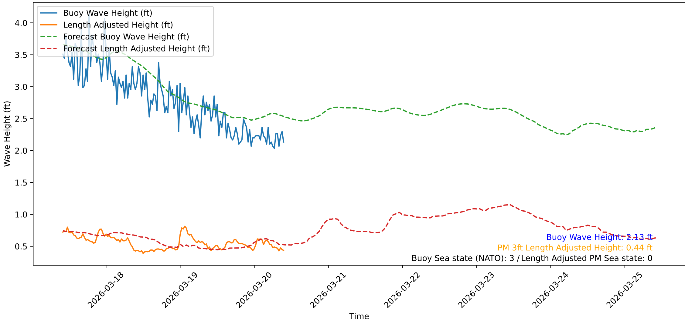
Wave Heights over Time for Green Beach at 2026-03-20 10:11:10
