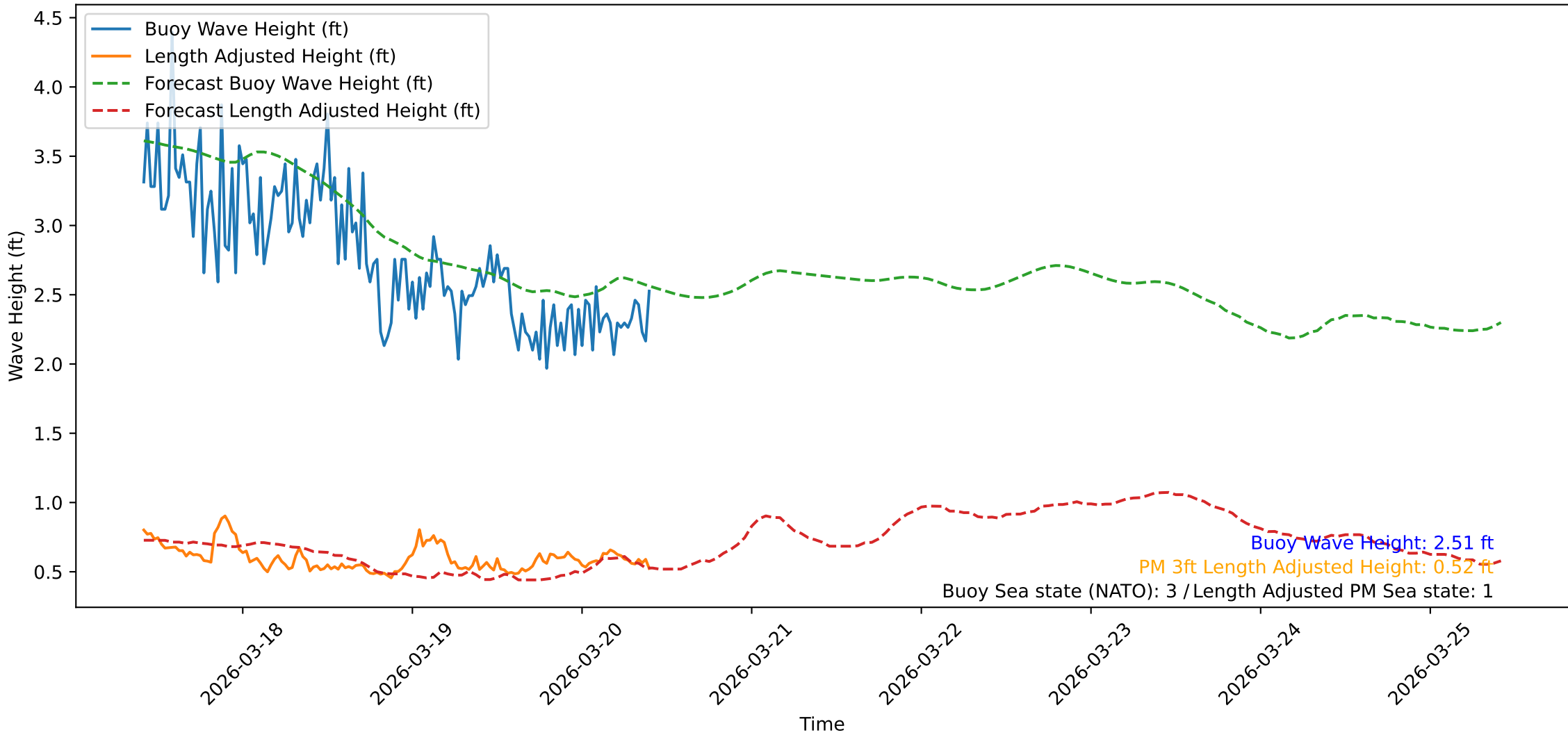
Wave Heights over Time for Oceanside Harbor at 2026-03-20 10:10:31
