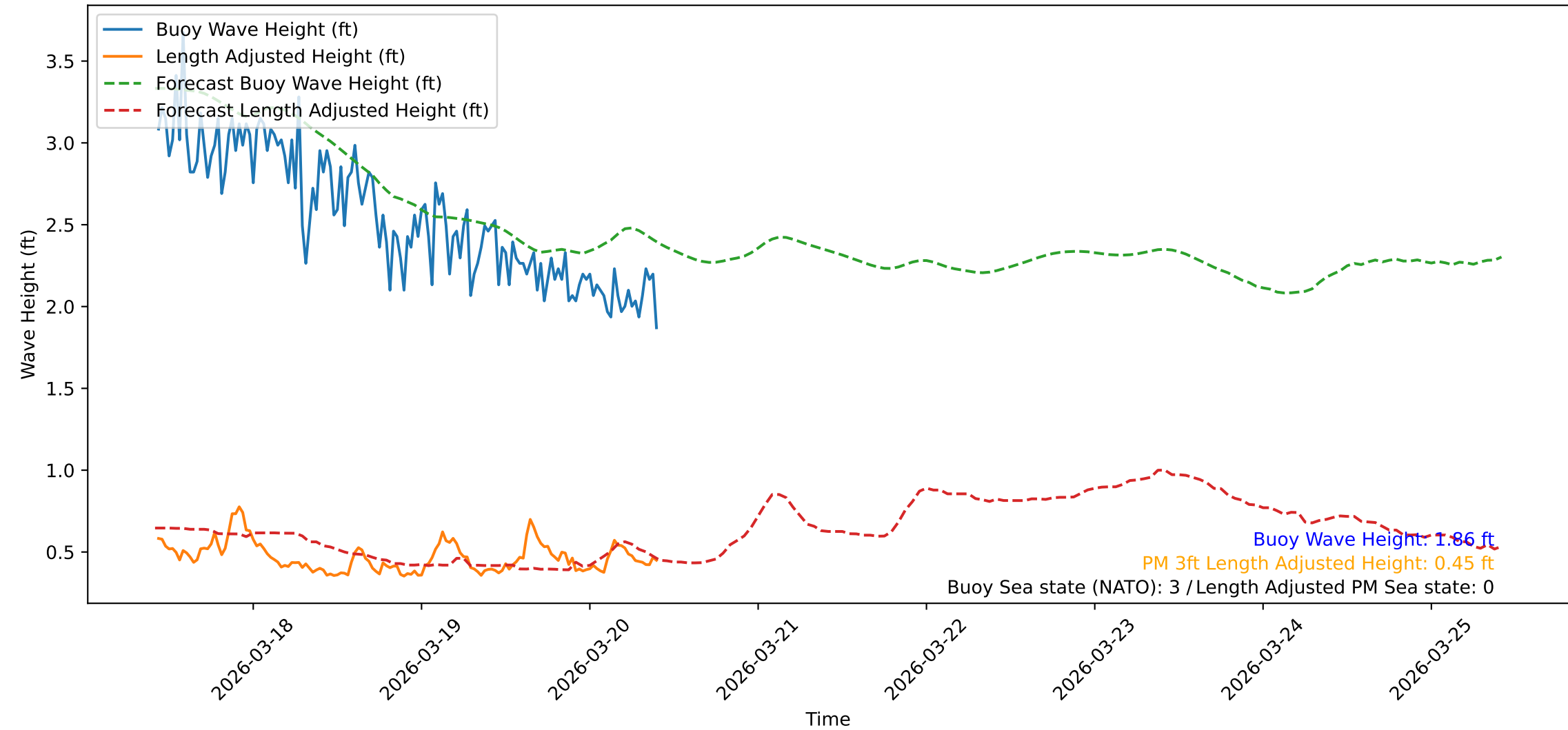
Wave Heights over Time for Red Beach at 2026-03-20 10:10:47
