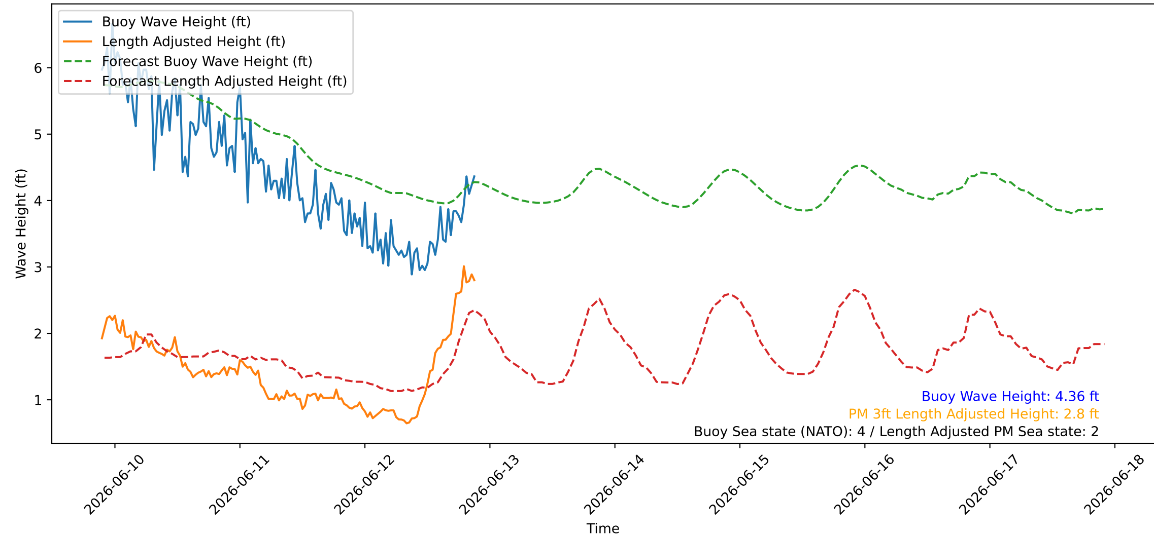
Wave Heights over Time for Green Beach at 2026-06-12 21:41:09
