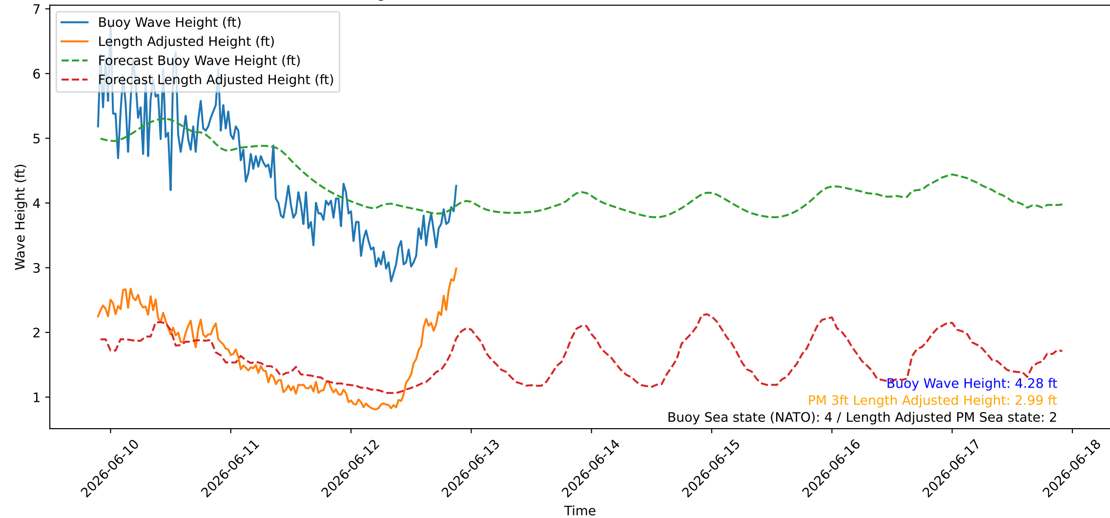
Wave Heights over Time for Oceanside Harbor at 2026-06-12 21:40:27
