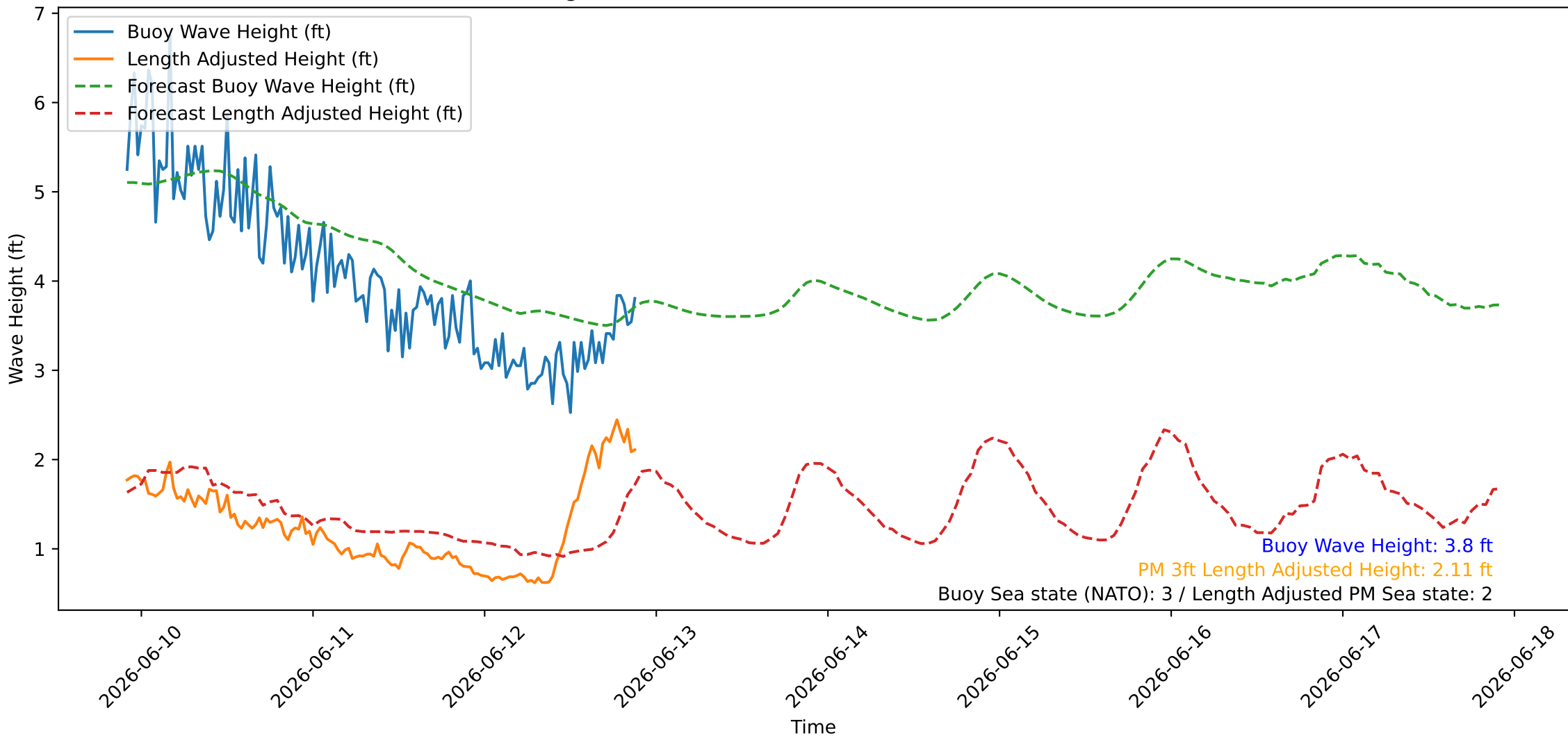
Wave Heights over Time for Red Beach at 2026-06-12 21:40:47
