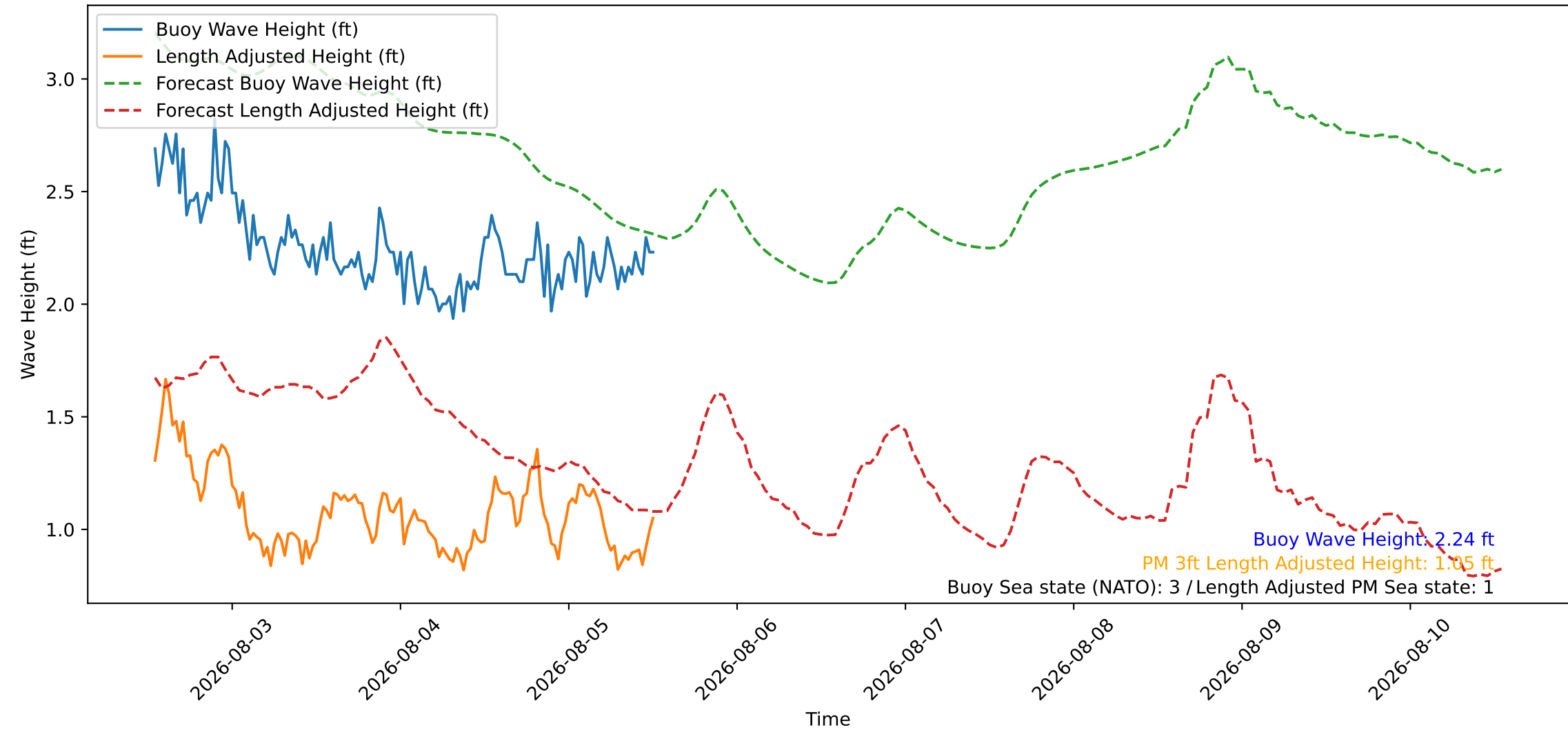
Wave Heights over Time for Green Beach at 2026-08-05 13:01:08
