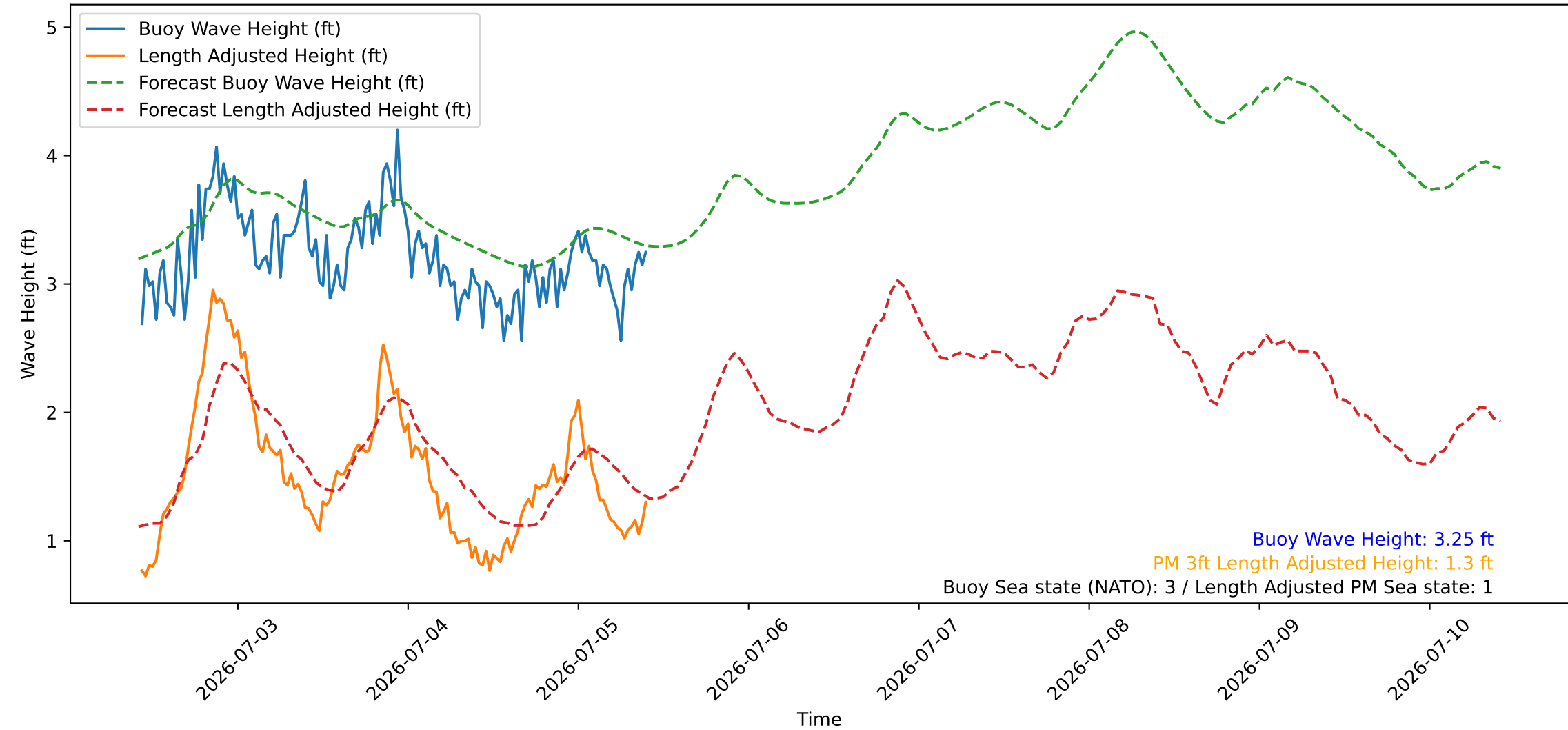
Wave Heights over Time for Green Beach at 2026-07-05 10:21:13
