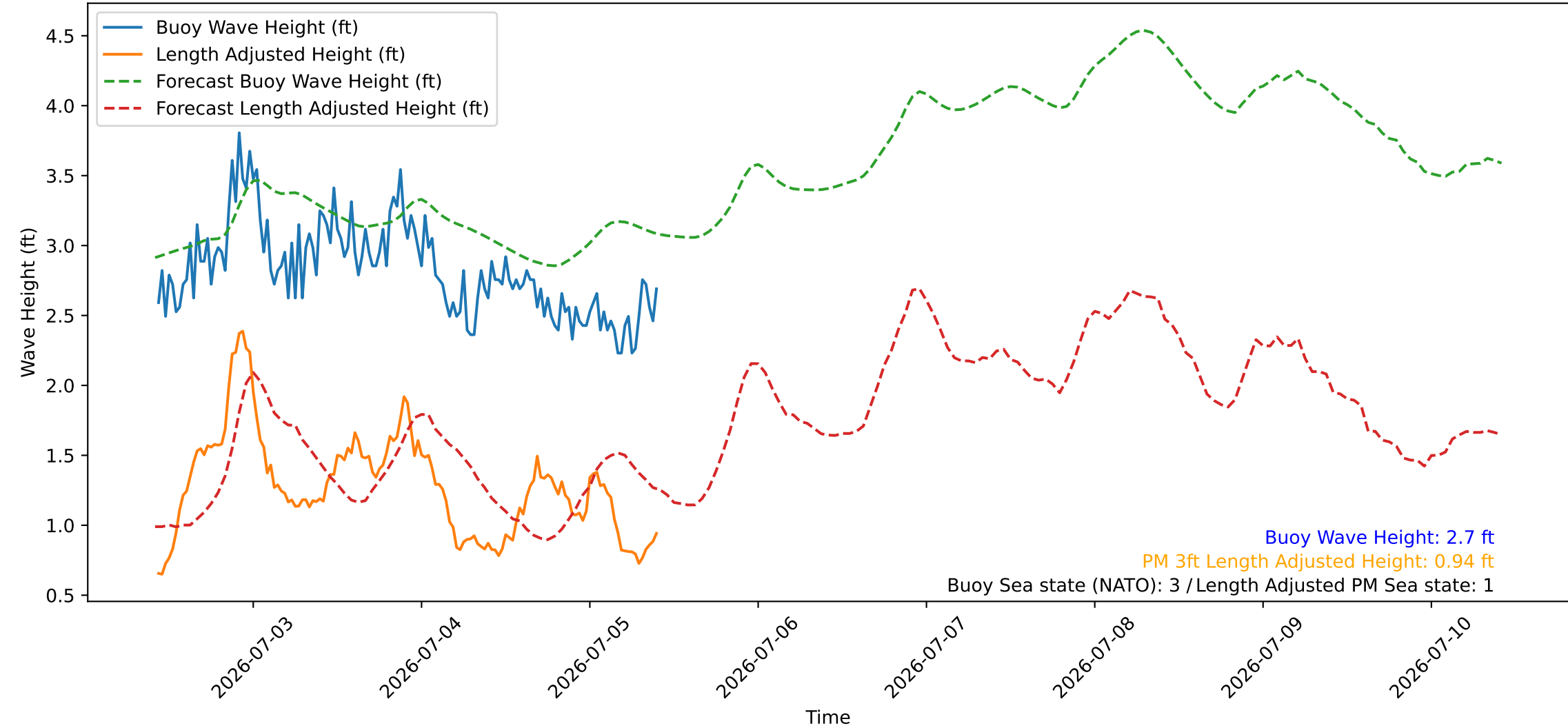
Wave Heights over Time for Red Beach at 2026-07-05 10:20:49
