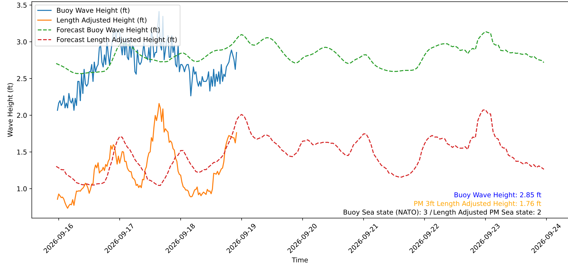
Wave Heights over Time for Red Beach at 2026-09-18 23:00:49
