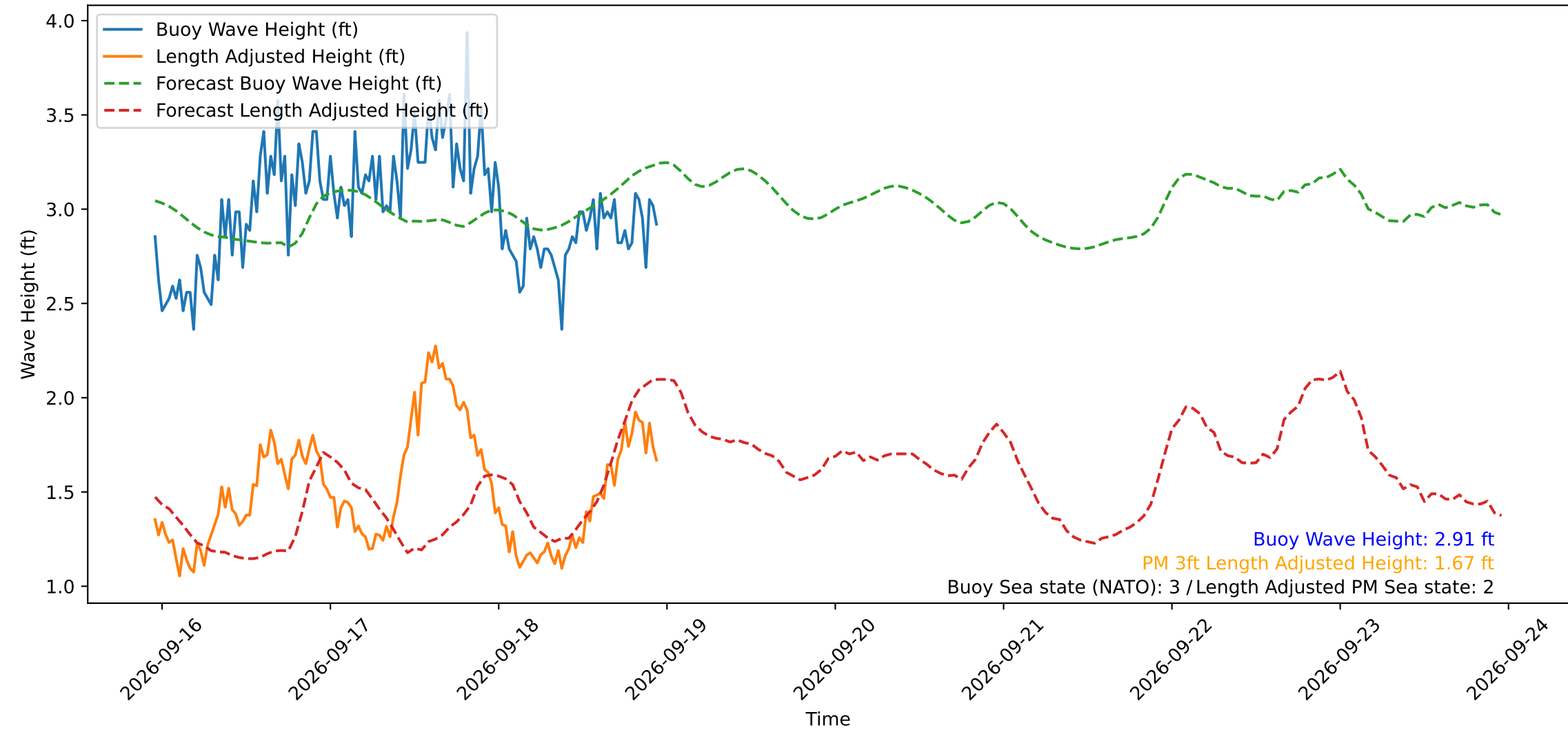
Wave Heights over Time for Oceanside Harbor at 2026-09-18 23:00:29
