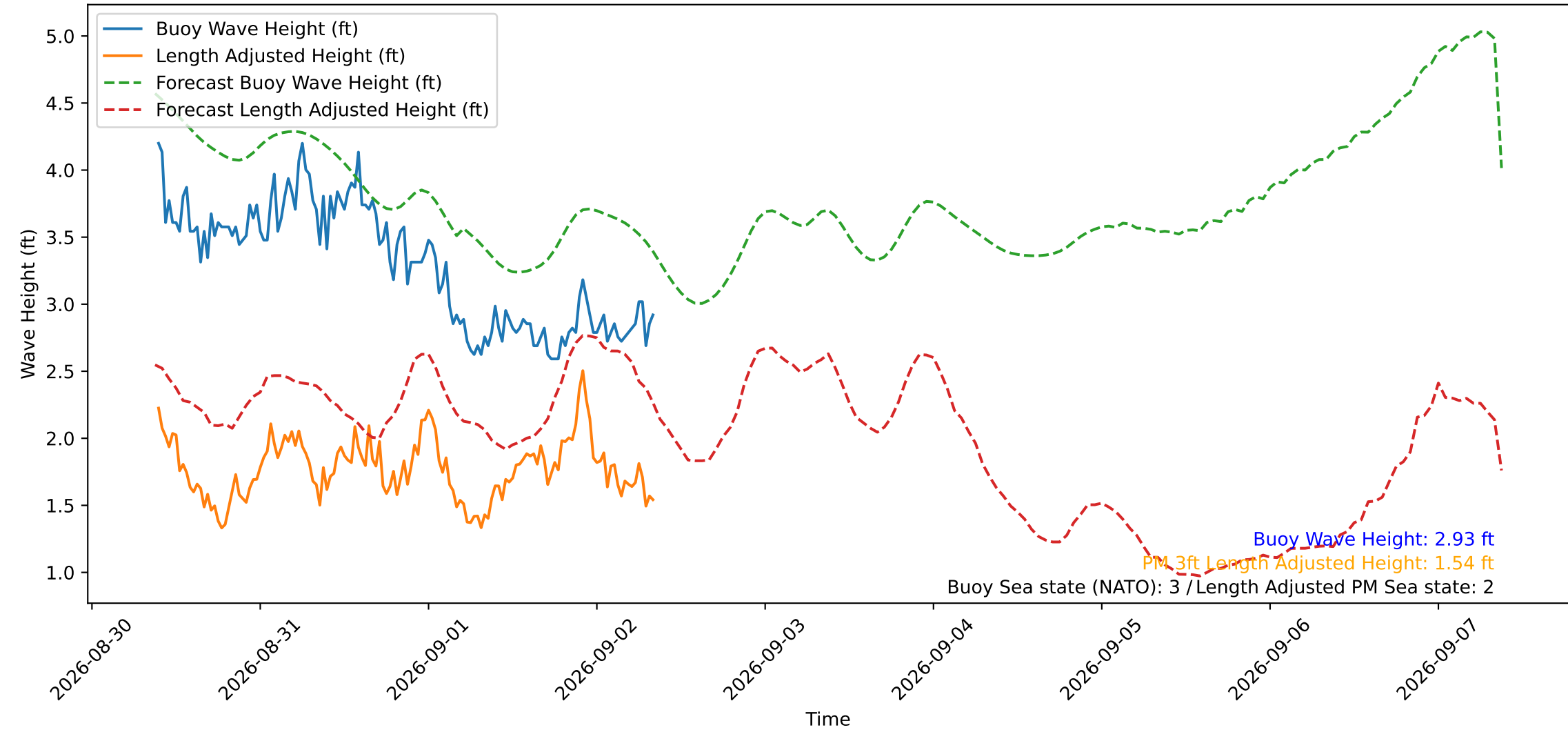
Wave Heights over Time for Red Beach at 2026-09-02 09:00:50
