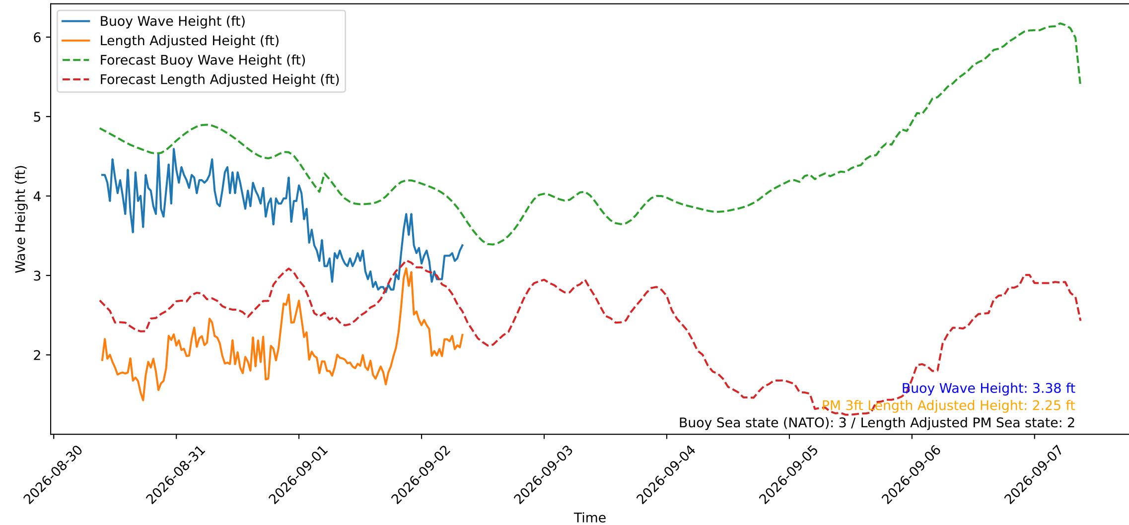
Wave Heights over Time for Green Beach at 2026-09-02 09:01:13
