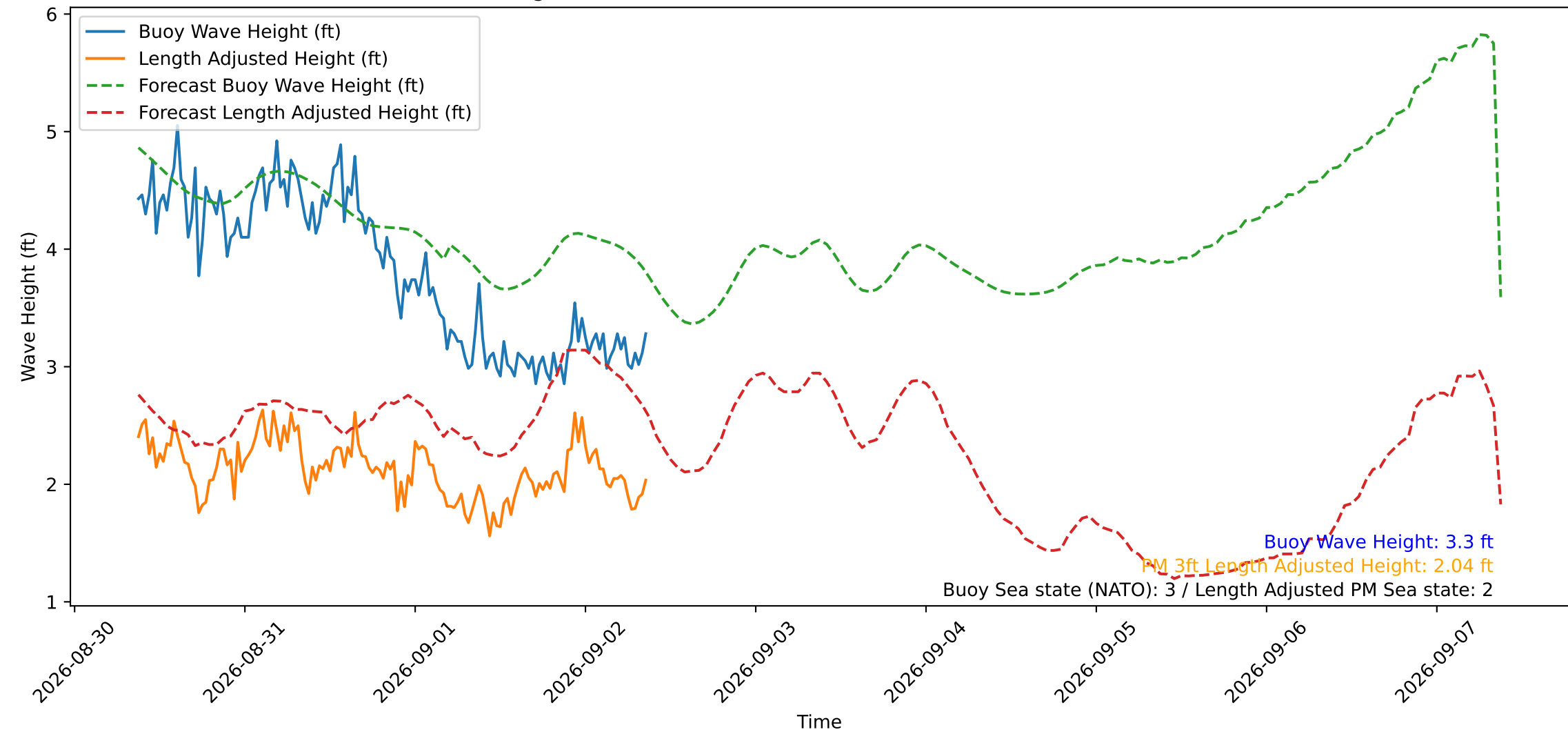
Wave Heights over Time for Oceanside Harbor at 2026-09-02 09:00:30
