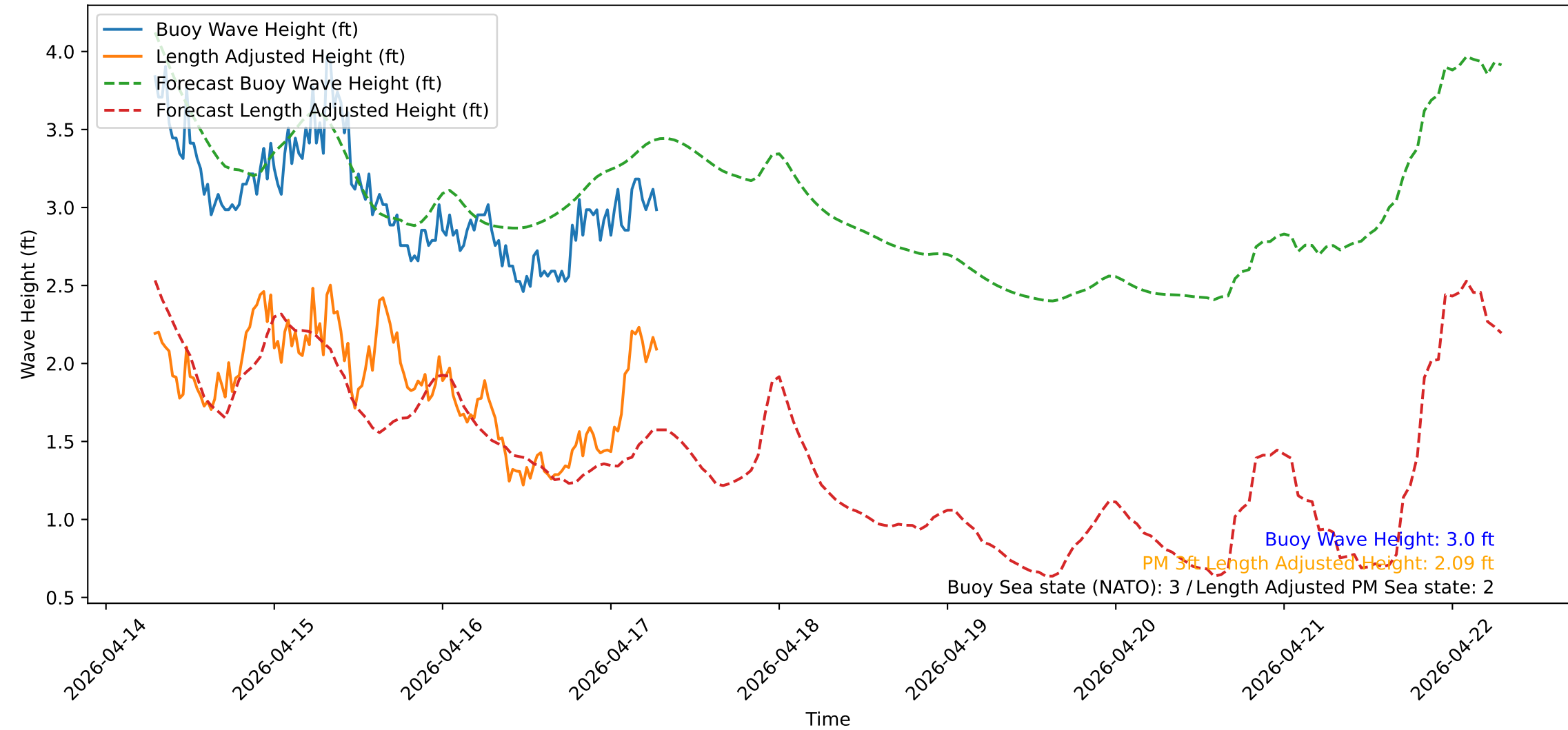
Wave Heights over Time for Green Beach at 2026-04-17 07:11:19
