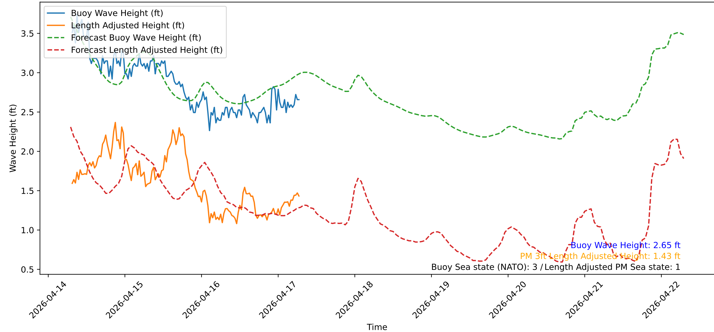
Wave Heights over Time for Red Beach at 2026-04-17 07:10:57
